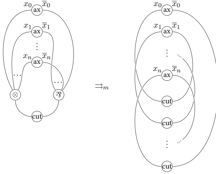
Figure 3.14 – A cyclic counterexample to Corollary 3.4.19
