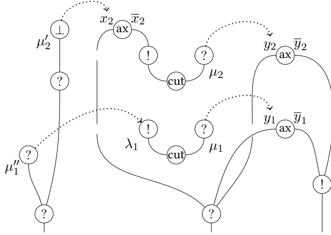
Figure 3.16 – Representation of the resource net p \in \mathbf{T}(P) where P is the net of Figure 3.15, k_b = 2 , k_{b',1} = 0 and k_{b',2} = 1 .
