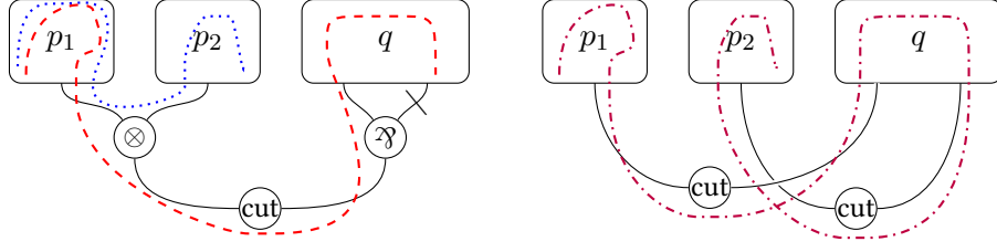
Figure 3.12 – A cut, the resulting slipknot, and examples of paths before and after reduction
