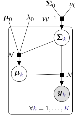
Figure 5.2: Graphical model of the hierarchical structure of the generative model for the vector y_k of peptide intensities in K groups of biological samples, i.e. K experimental conditions.
