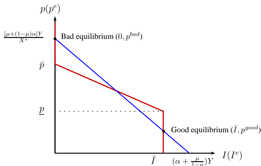
Figure 3.6: Multiple equilibria
