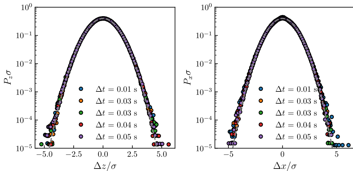
Figure 6.2.4: Normalized probability density functions P_i \sigma of the normalized displacements \Delta x/\sigma and \Delta z/\sigma , at short times, with \sigma^2 the corresponding MSD (see Fig. 6.2.3), for different time increments \Delta t ranging from 0.01 s to 0.05 s, as indicated with different colors. The gray dashed lines are normalized Gaussian distributions, with zero means and unit variances.
