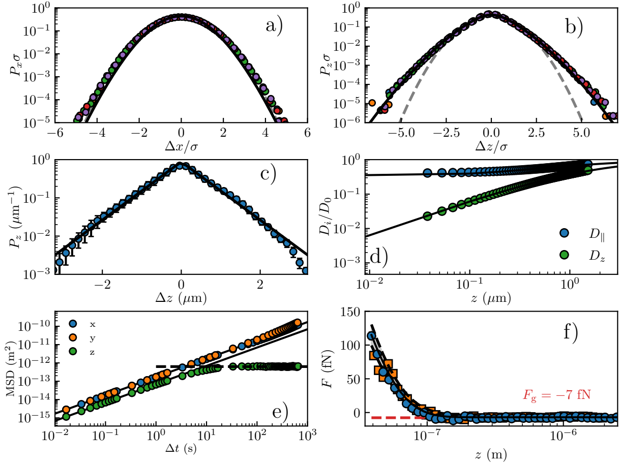
Figure 5.2.9: Summary of our inference method on simulated data with B = 4.8 , \ell_D = 21 nm, and \ell_B = 570 nm. The multi-fitting method of all the observable measures B = 4.2 \pm 0.5 , \ell_D = 21 \pm 1 nm, and \ell_B = 570 \pm 1 nm a,b) Normalized probability density functions P_i \sigma of the normalized displacements \Delta x/\sigma and \Delta z/\sigma , at short times, with \sigma^2 the corresponding MSD (see Fig. 5.2.4), for different time increments \Delta t ranging from 0.0167 s to 0.083 s, as indicated with different colors. The solid lines are the best fits to Eq. (5.2.6), using Eqs. (5.1.28), (5.1.46), and (5.1.47). For comparison, the gray dashed lines are normalized Gaussian distributions, with zero means and unit variances. c) Probability density function P_z of the displacement \Delta z , at long times, averaged over several values of \Delta t ranging between 25 s and 30 s. The solid line is the best fit to Eq. (5.2.8), using Eq. (5.1.28).d) Measured local short-term diffusion coefficients D_i of the microparticle, normalized by the bulk value D_0 , as functions of the distance z to the wall, along both a transverse direction x or y ( D_i = D_{\parallel} = D_x = D_y , blue) and the normal direction z ( D_i = D_z , green) to the wall. The solid lines are the theoretical predictions, D_{\parallel}(z) = D_0 \eta / \eta_{\parallel}(z) and D_z(z) = D_0 \eta / \eta_z(z) , using the local effective viscosities \eta_{\perp}(z) and \eta_{\parallel}(z) of Eqs. (5.1.46) and (5.1.46), respectively.e) Measured mean-squared displacements (MSD, see Eq. (5.2.1)) as functions of the time increment \Delta t , for the three spatial directions, x , y , and z . The solid lines are best fits to Eq. (5.2.2), using Eqs. (5.1.28), (5.1.46) and (5.1.47) providing the average diffusion coefficients \langle D_{\parallel} \rangle = \langle D_x \rangle = \langle D_y \rangle = 0.52 D_0 and \langle D_z \rangle = 0.24 D_0 . The dashed line is the best fit to Eq. (5.2.9), using Eq. (5.1.28), with B = 4.8 , \ell_D = 21 nm, and \ell_B = 530 nm.f) Total normal conservative force F_z exerted on the particle as a function of the distance z to the wall, reconstructed from Eq. (5.2.21), using Eq. (5.1.48) for the circles and Eq. (5.2.20) for the squares. The solid line corresponds to Eq. (5.2.23), with B = 4.8 , \ell_D = 21 nm and \ell_B = 530 nm. The black dashed lines and gray area indicate the amplitude of the thermal noise computed from Eq. (5.2.22). The horizontal red dashed line indicates the buoyant weight F_g = -7 fN of the particle.
