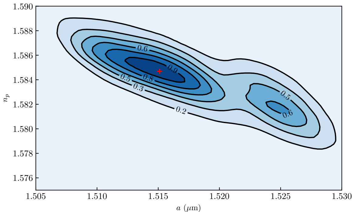
Figure 4.7.1: 2D Probability density function of the measurements of the optical index n_p and radius a . Black lines indicate iso-probability. Taking the 10% top probability, we measure n_p = 1.585 \pm 0.002 and a = 1.514 \pm 0.003 \mu\text{m} . 📍
