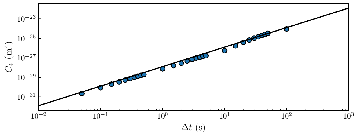
Figure 6.3.1: Fourth cumulant of the transverse displacement as a function of time increment calculated on a simulated 45 minutes long trajectory (see section 5.1.7) with the physical parameters B = 4.8 , \ell_D = 21 nm, \ell_B = 570 nm, and a time-step \tau = 0.05 s. The plain line corresponds to the short time approximation of Eq. (6.3.3).
