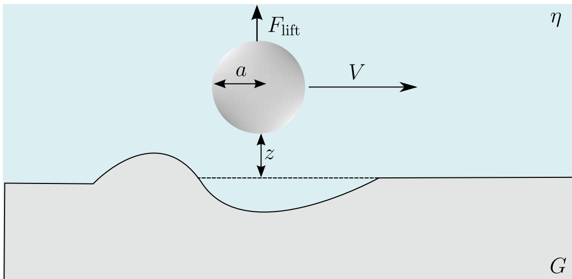
Figure 6.1.1: Schematic of a spherical colloid of radius a immersed in a fluid of viscosity \eta sliding at a velocity V above an incompressible and linear-elastic substrate of shear elastic modulus G . From the elastohydrodynamic interaction between the particle and the soft wall arises a net lift force F_{\text{lift}} (see Eq. (6.1.1)).
