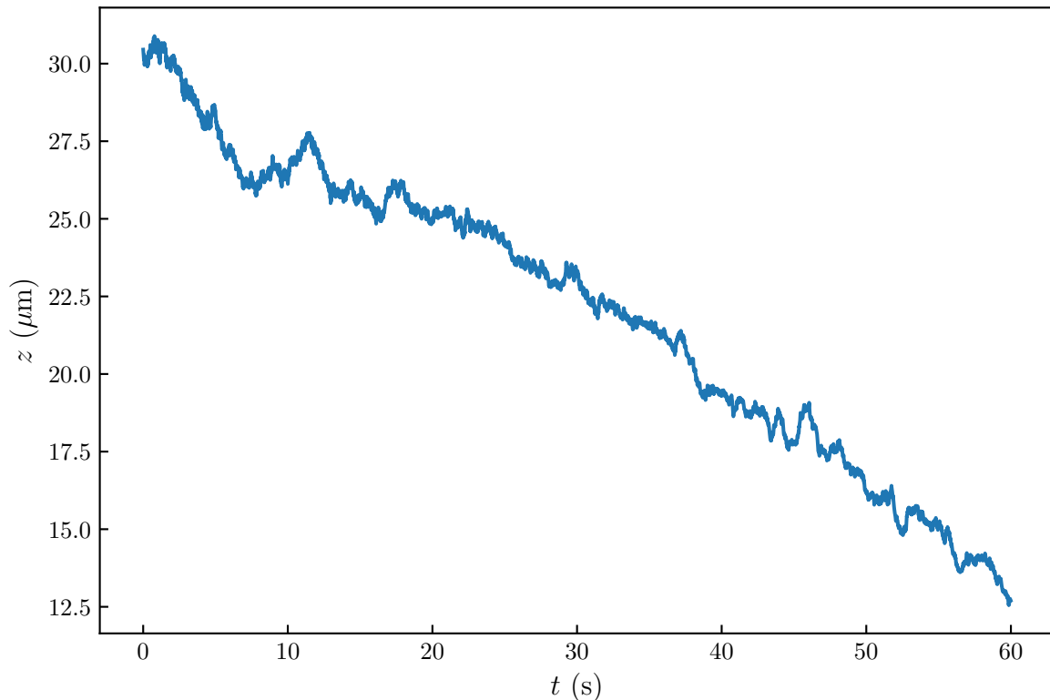
Figure 4.7.3: Experimental trajectory of a polystyrene particle of radius a = 1.5\mu\text{m} sedimenting in water, along the z -axis — i.e. the axis where the gravity acts.
