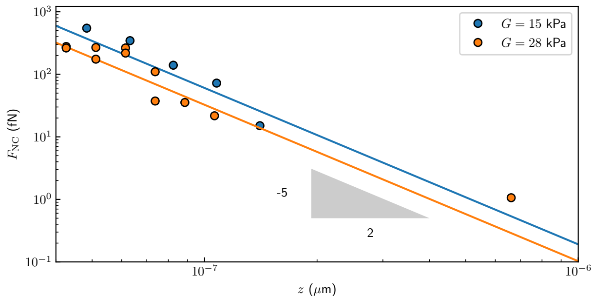
Figure 6.1.3: Non-conservative forces measured experimentally as a function of particle-wall distance, for colloidal particles of radius a = 1.5 \mu\text{m} diffusing in water above an incompressible and linear-elastic substrate of shear elastic moduli G = 15 and 28 \text{ kPa} . Plain lines correspond to the Brownian EHD prediction F_{\text{lift,Brown}} (see Eq. (6.1.2)).
