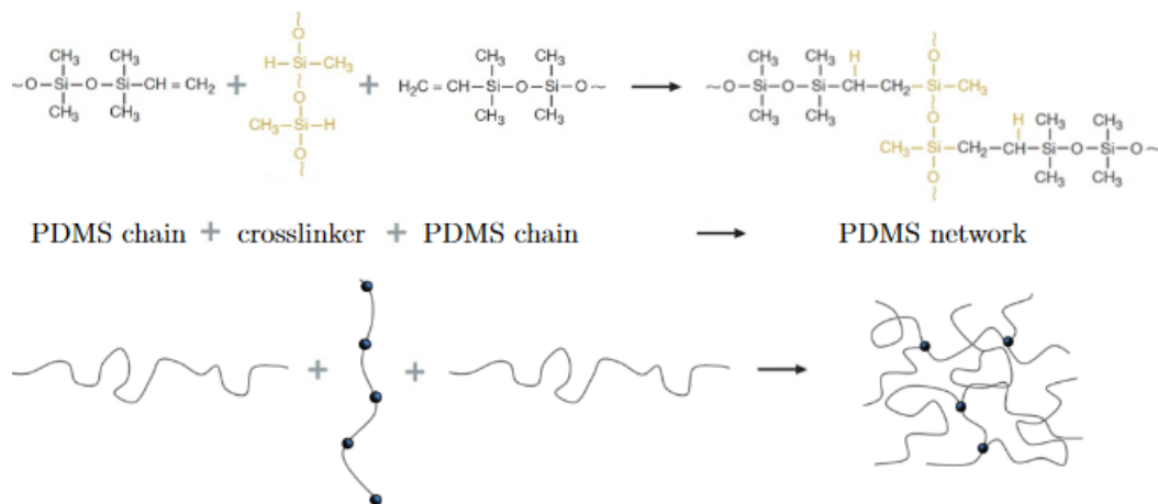
Figure 6.1.2: Figure taken from [118]. Examples of crosslinking reaction between the PDMS chains and a curing agent containing hydrosilane groups.
