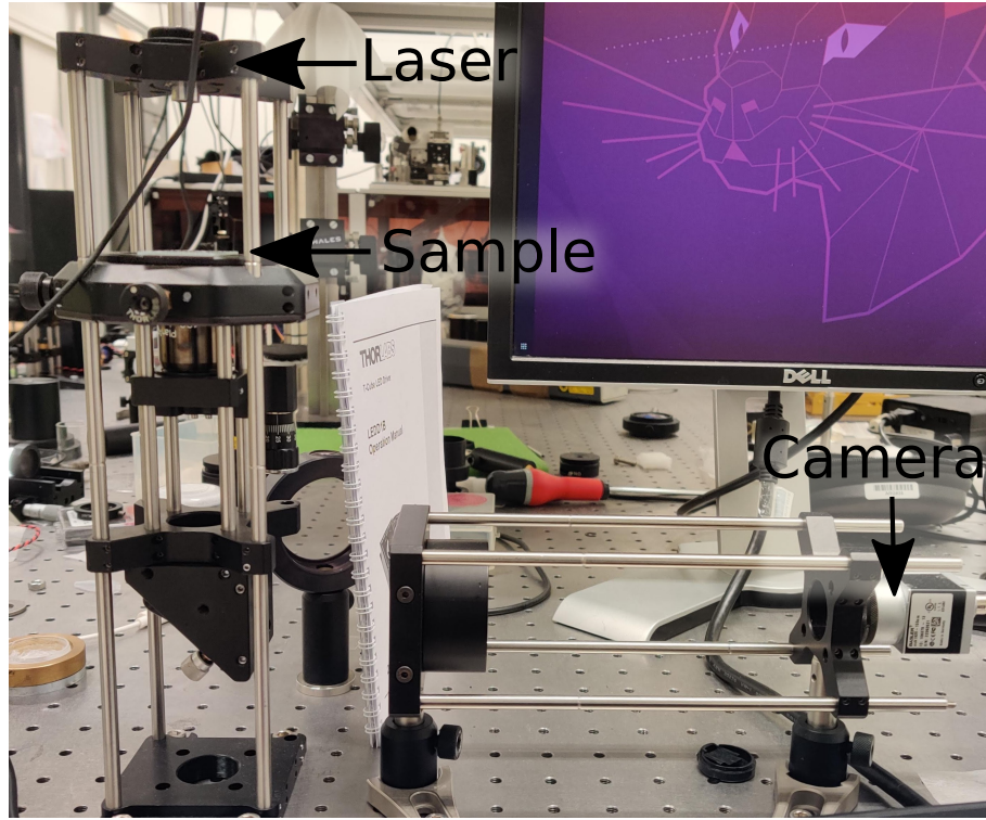
Figure 4.5.1: Photo of the custom-built microscope developed in my thesis. It is composed of a Thorlabs cage system. The camera used is a Basler acA1920-155um. We use a x60 magnification and 1.30 numerical aperture oil-immersion objective lens. The light source is a collimated \lambda = 521 nm wavelength laser.
