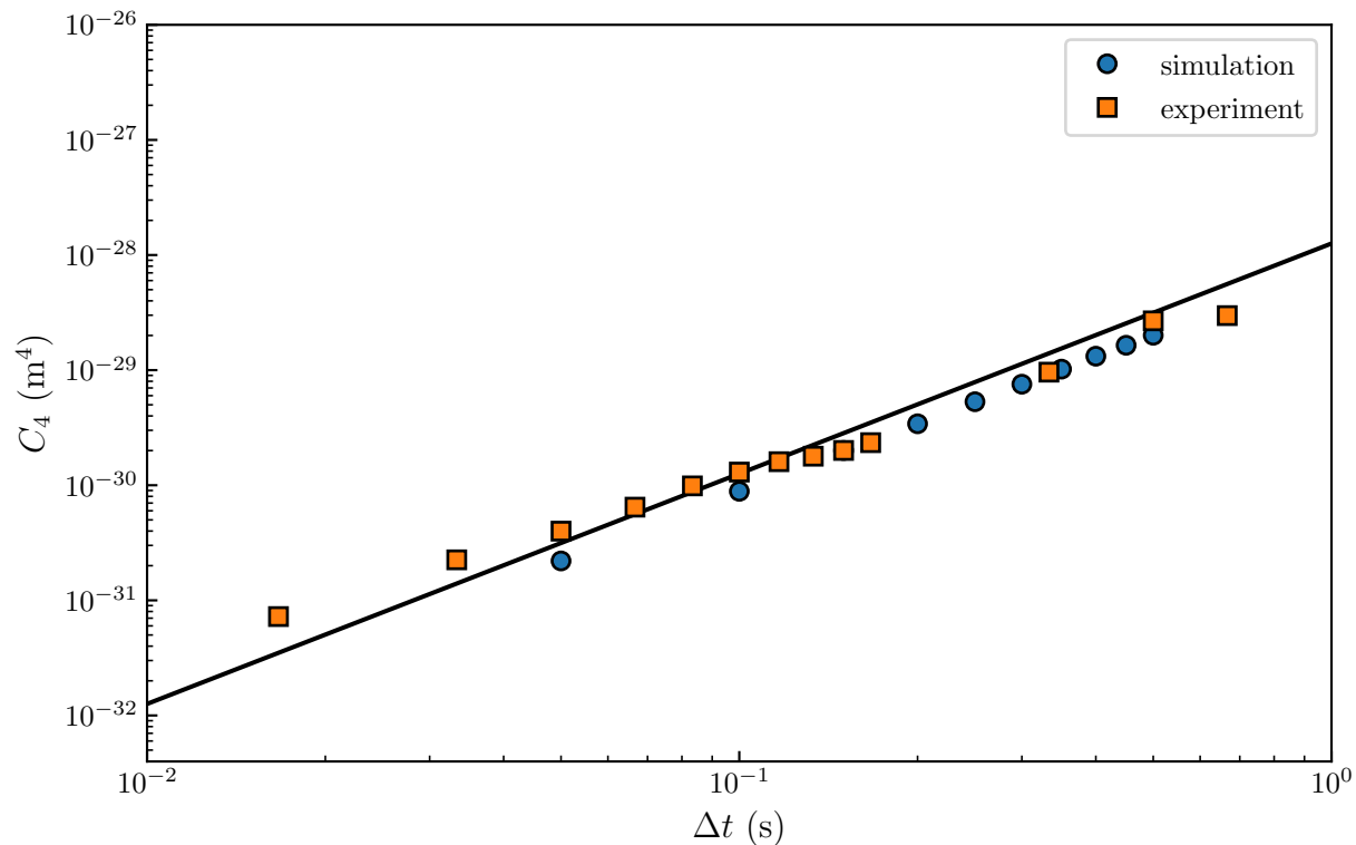
Figure 6.3.2: Experimentally measured 4th cumulant of the transverse displacement as a function of time increment \Delta t . The plain line corresponds Eq. (6.3.3) calculated using Eqs (5.1.47) and (5.1.29) with B = 4.8 , \ell_D = 21 nm, and \ell_B = 530 nm.
