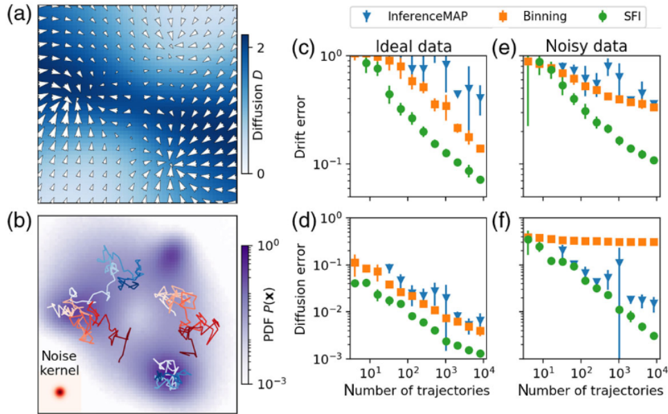
Figure 5.2.6: Figure from [100]. Quantitative comparison of Surface Force Inference (SFI) with other methods on a simulated system mimicking 2D single-molecule trajectories in a complex environment with space-dependent isotropic diffusion. a) The diffusion field (blue gradient) and drift field (white arrows). b) The steady-state distribution function (PDF) of the process. The traces are representative trajectories of 100 time steps. c-f) Comparison of the performance of SFI and two widely used inference methods: InferenceMAP, a method for single-molecule inference (blue triangles) [101], and grid-based binning with maximum-likelihood estimation [98, 102] (orange squares). They evaluated the performance of these methods on the approximation of the drift field (c,e)) and diffusion field (d,f)) as a function of the number N of single-molecule trajectories (similar to the ones in panel b)) used. With ideal data (c,d)) and in the presence of measurement noise(e,f)). The performance is evaluated as the average mean-squared error on the reconstructed field along trajectories. More information about the parameters of their simulation and analysis can be found in their work [100].
