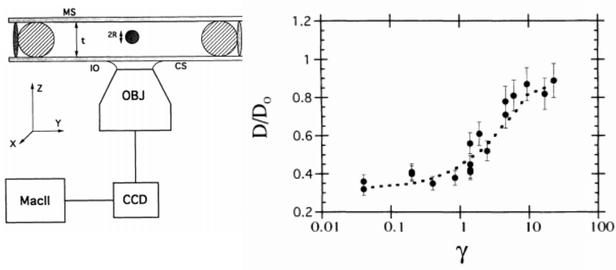
Figure 5.1.5: Figure extracted from [13]. On the left is the experimental setup. It is an inverted microscope used in order to track micrometric particles of diameter 2R inside a liquid cell of thickness t . On the right is the final result, where the authors measure the diffusion parallel ( i.e. along x or y ) coefficient D_{\parallel} (see Eqs. (5.1.47) and (5.1.45)), normalized by the bulk diffusion coefficient D_0 , as a function the confinement parameter \gamma = \langle z \rangle_t / a , with \langle z \rangle_t time-averaged particle-wall distance.
