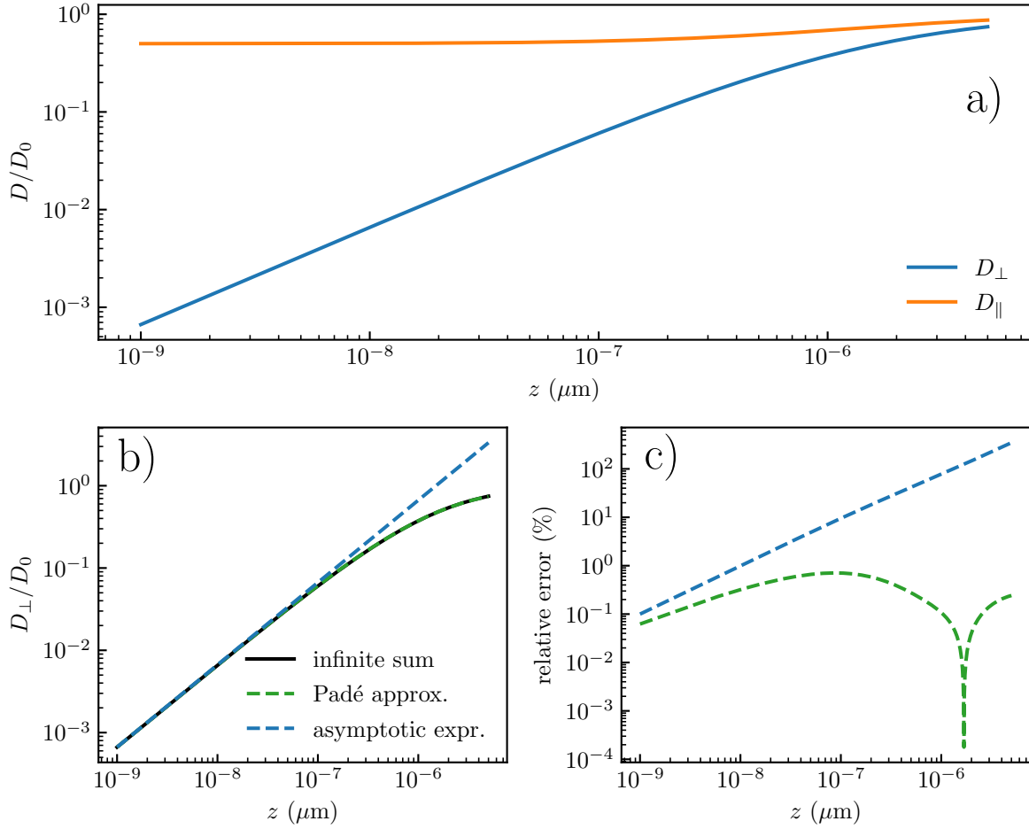
Figure 5.1.7: a) Parallel and perpendicular normalized diffusion coefficients for a colloidal particle of radius a = 1.5 \mu\text{m} . b) Perpendicular normalized diffusion coefficient at a distance z from a wall. The solid black line is the exact solution given by the infinite sum of Eq. (5.1.46). The green dashed line is the Padé approximation of Eq. (5.1.48). The blue dashed line is the near-wall asymptotic expression of Eq. (5.1.49). c) Relative errors between the two approximations (dashed lines of panel b), same color code) and the exact result (solid line of panel b)).
