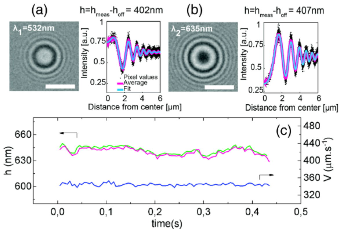
Figure 4.2.1: Figure from [45] representing RICM with two wavelengths. (a) Left: interference patterns created with a wavelength \lambda_1 = 532 \text{ nm} (scale bar 5 \mu\text{m} ). Right: radial intensity profile (black dots) extracted from the image, azimuthally averaged (magenta line) and fitted with Eq. (4.2.8) to measure the height of the particle (here noted h ). (b) Same as (a) with a wavelength \lambda_2 = 635 \text{ nm} . (c) Time series of the height h of a particle (green: \lambda_1 , purple: \lambda_2 ) and the particle velocity measured along the flow (in blue).
