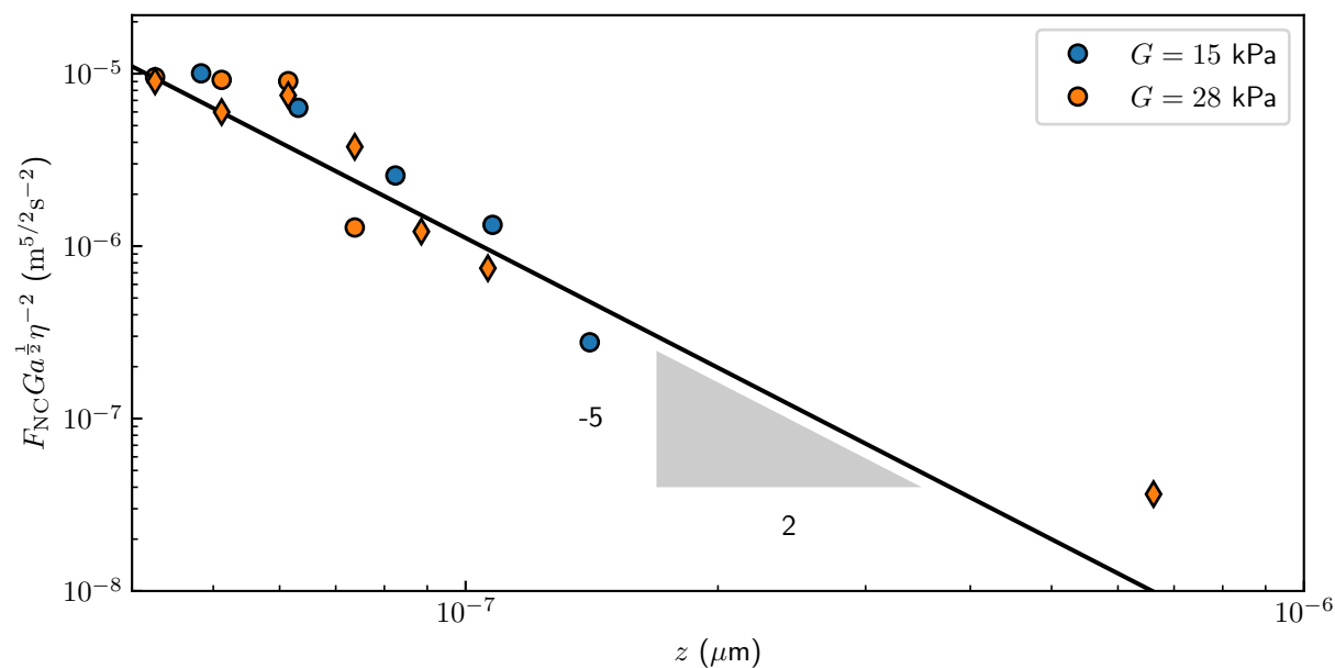
Figure 6.1.4: Non-conservative forces normalized by G a^{1/2} z \eta^{-2} by measured experimentally for colloidal particles of radius a = 1.5 \mu\text{m} diffusing in water above an incompressible and linear-elastic substrate of shear elastic moduli G = 15 and 28 \text{ kPa} . The plain line corresponds to the Brownian EHD lift force F_{\text{lift,Brown}} (see Eq. (6.1.2)).
