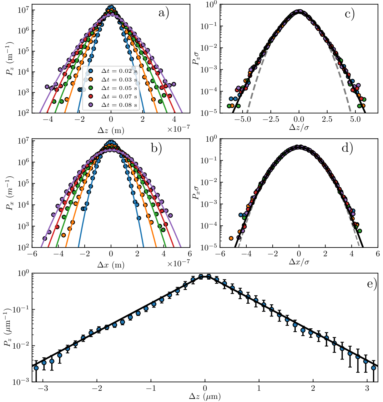
Figure 5.2.5: a, b) Probability density functions P_i of the displacements \Delta x and \Delta z , at short times. The solid lines are the best fits to Eq. (5.2.6), using Eqs. (5.1.29), (5.1.46), and (5.1.47), with B = 4.8 , \ell_D = 21 nm, and \ell_B = 530 nm. c,d) Normalized probability density functions P_i \sigma of the normalized displacements \Delta x/\sigma and \Delta z/\sigma , at short times, with \sigma^2 the corresponding MSD (see Fig. 5.2.4), for different time increments \Delta t ranging from 0.0167 s to 0.083 s, as indicated with different colors. The solid lines are the best fits to Eq. (5.2.6), using Eqs. (5.1.28), (5.1.46), and (5.1.47), with B = 4.8 , \ell_D = 21 nm, and \ell_B = 530 nm. For comparison, the gray dashed lines are normalized Gaussian distributions, with zero means and unit variances. e) Probability density function P_z of the displacement \Delta z , at long times, averaged over several values of \Delta t ranging between 25 s and 30 s. The solid line is the best fit to Eq. (5.2.8), using Eq. (5.1.28), with B = 4.8 , \ell_D = 21 nm, and \ell_B = 530 nm.
