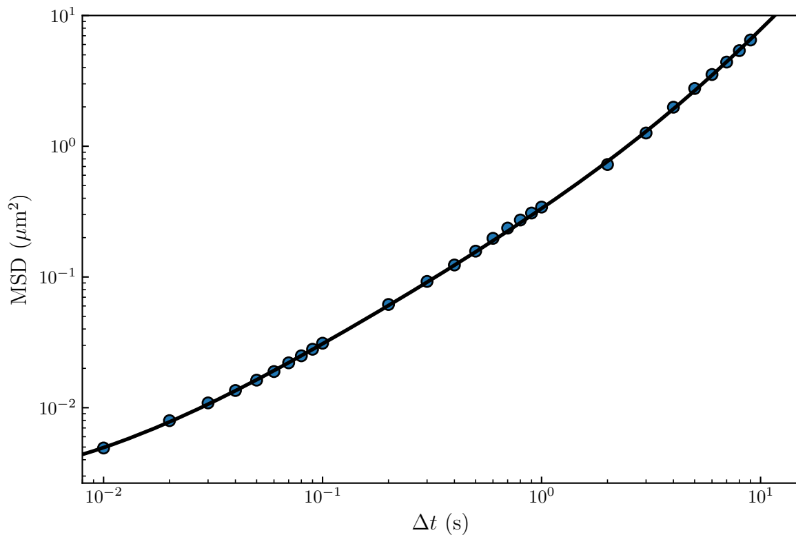
Figure 4.7.4: Measured mean-squared displacement as a function of the time increment \Delta t , along the z -axis. The solid line is the best fit to Eq. (4.7.2), with D_0 = 144 \pm 1 \mu\text{m}^2 \cdot \text{ms}^{-1} , v_{\text{sed}} = 222 \pm 1 \text{ nm} \cdot \text{s}^{-1} and \xi = 25 \text{ nm} .
