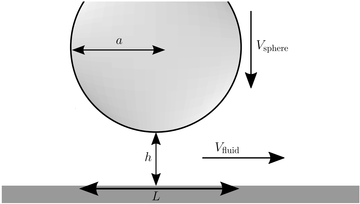
Figure 5.1.6: Schematic representation of a spherical object of radius a moving towards a wall at velocity V_{\text{sphere}} and inducing a fluid velocity V_{\text{fluid}}
