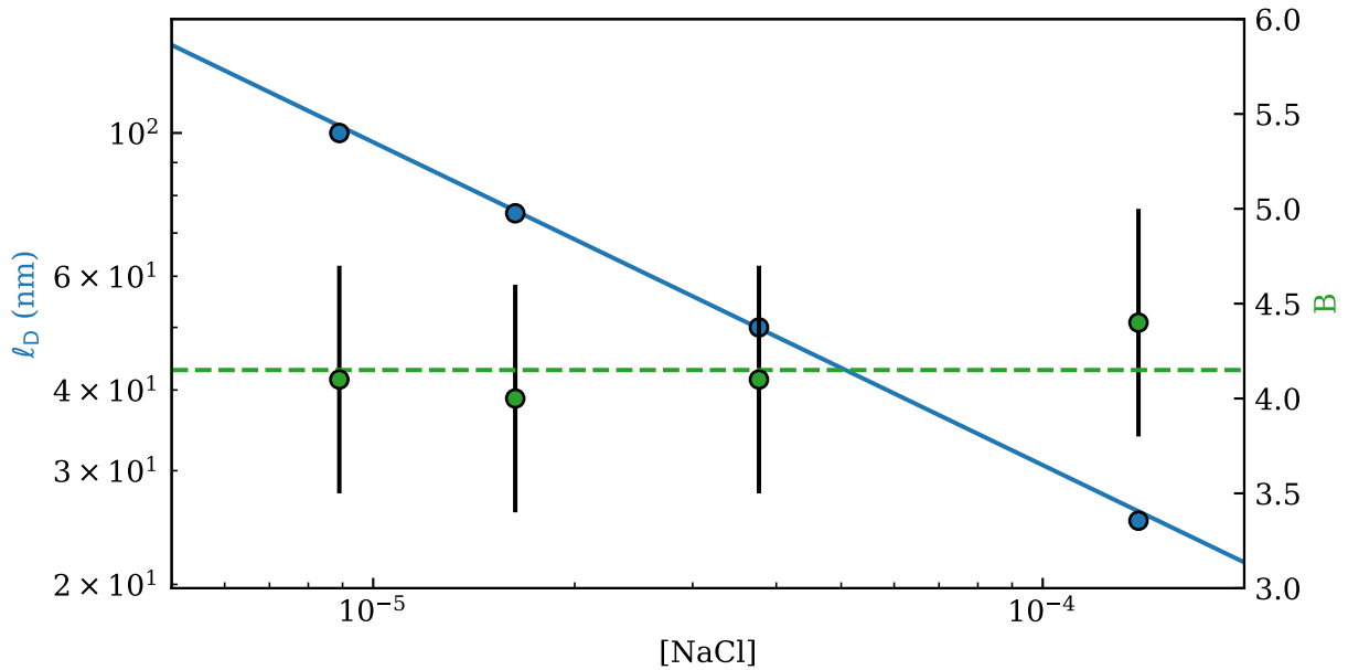
Figure 5.2.3: In blue, left axis, measured Debye length \ell_D as a function of salt concentration [\text{NaCl}] . The solid line is the expected Debye relation \ell_D = 0.304/\sqrt{[\text{NaCl}]} , for a single monovalent salt in water at room temperature. In green, right axis, measured B as a function of salt concentration [\text{NaCl}] . The dashed line represents the mean value of the measured B values. \odot
