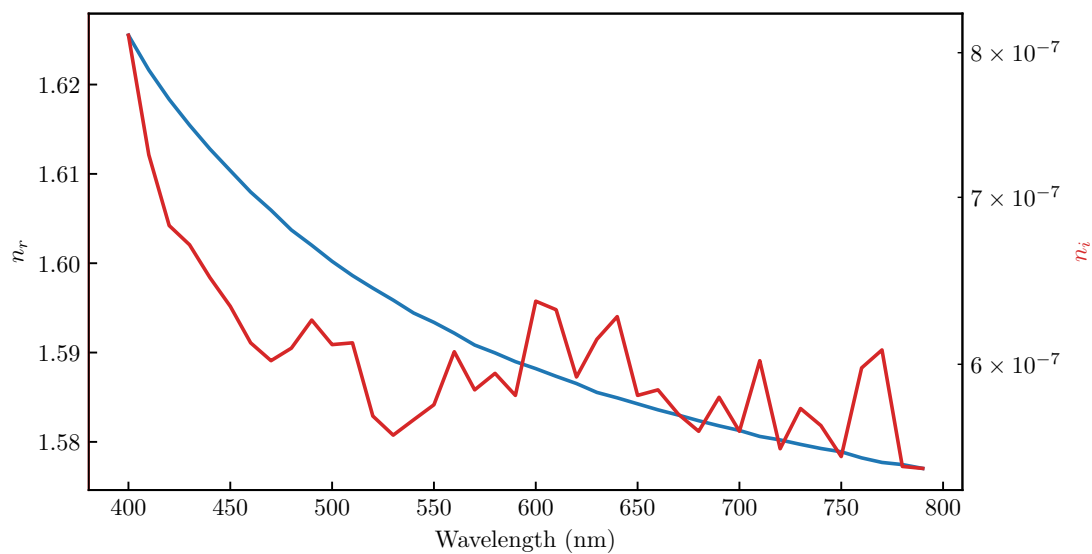
Figure 4.6.1: Real (left axis) and imaginary (right axis) part of the refractive index of polystyrene as a function of the incident wavelength. Data obtained from [71].
