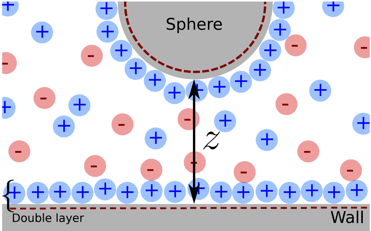
Figure 5.1.2: A colloid diffusing near a wall. Both the wall and colloid surfaces charge negatively. As a consequence, a layer of positively-charged ions is attracted towards each surface, forming a double layer.
