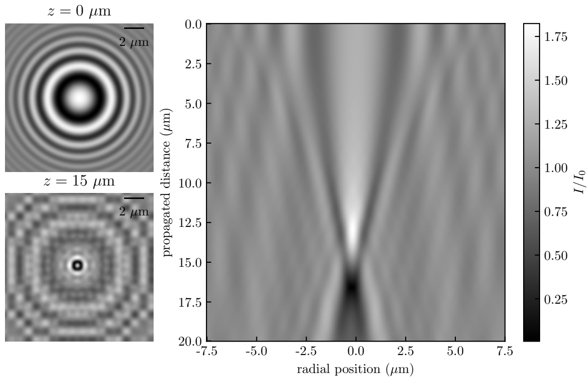
Figure 4.4.1: On the left: the original hologram on the top and propagated along 15 \mu\text{m} on the bottom. On the right: reconstruction using Eq. (4.4.5) of the scattered intensity by a single colloidal sphere of radius a = 0.1 \mu\text{m} , with optical index n_p = 1.59 in water whose index is n_m = 1.59 , and for a height of 15 \mu\text{m} . 🌀
