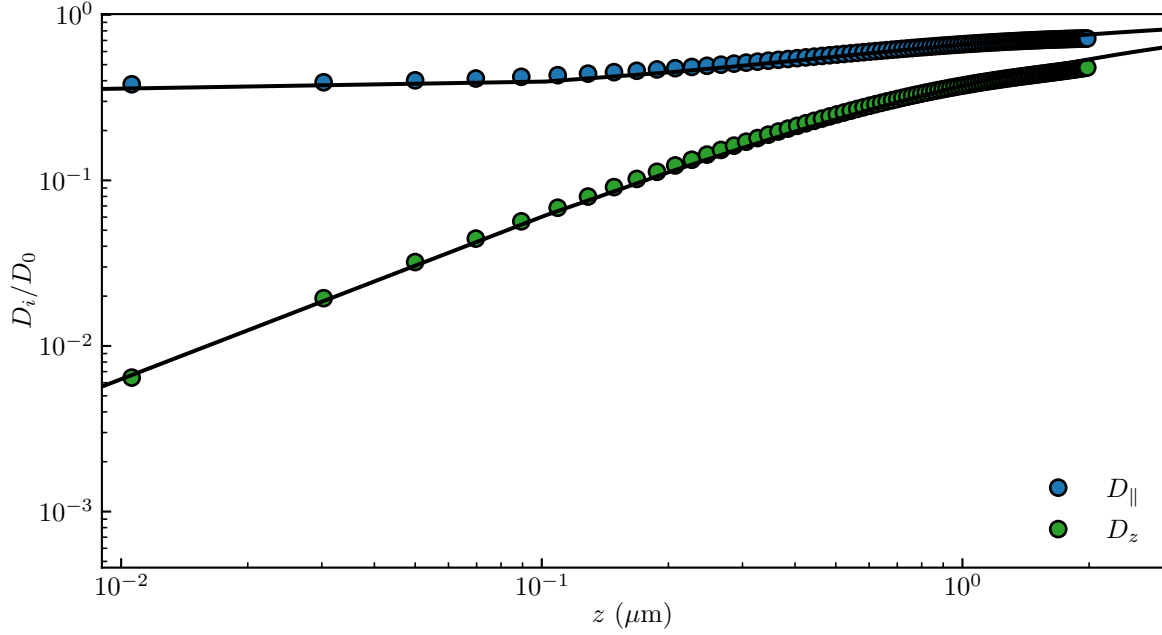
Figure 5.2.7: Measured local short-term diffusion coefficients D_i of the microparticle, normalized by the bulk value D_0 , as functions of the distance z to the wall, along both a transverse direction x or y ( D_i = D_{\parallel} = D_x = D_y , blue) and the normal direction z ( D_i = D_z , green) to the wall. The solid lines are the theoretical predictions, D_{\parallel}(z) = D_0\eta/\eta_{\parallel}(z) and D_z(z) = D_0\eta/\eta_z(z) , using the local effective viscosities \eta_{\perp}(z) and \eta_{\parallel}(z) of Eqs. (5.1.46) and (5.1.47), respectively. \odot
