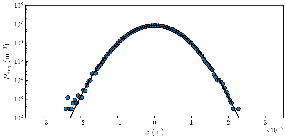
Figure 6.2.5: Measured equilibrium probability distribution function P_{Heq} of the position x of the stuck particle. The solid line represents the best fit to the normalized Gibbs-Boltzmann distribution in position a particle in an harmonic potential (see Eq. (6.2.2)) for k_{kH} = 1.738 \pm 0.004 \mu\text{N.m}^{-1} .
