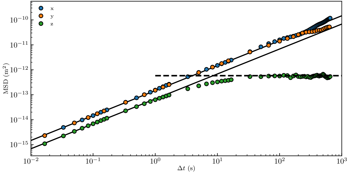
Figure 5.2.4: Measured mean-squared displacements (MSD, see Eq. (5.2.1)) as functions of the time increment \Delta t , for the three spatial directions, x , y , and z . The solid lines are best fits to Eq. (5.2.2), using Eqs. (5.1.28), (5.1.46) and (5.1.47), with B = 4.8 , \ell_D = 21 nm, and \ell_B = 530 nm, providing the average diffusion coefficients \langle D_{\parallel} \rangle = \langle D_x \rangle = \langle D_y \rangle = 0.52 D_0 and \langle D_z \rangle = 0.24 D_0 . The dashed line is the best fit to Eq. (5.2.9), using Eq. (5.1.28), with B = 4.8 , \ell_D = 21 nm, and \ell_B = 530 nm. \odot
