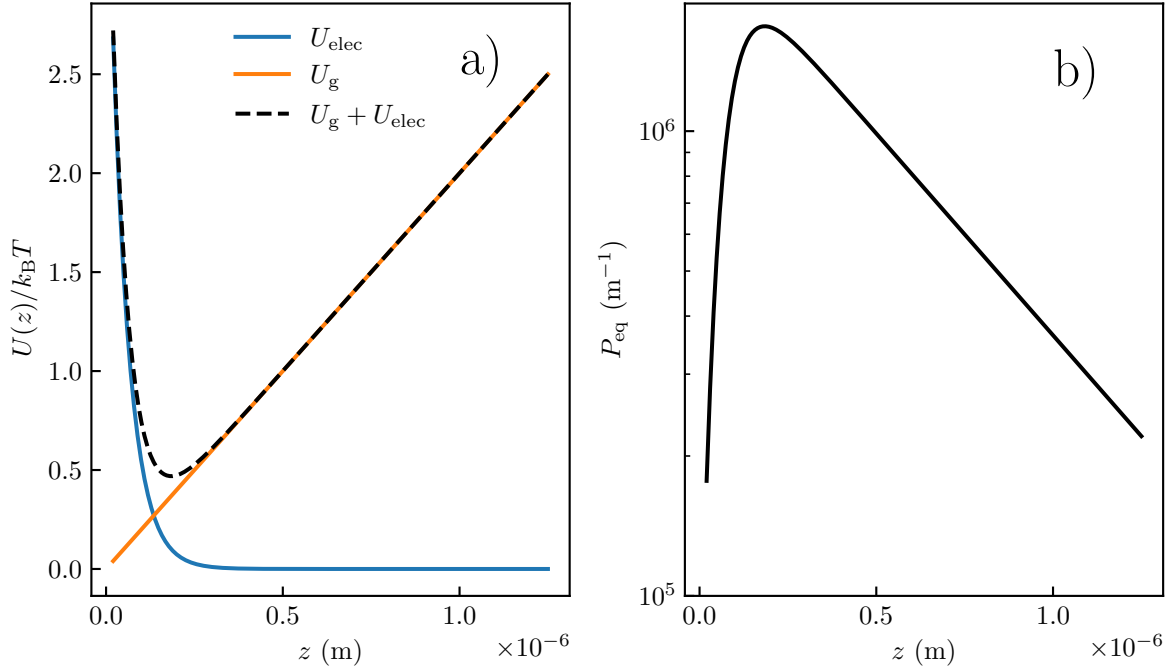
Figure 5.1.4: a) In orange potential energy U_g (see Eq. (5.1.3)) of a colloid with a Boltzmann length \ell_B = 500 nm. In blue, the electrostatic potential energy U_{\text{elec}} (see Eq. (5.1.22)) is characterized by a dimensionless magnitude B = 4 and a Debye length \ell_D = 50 nm. The dashed line corresponds to the total potential U , see Eq. (5.1.27). b) Corresponding Gibbs-Boltzmann equilibrium distribution of position calculated using the energy potential of panel a). \odot
