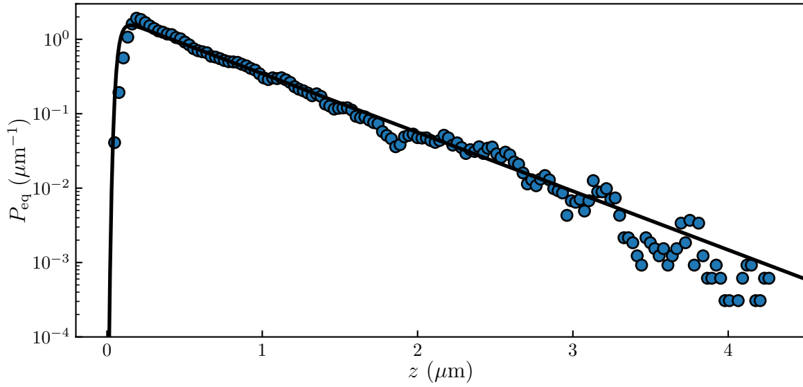
Figure 5.2.2: Measured equilibrium probability density function P_{\text{eq}} of the distance z between the particle and the wall. The solid line represents the best fit to the normalized Gibbs-Boltzmann distribution in position, using the total potential energy U(z) of Eq. (5.1.28), with B = 4.8 , \ell_D = 21 nm, and \ell_B = 530 nm. \odot
