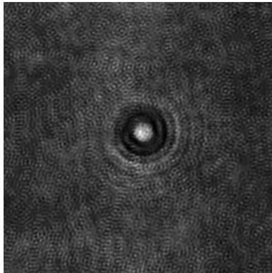
Figure 6.2.1: Median of the a movie of the hologram of a stuck yet moving particle. The median is calculated over 120 images taken every 30 s.
