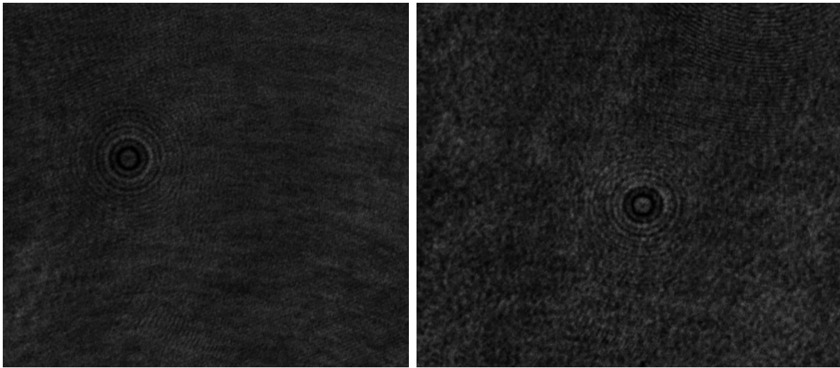
Figure 6.4.1: Hologram of a particle diffusing above a soft surface ( G = 1.5 kPa). The image on the right has been taken 3 hours after the one on the left. The images are 45 \mu\text{m} wide and 50 \mu\text{m} tall.
