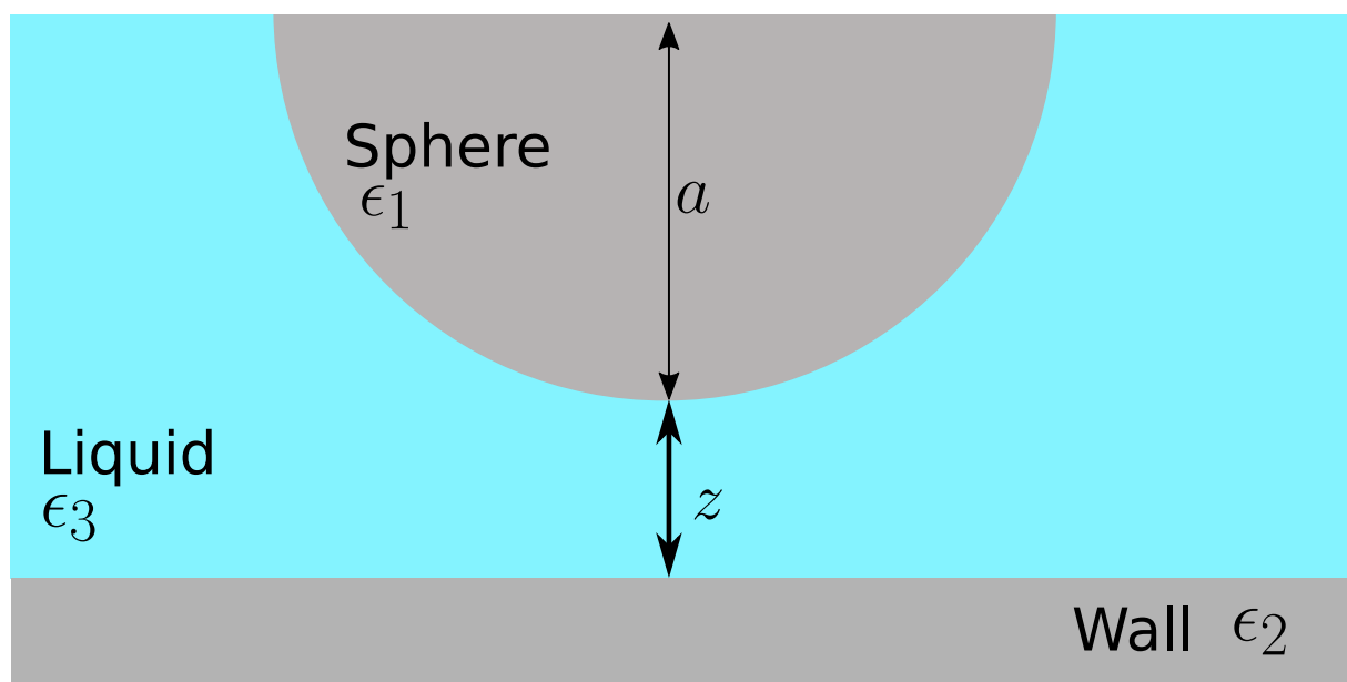
Figure 5.1.3: A colloid of radius a is located at a distance z from the wall. The dielectric constants of the sphere, wall and liquid are respectively \epsilon_1 , \epsilon_2 , and \epsilon_3 .
