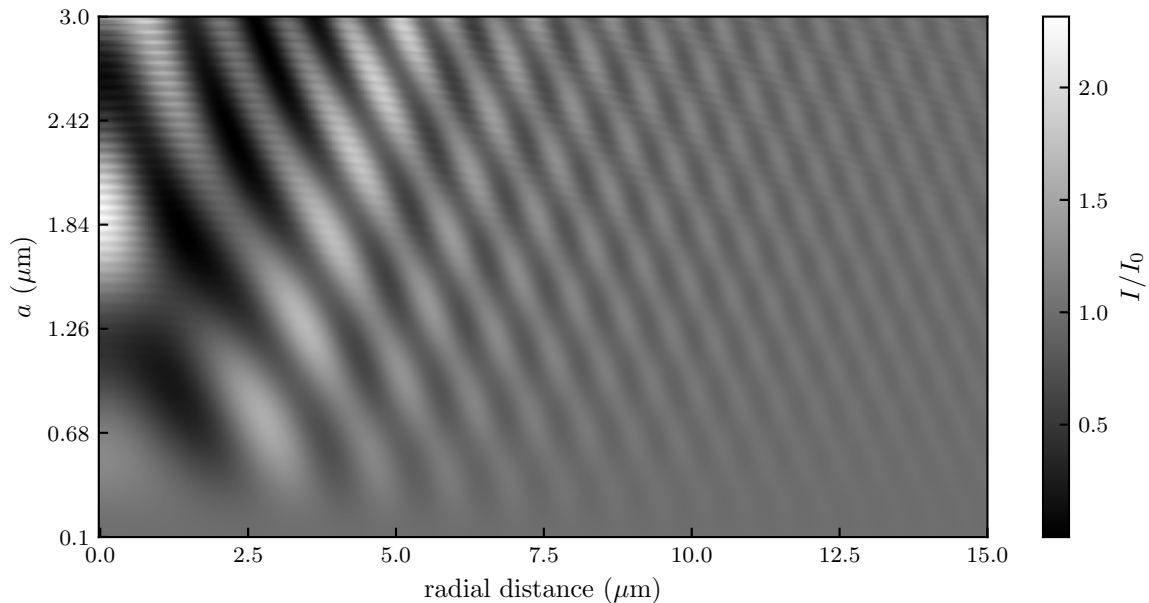
Figure 4.3.3: Hologram intensity map in the (r, a) -plan, calculated (see. Eq. (4.3.4)) with a wavelength \lambda = 532 nm for a particle of optical index n = 1.59 , and a distance z = 15 \mu\text{m} between the particle center and the focal plane of the objective lens. 🔄
