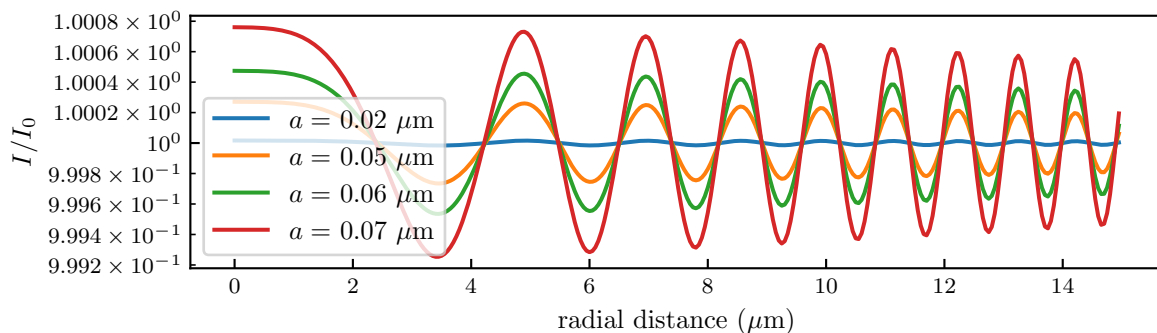
Figure 4.3.4: Radial intensity profile for particle radius a \ll \lambda , and an optical index n_p = 1.59 with a distance z = 15 \mu\text{m} between the particle center and the focal plane of the objective lens, and for a wavelength \lambda = 532 nm. 🔄
