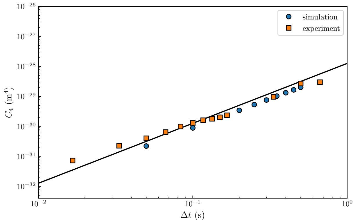
Figure 6.3.2: Experimentally measured 4th cumulant of the transverse displacement as a function of time increment . The plain line corresponds Eq. (6.3.3) calculated using Eqs (5.1.47) and (5.1.29) with with B = 4.8 , \ell_D = 21 nm, and \ell_B = 530 nm.
