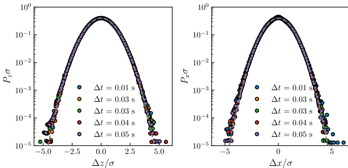
Figure 6.2.4: Normalized probability density functions P_i \sigma of the normalized displacements \Delta x/\sigma and \Delta z/\sigma , at short times, with \sigma^2 the corresponding MSD (see Fig. 6.2.3), for different time increments \Delta t ranging from 0.01 s to 0.05 s, as indicated with different colors. The gray dashed lines are normalized Gaussian distributions, with zero means and unit variances.
