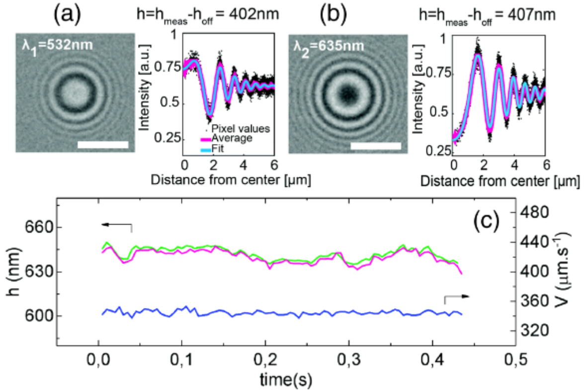
Figure 4.2.1: Figure from [45] representing RICHM with two wavelengths. (a) Left: interference patterns created with a wavelength \lambda_1 = 532 \text{ nm} (scale bar 5 \mu\text{m} ). Right: radial intensity profile (black dots) extracted from the image, azimuthally averaged (magenta line) and fitted with Eq. (4.2.8) to measure the height of the particle (here noted h ). (b) Same as (a) with a wavelength \lambda_2 = 635 \text{ nm} . (c) Time series of the height h of a particle (green: \lambda_1 , purple: \lambda_2 ) and the particle velocity measured along the flow (in blue).
