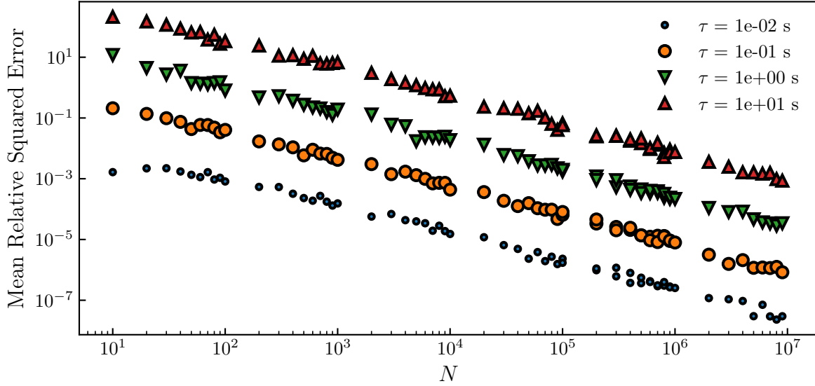
Figure 3.4.2: Mean Relative Squared Error (MRSE) of the Probability Density Function PDF measured from a generation of N Gaussian random numbers w_i and the actual Gaussian (see Eq. (3.4.3)) from which the generation is done. The generation is done over a Gaussian which has a mean value \langle w_i \rangle = 0 and variance \langle w_i^2 \rangle = \tau . We explore parameter ranges from N = 10 to 10^7 and \tau = 10^{-2} to 10 s. 🔄
