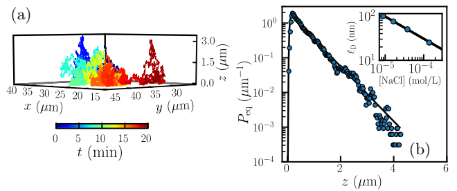
FIG. 3. (a) Typical measured tridimensional trajectory \mathbf{r}(t) = [\mathbf{x}(t), \mathbf{y}(t), \mathbf{z}(t)] of the microparticle near the wall ( z = 0 ). (b) Measured equilibrium probability density function P_{\text{eq}} of the distance z between the particle and the wall. The solid line represents the best fit to the normalized Gibbs-Boltzmann distribution in position, using the total potential energy U(z) of Eq. (1), with B = 4.8 , \ell_D = 21 nm, and \ell_B = 530 nm. The inset shows the measured Debye length \ell_D as a function of salt concentration [\text{NaCl}] . The solid line is the expected Debye relation \ell_D = 0.304/\sqrt{[\text{NaCl}]} , for a single monovalent salt in water at room temperature.
