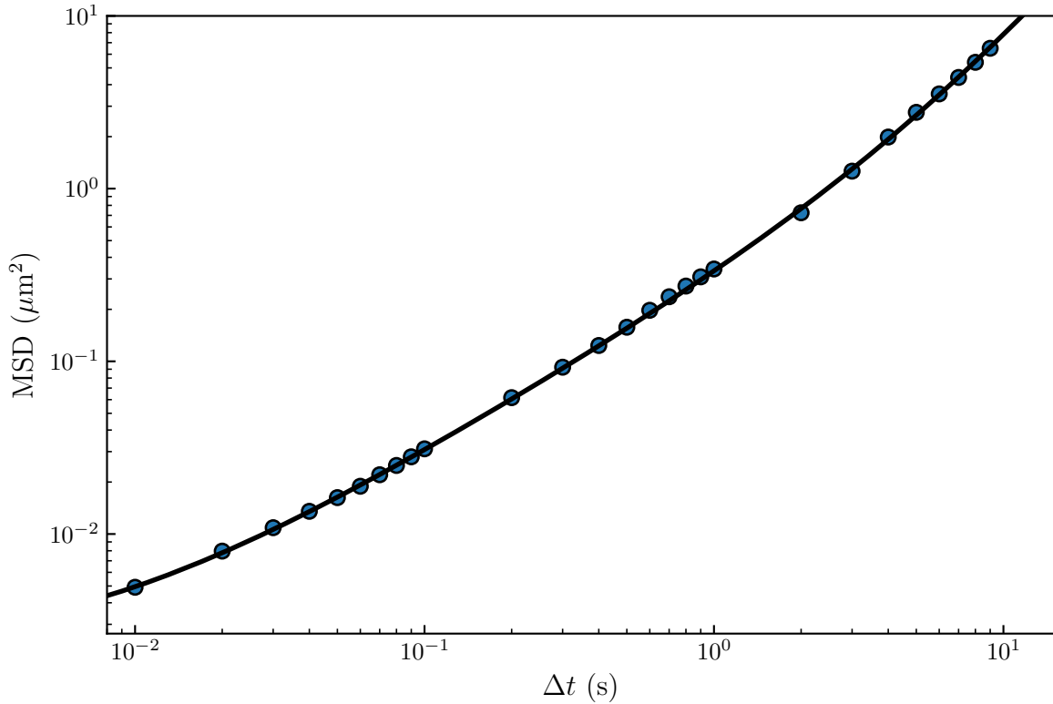
Figure 4.7.4: Measured mean-squared displacement as a function of the time increment \Delta t , along the z -axis. The solid line is the best fit to Eq. (4.7.2), with D_0 = 144 \pm 1 \mu\text{m}^2.\text{ms}^{-1} , v_{\text{sed}} = 222 \pm 1 \text{ nm.s}^{-1} and \xi = 25 \text{ nm} .
