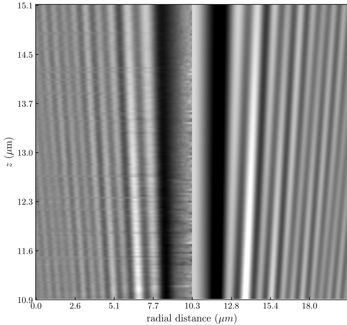
Figure 4.3.6: Hologram intensity map in the (r, z) -plan, calculated (see. Eq. (4.3.4)) with a wavelength \lambda = 532 \text{ nm} , for a particle of optical index n = 1.59 , and radius a = 1.51 \mu\text{m} using the experimental setup presented in the section 4.5. On the right, the corresponding theoretical intensity using the result of each individual hologram's fit to Eq. (4.3.5).
