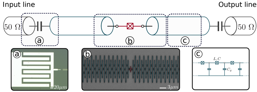
Figure 1.1 – Schematic of the first designed circuits. The SQUID chains, depicted as blue transmission lines, are capacitively coupled to the input and output 50 \Omega coaxial cables and galvanically coupled to the nonlinear Josephson junction (in red). a Optical picture of the input and output capacitive coupling pads. b SEM picture of a few of the SQUIDs (1500 in total for each chain) that are coupled to the nonlinear Josephson junction (in red). c Equivalence between the transmission line effective picture and the SQUID chain characterized by three microscopic parameters L and C the inductance and capacitance per SQUID respectively and C_g the ground capacitance.
