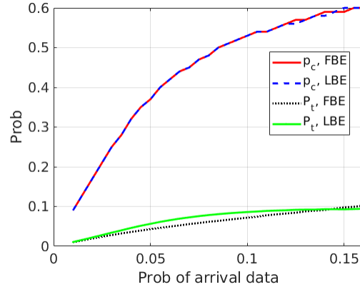
Figure 7.2: Probability of sensing a busy channel and transmission probability of a UE using FBE and LBE.
