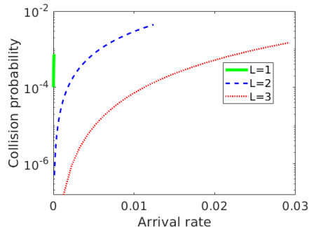
Figure 2.9: The arrival rate vs collision probability.
