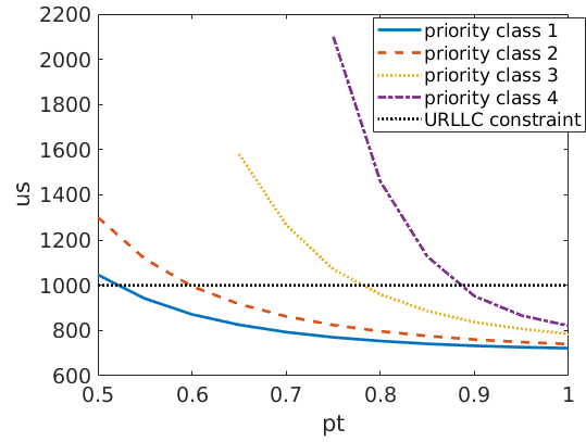
Figure 5.6: Total transmission time in UL transmission with 4 repetitions in SCS of 30kHz.
