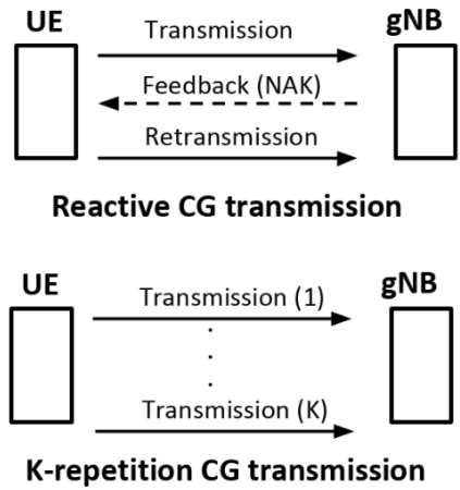
Figure 1.2: UL repetition CG transmission.
