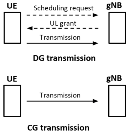
Figure 1.1: UL DG and CG transmission.
