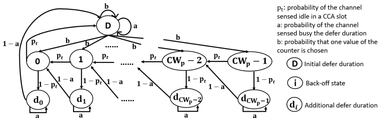
Figure 5.1: Markov chain for Type 1 channel access procedures.
