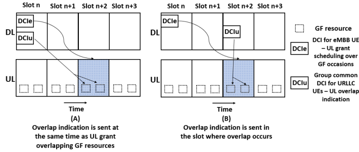
Figure 3.4: Timing to send the UL Overlap Indication.
