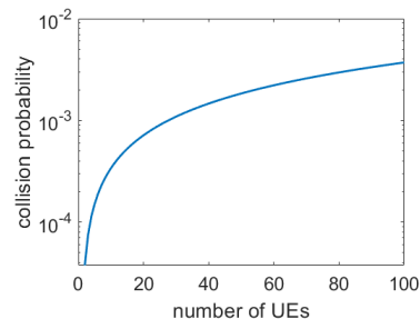
(a) Collision probability with respect to the number of the UEs.
