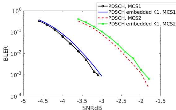
Figure 4.6: Performance of normal PDSCH and PDSCH embedded dynamic K1 indication.
