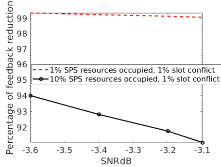
Figure 4.5: The reduction of feedback in ACK-only feedback structure.
