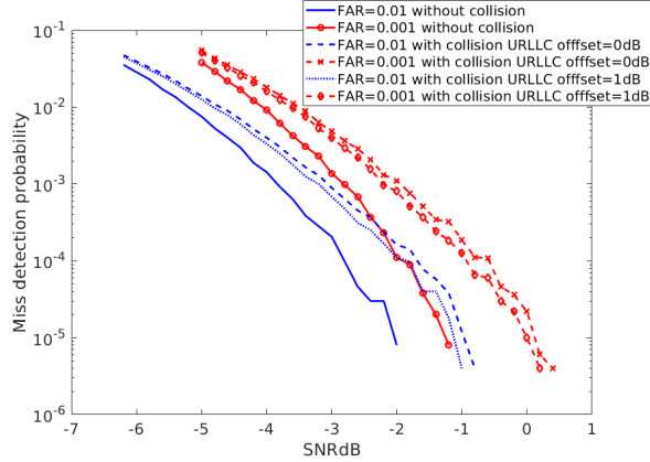
Figure 3.5: DMRS detection performance.
