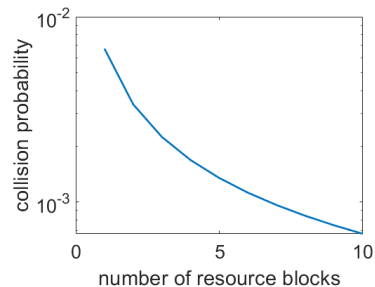
(b) Collision probability of the second reserved resource.
