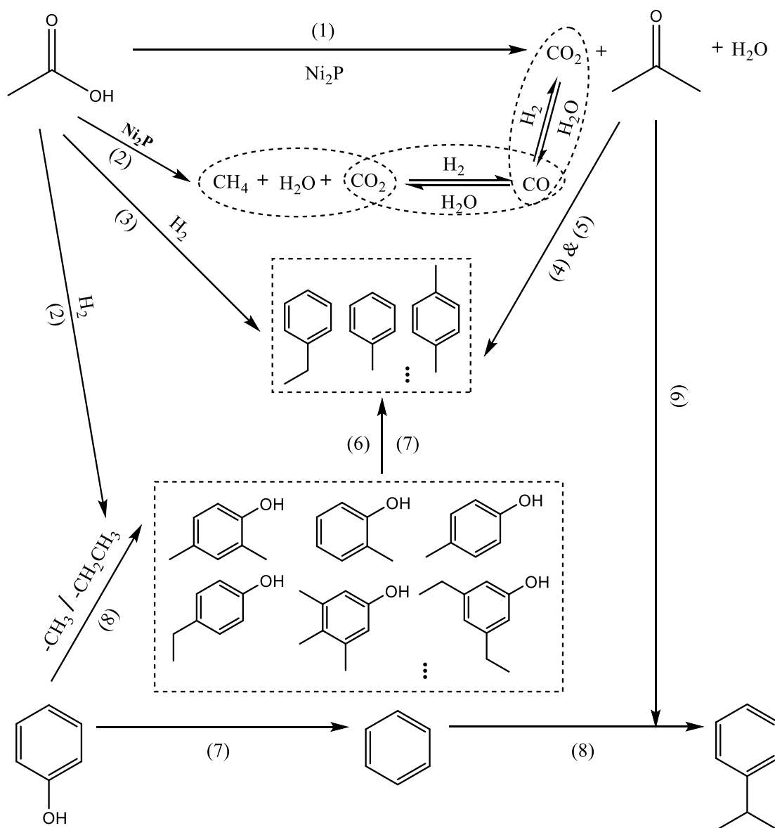
Figure 5.6 Proposed interaction network of Mixture 1 HDO on Ni 2 P/HZSM-5 catalysts: (1) Self-condensation; (2) Decarboxylation; (3) Condensation; (4) Adol condensation; (5) Isomerization; (6) Dealkylation; (7) Dehydroxylation; (8) Alkylation substitution; (9) Deoxygenation
