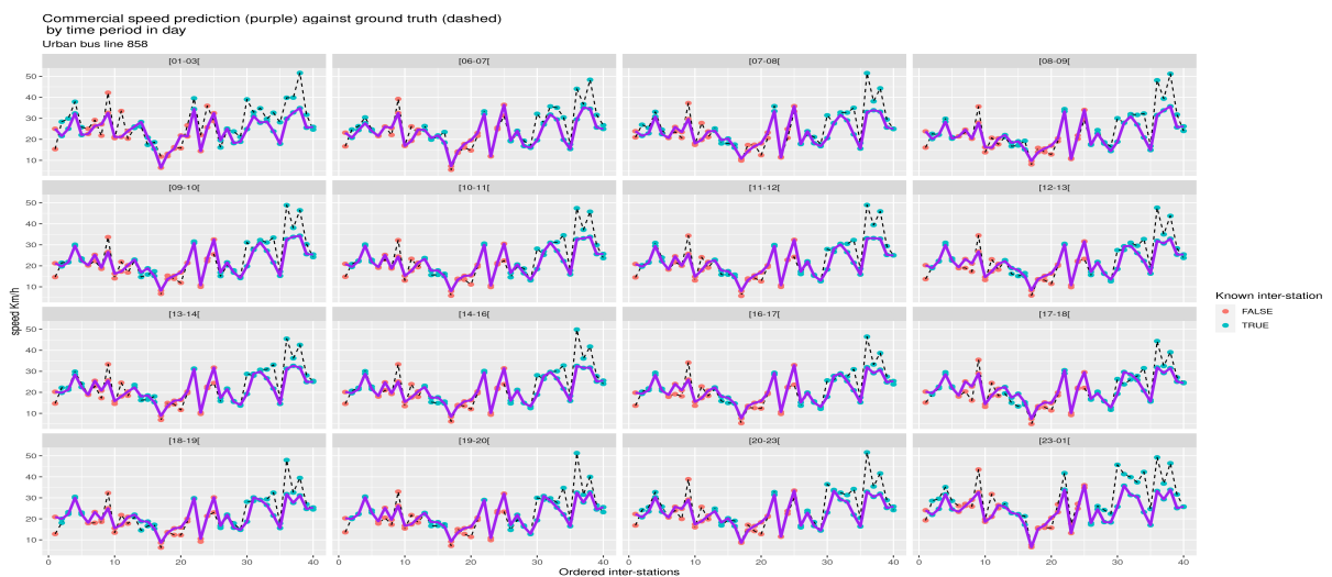
Figure 4.3 – Speed of urban bus line 858 at inter-stations using micro-learning (purple) vs true speed (dashed). Orange inter-stations were not used by any other bus, i.e. are absent from the training set.
