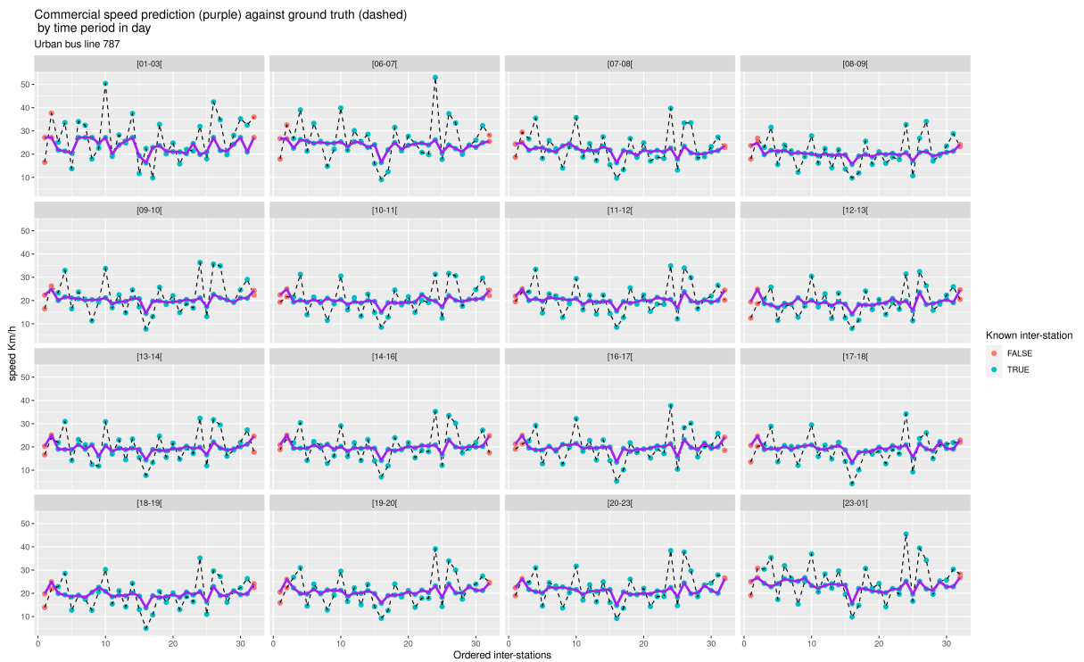
Figure A.4 – micro-predictions of bus line 787 with and without OSM features
