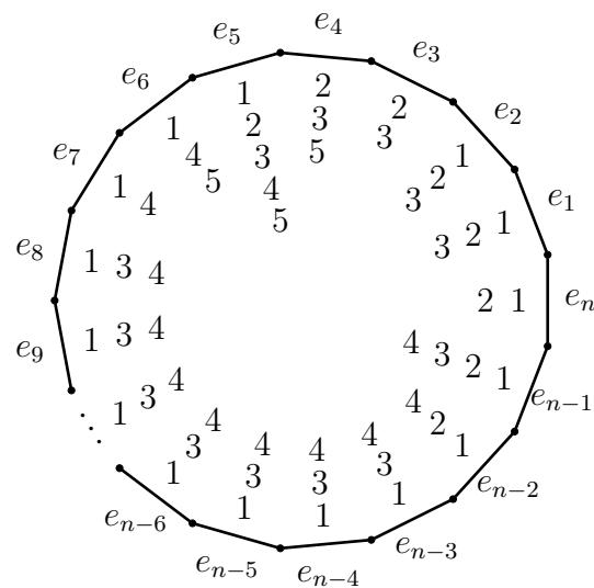
(c) Case: n \equiv 2 \pmod{3} .
