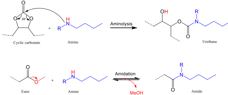
Figure 29. Reaction scheme for aminolysis and amidation reactions.
