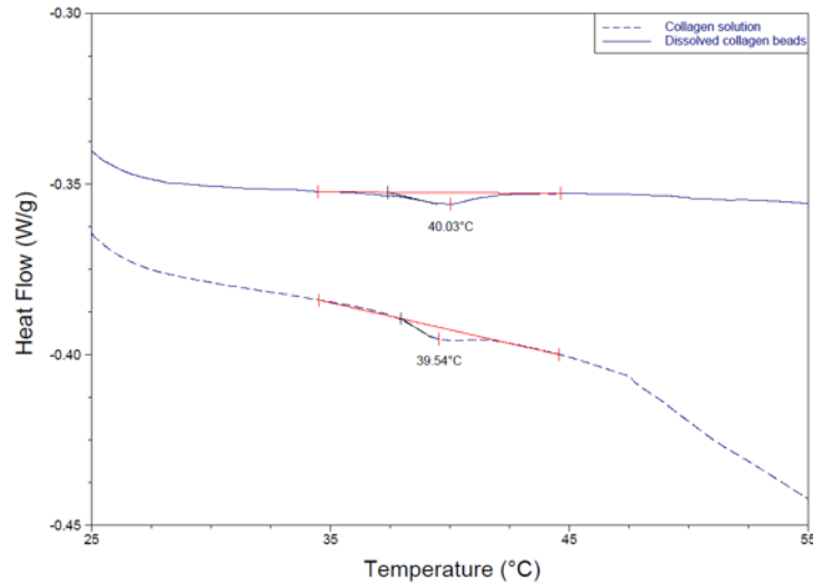
Figure 2.10: Differential Scanning calorimetry of a collagen solution (dashed line) and of a solution made of dissolved collagen beads (solid line). The endothermic peak, typical of collagen triple helix denaturation, occurs at the same temperature for both solutions thus proving that no denaturation occurred during the whole spray-drying process. (SI)
