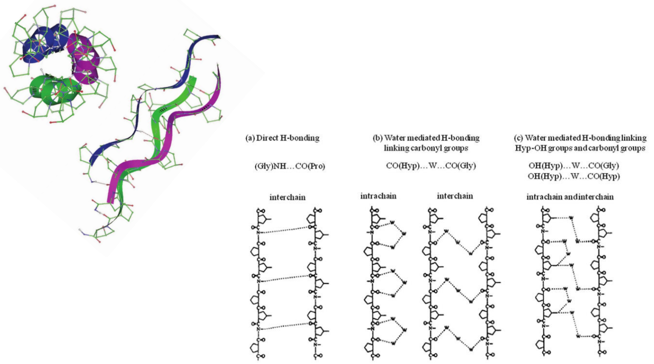
Figure 1.3: Top left: Collagen triple helix, top view on the left, side view on the right. Reproduced from Bhattacharjee 2005 [8]; bottom right: hydrogen bonding possibilities between neighbouring amino acids in the triple helix. Reproduced from Nguyen 2013 [10].
