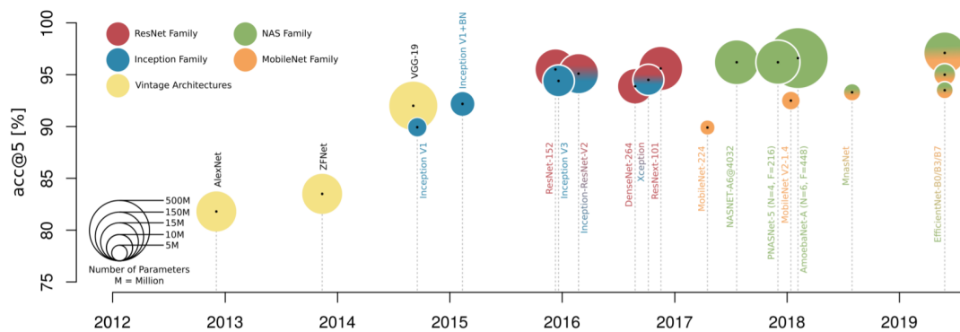
Figure 2.7: Performance evaluation for basic CNN-based architecture from 2012 to 2019 carried on ImageNet 2012 dataset [69]
