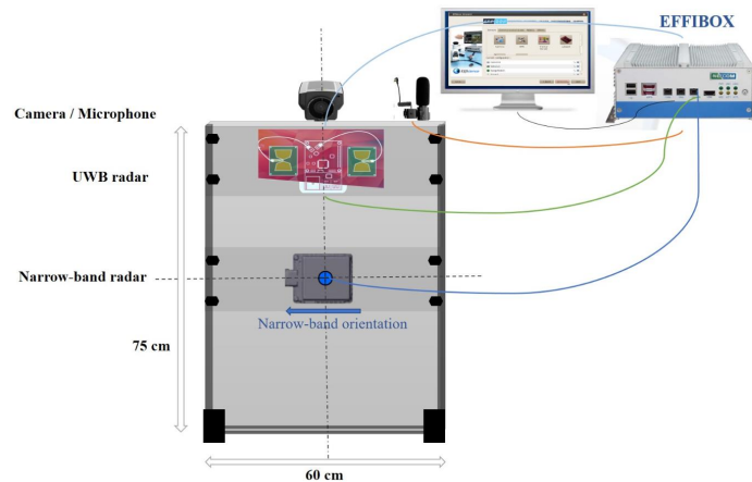
Figure 3.3: Structure setup
