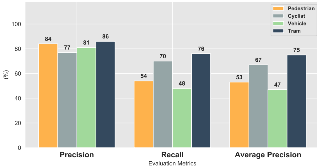
Figure 3.10: MobileNet results (%)
