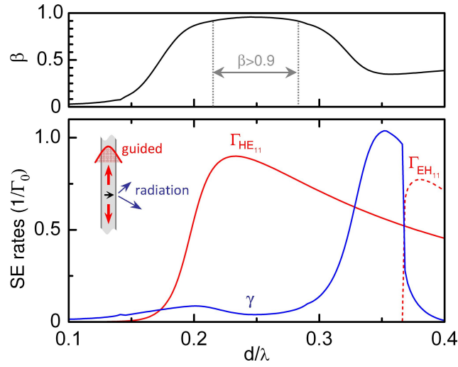
Fig. 1.15 SE dynamics for an on-axis emitter. (Bottom panel) Normalised SE rate into the fundamental HE_{11} mode (red), radiation modes (blue), EH_{11} mode, as a function of d/\lambda for an on-axis transverse optical dipole with \lambda = 950 nm, embedded in an circular, infinitely long wire. (Top panel) The \beta -factor as a function of d/\lambda . [75].
