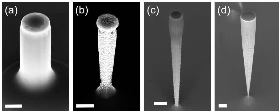
Fig. 4.8 A timeline of a few selected results leading to the definition of our recipe for ICP etching of GaAs trumpets. (a) The base recipe we picked served to etch cylindrical GaAs nanowires. This recipe was modified to etch trumpets. (b) Elevated sample temperature, T = 140^\circ\text{C} . (c) Reduced RF power to 90 W. (d) Increased all gas flow rates. The scale bar on each image represents 1\ \mu\text{m} .
