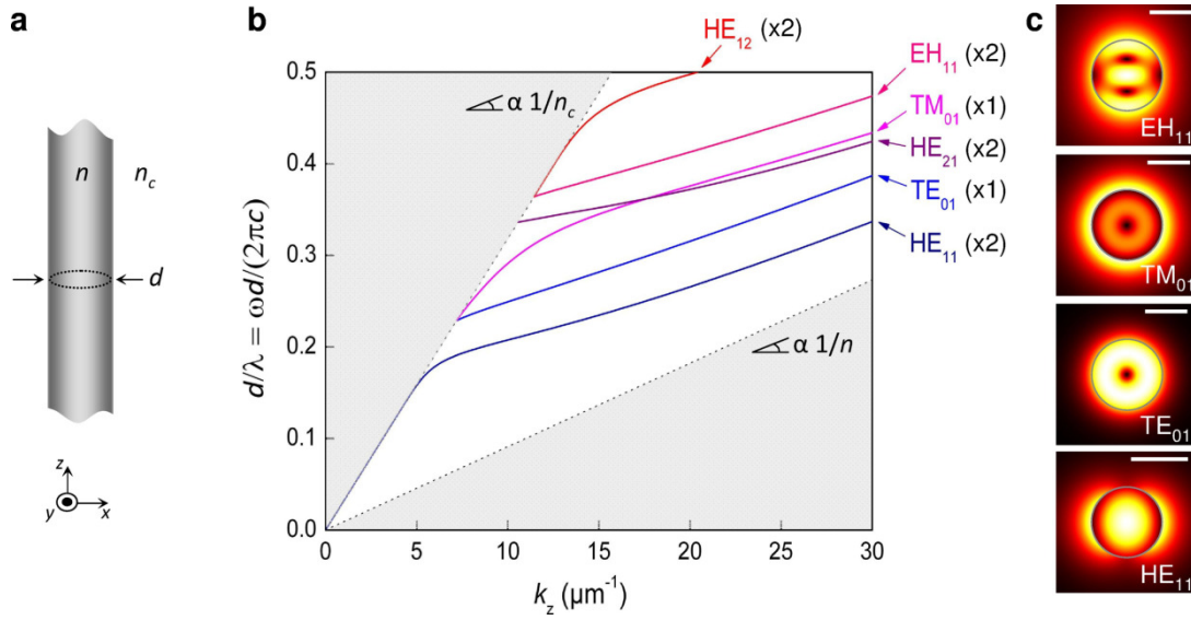
Fig. 1.13 Guided modes of an infinitely long cylindrical GaAs wire. (a) The geometry of the cylindrical waveguide. (b) Dispersion curves of the first guided modes of the wire. d/\lambda = \omega d/(2\pi c) is plotted as a function of the propagation constant k_z . The polarisation degeneracy is indicated within brackets beside the mode label. (c) In-plane electric field amplitude for the first few guided modes. The map of HE_{11} is plotted for d/\lambda = 0.25 while the others are plotted for d/\lambda = 0.37 . The scale bars represent 200 nm. [144].
