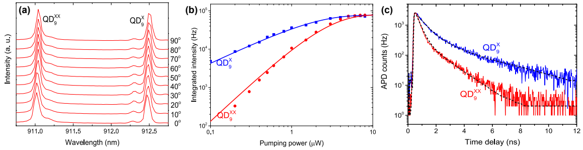
Fig. 3.23 (a) Micro-PL spectrum of an exciton-biexciton pair hosted by \text{QD}_9 . The exciton \text{QD}_9^X emission line is positioned at 912.5 \text{ nm} and the biexciton \text{QD}_9^{XX} at 911 \text{ nm} . (b) Integrated intensity plots for \text{QD}_9^X (blue) and \text{QD}_9^{XX} (red) both saturating at 77 \text{ kHz} . At low pumping power the data of \text{QD}_9^X ( \text{QD}_9^{XX} ) display a linear (quadratic) dependence. (c) Time-resolved measurement of decay time for \text{QD}_9^X (blue) and \text{QD}_9^{XX} (red) corresponding to radiative rates of \Gamma_{rad}^X = 1.9 \text{ ns}^{-1} and \Gamma_{rad}^{XX} = 3.8 \text{ ns}^{-1} .
