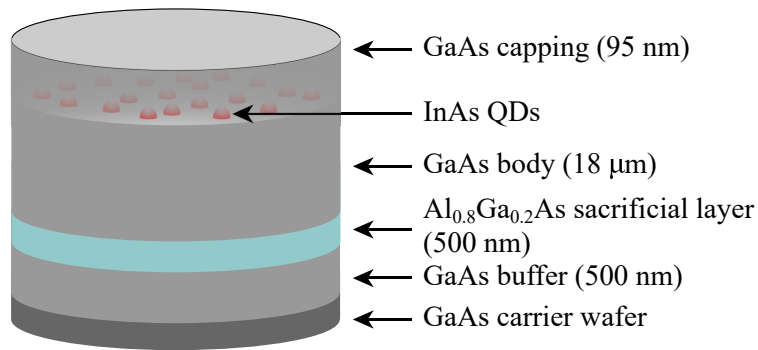
Fig. 4.10 Planar heterostructures used for the fabrication of trumpets.
