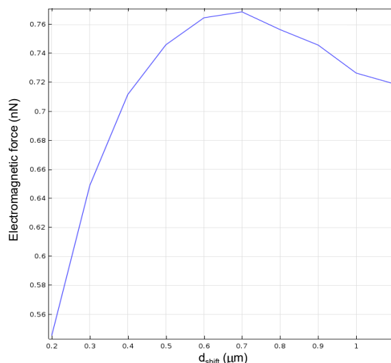
Fig. 4.5 The electrostatic force at the trumpet top facet as a function of separation offset d_{shift} = d_2 - d_1 between the electrodes and the trumpet. A potential difference of 50 V was applied across E_1 and E_2 .
