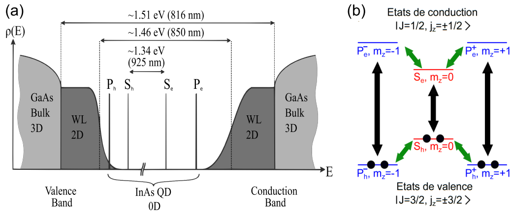
Fig. 1.7 Electronic states of an InAs/GaAs QD. (a) Schematic diagram of the density of states corresponding InAs/GaAs QD system. Values of energy gaps indicated here correspond to typical values at T \approx 4K for QDs used in this work. (b) The ground state of the QD with its valence band completely occupied by electrons, represented by black dots. The arrows correspond to the allowed transitions between the different envelop states. Black arrows represent interband transitions, while green arrows represent intraband transitions. Figures adapted from Ref. [101].
