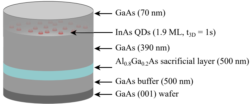
Fig. 3.7 Planar heterostructures used for the fabrication of nanocavities.
