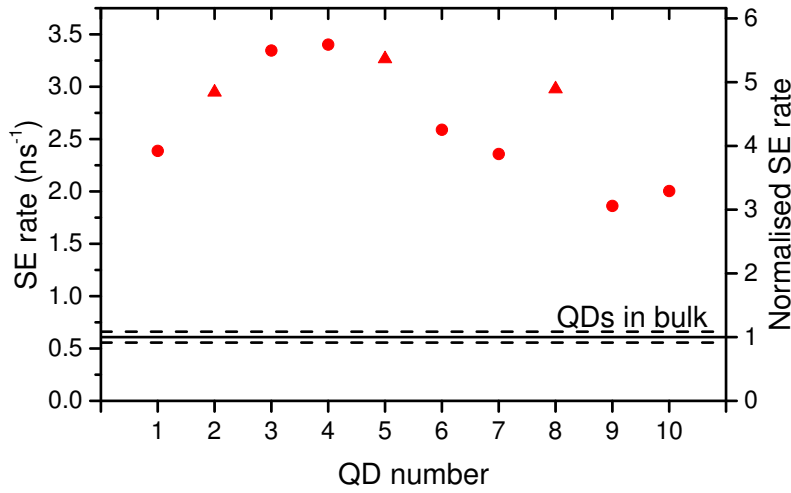
Fig. 3.20 SE rate of individual QDs embedded in nanocavities. Disks (triangles) correspond to neutral (charged) excitons. The SE rate of similar QDs embedded in bulk GaAs serves as a reference (horizontal solid line represents a mean value, and the dashed lines delineate \pm 1 standard deviation).
