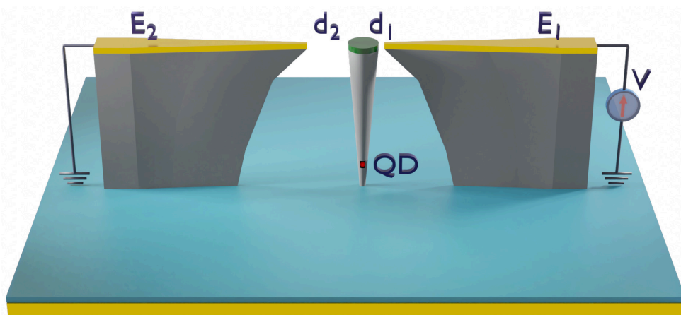
Fig. 4.4 Design of the electrostatically-tuned SPS. E_1 and E_2 represent the tuning electrodes with an Au coating indicated in yellow. The QD is housed near the base of the trumpet represented by the red triangle. The entire system sits on a \text{SiO}_2 -Au mirror. The simulated design consists of a 20\ \mu\text{m} -tall trumpet with a top diameter of 3.5\ \mu\text{m} .
