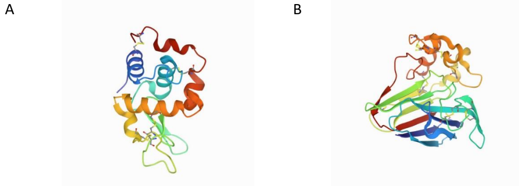
Figure 1. Structures of A) hen egg white lysozyme at 1.33 Å. PDB code: 193L and B) Thaumatin at 1.05 Å. PDB code: 1RQW [17].
