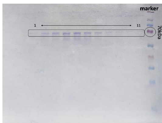
Figure 29. Purification of ShuA by affinity chromatography using a NiNTA column. A 10 % SDS PAGE gel was used and 5 \mu L of the solution containing 10 \mu L of the fraction and 2.5 \mu L of Coomassie Blue was loaded into each well of the gel. The samples were not boiled before loading onto the gel.
