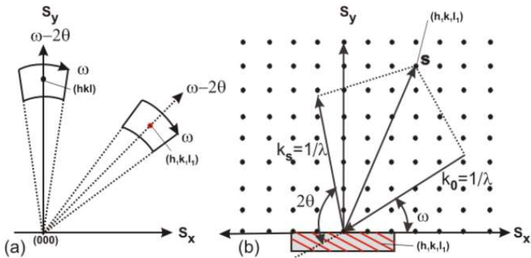
Figure 2. 12 (a) Scans in reciprocal space for two different reciprocal lattice points (hkl) (symmetric) and (h_1k_1l_1) (asymmetric). (b) Reciprocal space construction for the asymmetric reflection (h_1k_1l_1) . k_s and k_0 are the wave vectors for the diffracted and the incident X-rays, respectively. S = k_0 + k_s is the scattering vector. Taken from Ref. 34.
