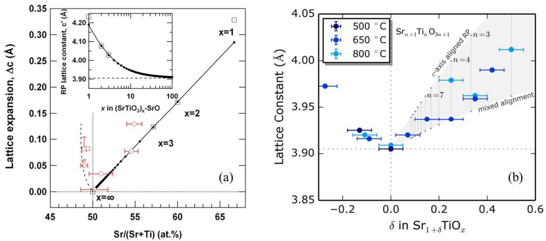
Figure 5. 1 (a) Lattice expansion as a function of Sr/(Sr+Ti) cationic ratio. The closed circles are the calculated data and open squares are the reported bulk values. Taken from Ref. 4. (b) The apparent out-of-plane lattice constant measured by XRD for \text{Sr}_{1+\delta}\text{TiO}_x films versus Sr:Ti stoichiometry ratio determined by RBS. Taken from Ref. 5.
