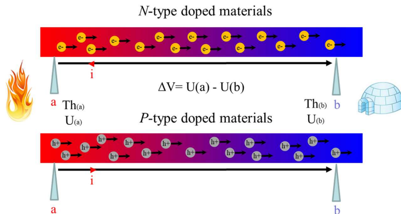
Figure 2. 17 Charge carrier migration of n -type (top) and p -type (bottom) thermoelectric materials during Seebeck measurement.
