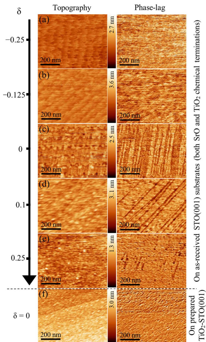
Figure 3. 11 Tapping mode AFM: topographic (left panel) and phase-lag (right panel) images of the LCO epitaxial thin films grown on as-received \text{STO}(001) substrate with (a) \delta = -0.25 , (b) \delta = -0.125 , (c) \delta = 0 , (d) \delta = 0.1 , and (e) \delta = 0.25 . (f) LCO thin film grown on prepared \text{TiO}_2 -terminated \text{STO} substrate with \delta = 0 . Taken from Ref. 1.
