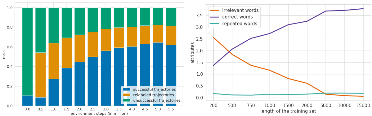
Figure 4.6: Transition distributions in the replay buffer between successful, unsuccessful and relabelled trajectories. We remove time-out trajectories for clarity, which accounts for 54% of the transition in average ( \pm 3\% over training). Right: Evaluating the language learned by the instruction generator on unseen instructions. Over time, the number of correct attributes (purple) is increasing, as the number of irrelevant words (orange) is decreasing. The number of repeated attributes (green) stays low. The beginning clause is ignored as it doesn't provide information regarding the objective.
