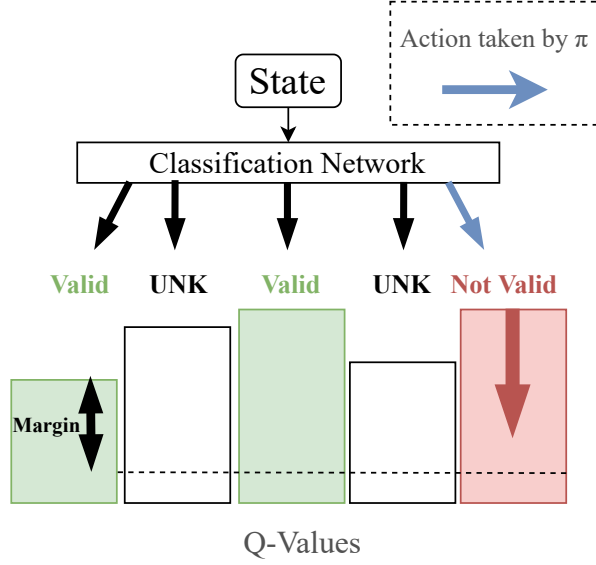
Figure 2.4: Illustration of frontier loss.
