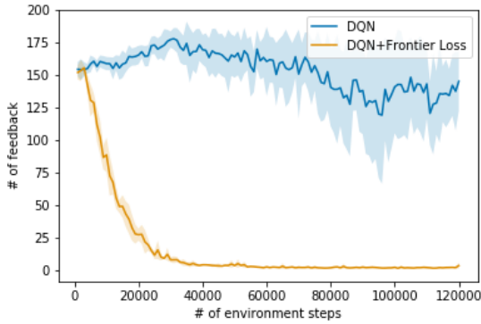
Figure 2.8: DQN- \mathcal{F} (yellow) DQN (blue), the shaded area represents one standard deviation. Results are averaged over 5 random seeds. Left: Number of times a forbidden action is taken. Right: Percentage of success over time.
