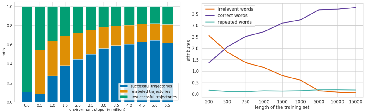
Figure 4.6: Transition distributions in the replay buffer between successful, unsuccessful and relabelled trajectories. We remove time-out trajectories for clarity, which accounts for 54% of the transition in average ( \pm 3\% over training). Right: Evaluating the language learned by the instruction generator on unseen instructions. Over time, the number of correct attributes (purple) is increasing, as the number of irrelevant words (orange) is decreasing. The number of repeated attributes (green) stays low. The beginning clause is ignored as it doesn't provide information regarding the objective.
