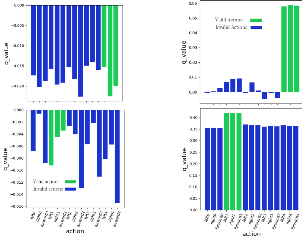
Figure 2.10: Top: Q -values, after 150 episodes of training (30 000 environment steps) for a handpicked state. Bottom: Q -values, after 100 000 training steps on another state.
