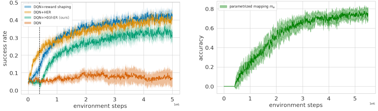
Figure 4.4: Left: learning curves for DQN, DQN+HER, DQN+HIGHhER in a 10x10 gridworld with 10 objects with 4 attributes. The instruction generator is used after the vertical bar. Right: the mapping accuracy for the prediction of instructions. m_w starts being trained after collecting 1000 positive trajectories. Results are averaged over 5 seeds with one standard deviation.
