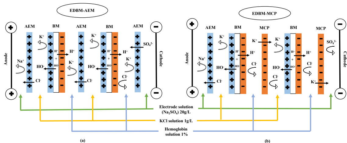
Figure IV-1. Schematic representation of electrodiagnosis cell configurations for electro-acidification and hydrolysis of bovine hemoglobin in electrodiagnosis with bipolar and anion exchange membranes (EDBM-AEM (a)) and in electrodiagnosis with bipolar and monovalent cation permselective membranes (EDBM-MCP (b)). MCP: monovalent cation permselective membrane; AEM: anion exchange membrane; BM: bipolar membrane.
