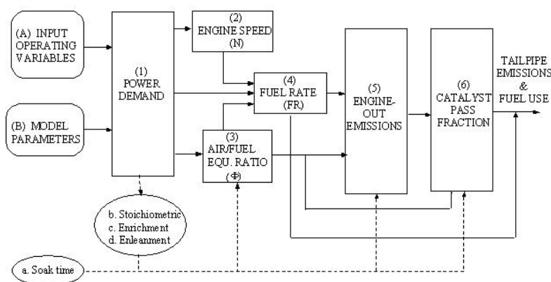
Figure 3.3: Structure of the CMEM [231] [Published with permission of the Center for Environmental Research and Technology].
