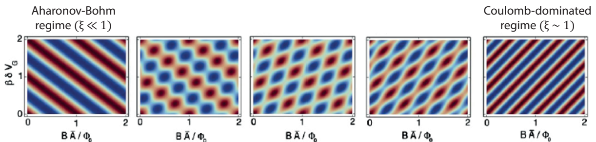
FIGURE 3.10: Transition from Aharonov-Bohm oscillations to Coulomb-dominated oscillations in QH FP interferometers. Evolution of the 2D pattern formed by the resistance oscillations in the magnetic field/gate voltage plane depending on the value of \xi . Pure AB oscillations ( \xi \ll 1 ) form lines with negative slopes while Coulomb-dominated oscillations ( \xi \sim 1 ) form lines with positive slopes. A transition exists between the two extreme regimes where both types of oscillations coexist. Intermediate regimes are characterized by 2D rhombic lattice patterns. Adapted from ref. [148].
