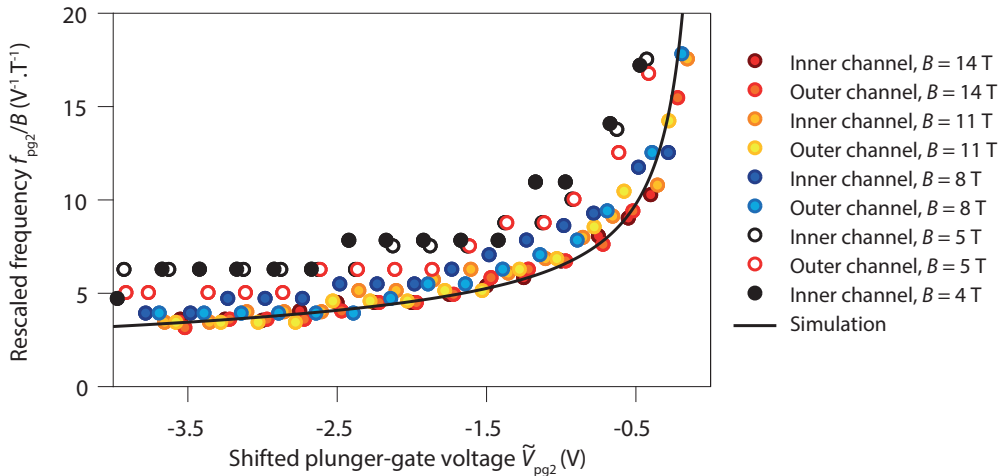
FIGURE 5.6: Magnetic field dependence of the frequency of gate-induced oscillations. Evolution of the main peak frequency f_{\text{pg}2} rescaled by the magnetic field B as a function of \tilde{V}_{\text{pg}2} , the plunger-gate voltage shifted with respect to the voltage that expels the interfering edge channel in several experiments. The data points for different interferometry experiments collapse onto a single curve, except for the low field data. The solid black line is an electrostatics simulation of the pn junction displacement with the plunger-gate voltage.
