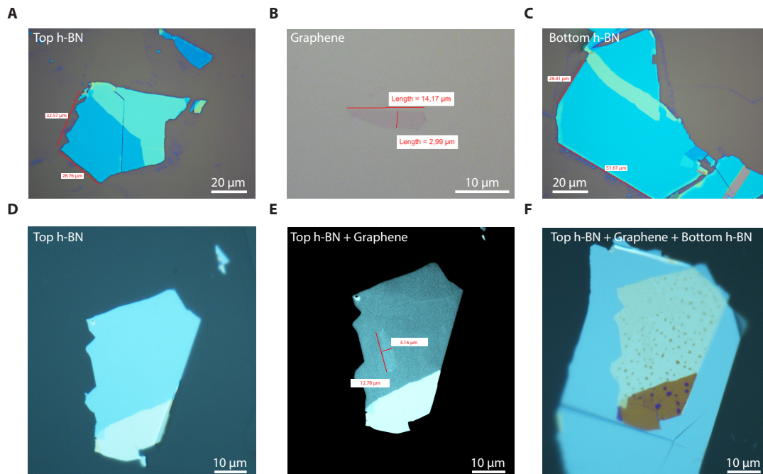
FIGURE 12.8: Assembling of a h-BN/graphene/h-BN stack. A, B, C, Optical images of the flakes used to make the heterostructure. D, E, F, Optical images of the heterostructure on the stamp after the successive pick-ups. The final heterostructure released on the substrate is shown in Fig 12.10
