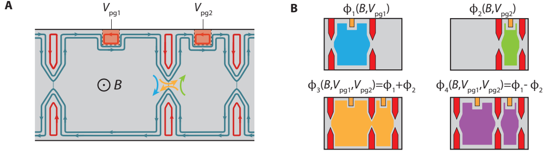
FIGURE 7.1: Double QH FP interferometry. A , Schematic of a graphene double FP interferometer in a configuration of partial backscattering of the inner edge channel. The central QPC can either reflect an incoming electron from the left cavity (blue arrow) or the right cavity (green arrow), or transmit coherently an electron from one cavity to the other (yellow arrows). In the latter case, the electrons pick up the Aharonov-Bohm phase given by the combined areas of the small and medium interferometers. In higher order processes, the electrons make multiple loops in the two cavities. B , Schematics of the cavities involved in the different interference processes in a double FP cavity. \phi_{1,2,3,4} are the corresponding Aharonov-Bohm phases, indicated with the magnetic field and plunger-gate voltages that modulate them.
