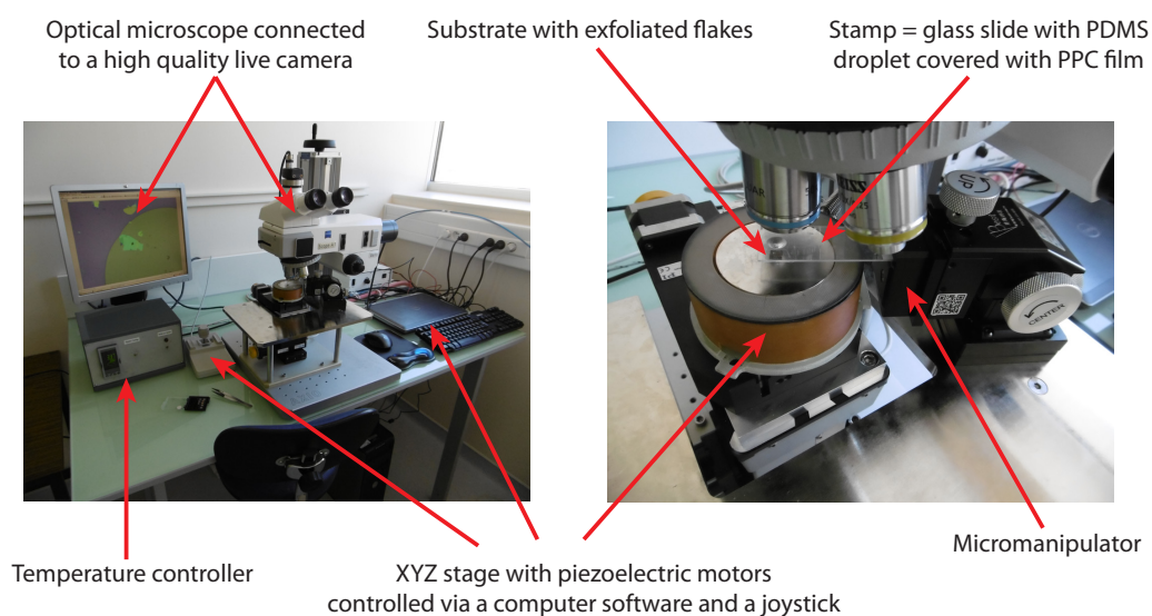
FIGURE 12.6: Transfer microscope. Photos of the transfer set-up used to assemble Van der Waals heterostructures. The set up is composed of a high quality optical microscope, a XYZ stage controlled by piezoelectric motors and a micromanipulator where the stamp is placed. It enables to pick-up and stack flakes with a precision of about one micron on the alignment of the flakes.
