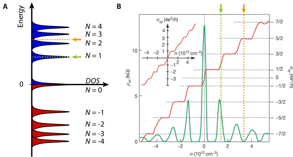
FIGURE 1.7: Graphene QH plateaus. A , Density of states (DOS) of graphene LLs. Each LL can be represented as a peak in the DOS with finite width. B , Typical signatures of graphene QH effect in six-terminal Hall bar geometry. When the Fermi level lies in the tail of a LL peak (orange dashed line), there is no backscattering in the sample and the transport is quantized. When the Fermi level lies in the middle of a LL (green dashed line), there is some backscattering in the sample and the transport is no longer quantized. Adapted from ref. [8].
