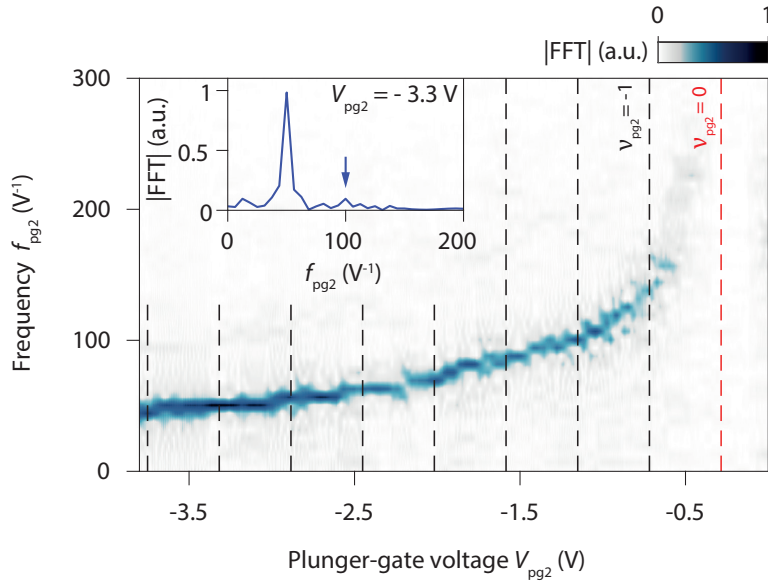
FIGURE 5.3: Fourier transform of gate-induced oscillations. Evolution of the Fourier amplitude of the resistance oscillations shown in Fig. 5.1.C with the plunger-gate voltage V_{pg2} and the plunger-gate-voltage frequency f_{pg2} . The vertical dashed lines indicate when the filling factor beneath the plunger gate \nu_{pg2} is an integer. Oscillations with a small voltage period emerge at V_{pg2} \simeq -0.3 V corresponding to the CNP below the plunger gate. Inset: Linecut at V_{pg2} = -3.3 V evidencing the presence of a second harmonic (blue arrow).
