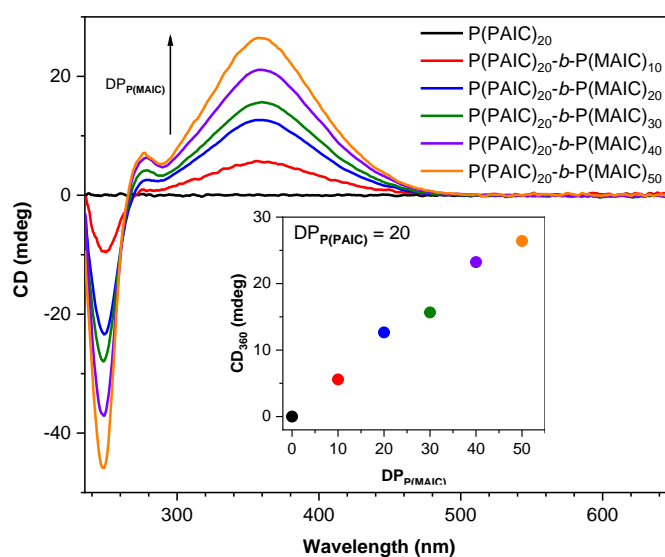
Figure A2.23. CD (THF, 0.5 \text{ mg}\cdot\text{mL}^{-1} ) spectra of PAIC monomer and \text{P(PAIC)}_{20}\text{-}b\text{-P(MAIC)}_x copolymers ( x = 0, 10, 20, 30, 40, 50 ). Inset : CD signal at \lambda = 360 \text{ nm} plotted vs \text{DP}_{\text{P(MAIC)}} .
