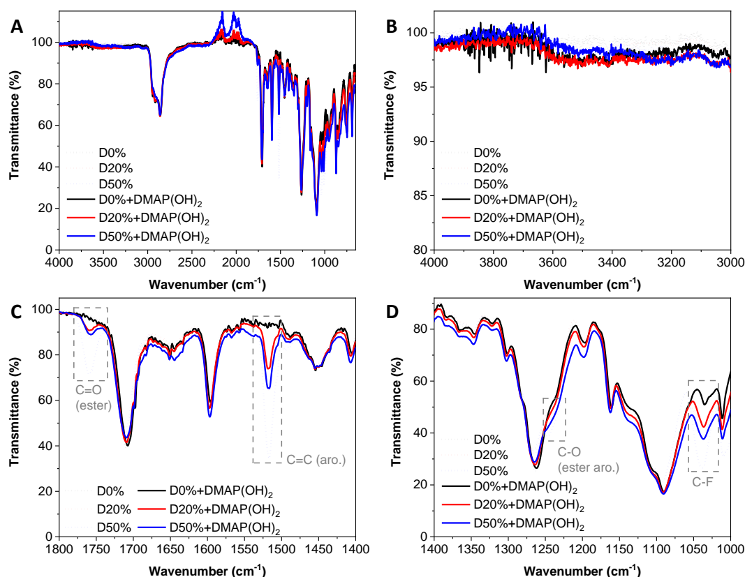
Figure 5.17. FT-IR spectra of the D0% (black), D20% (red) and D50% (blue) copolymers unreacted (dotted line) and reacted with \text{DMAP}(\text{OH})_2 (solid line). (A) Full spectrum. (B) Zoom in the 4000\text{--}3000\text{ cm}^{-1} region. (C) Zoom in the 1800\text{--}1400\text{ cm}^{-1} region. (D) Zoom in the 1400\text{--}1000\text{ cm}^{-1} region.
