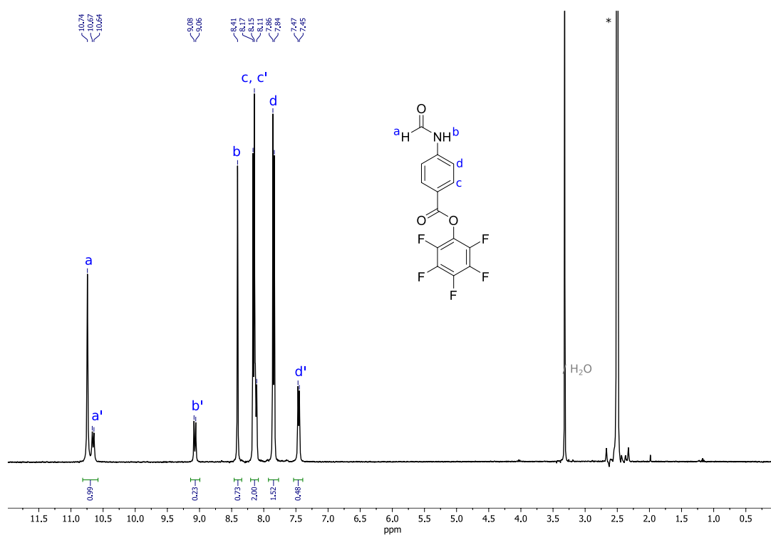
Figure 7.41. 1 H NMR of pentafluorophenyl 4-formamidobenzoate in (CD 3 ) 2 SO (400 MHz, 298 K)
