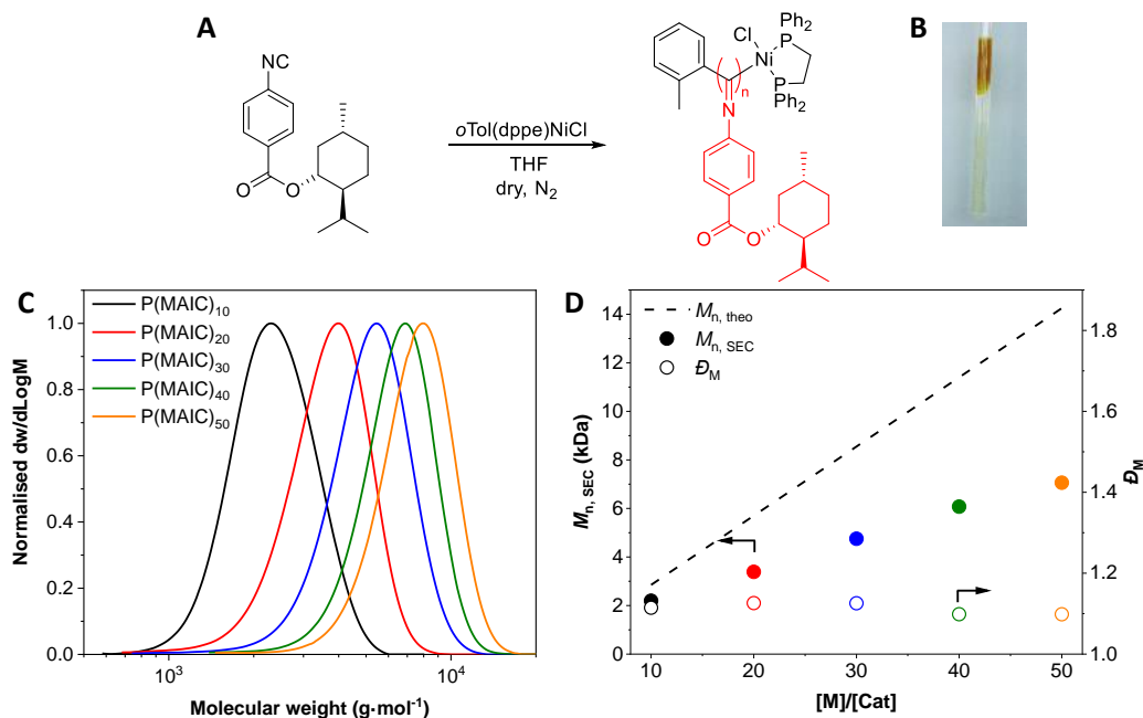
Figure 2.3. (A) Scheme of the homopolymerisation of MAIC. (B) The NMR tube contains P(MAIC) \text{DP}_{\text{MAIC}} = 10 in DMSO which shows the insolubility of the homopolymer in DMSO. (C) Normalised SEC RI molecular weight distributions (THF + 2% v/v \text{NEt}_3 , 40 °C, PS standards) of the different DPs of P(MAIC) y homopolymer. (D) M_{n,\text{SEC}} (filled circles) and D_M (hollow circles) as a function of monomer over catalyst ratio.
