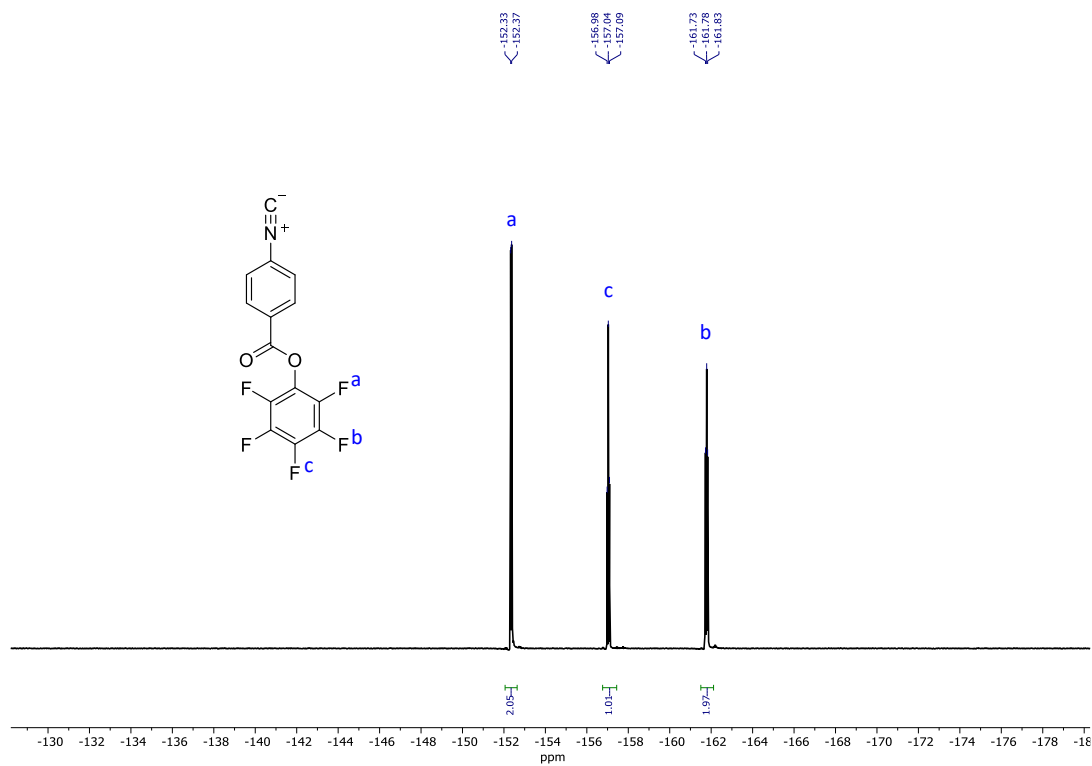
Figure 7.46. 19 F NMR of FAIC in CDCl 3 (377 MHz, 298 K)
