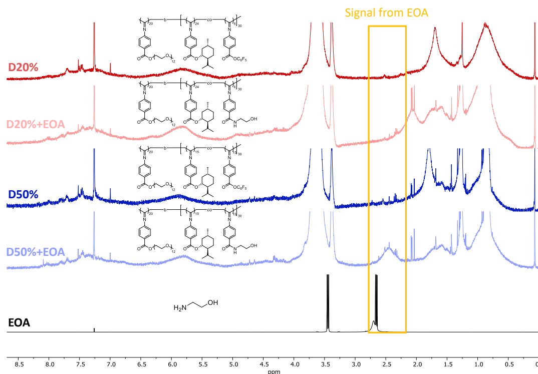
Figure 3.12. 1 H NMR of D20%, D20%+EOA, D50%, D50%+EOA and EOA in CDCl 3 (400 MHz, 298 K).
