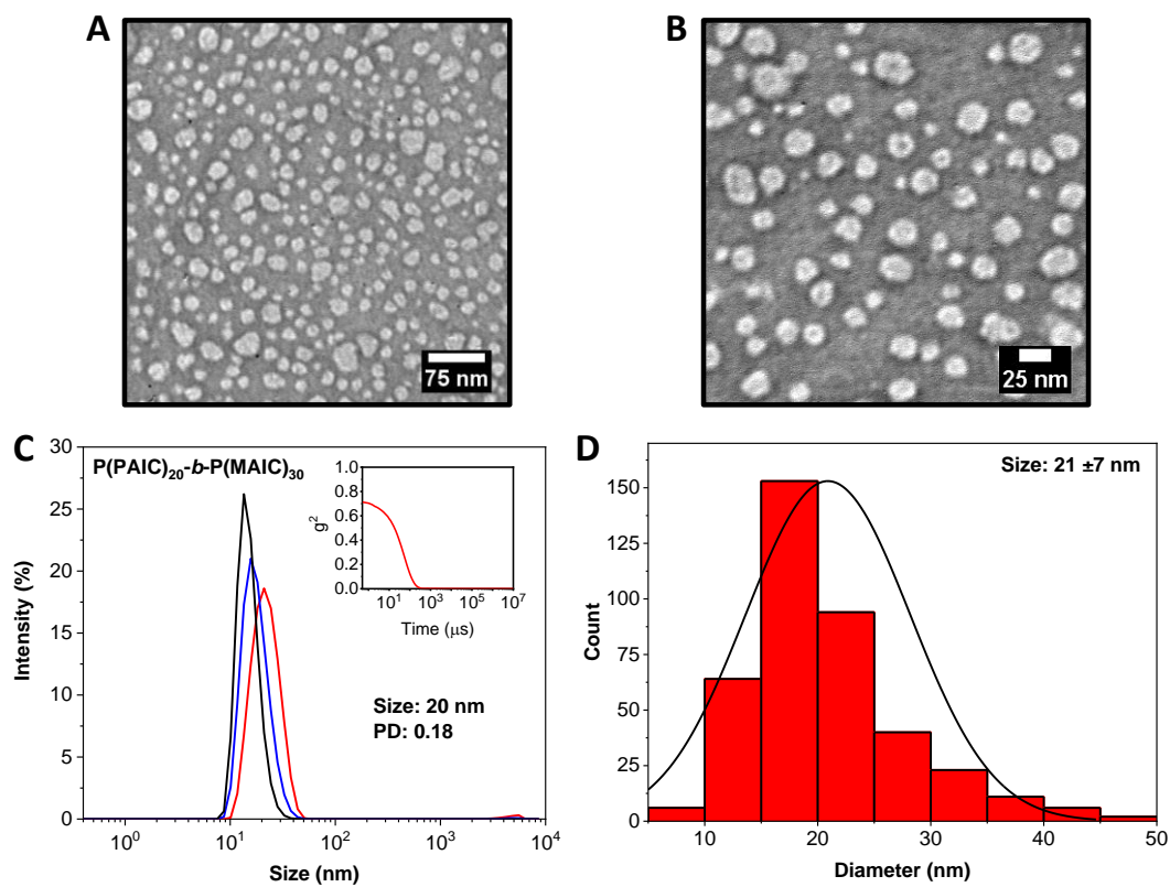
Figure A2.30. (A and B) Dry-state TEM images of the sphere morphology obtained from NiCCo-PISA of P(\text{PAIC})_{20}\text{-}b\text{-}P(\text{MAIC})_{30} . (C) Intensity-weighted size distributions of P(\text{PAIC})_{20}\text{-}b\text{-}P(\text{MAIC})_{30} in DMSO obtained by DLS. Inset : DLS autocorrelation function. (D) Histogram of spherical particles' size distribution measured from particle analysis of TEM images.
