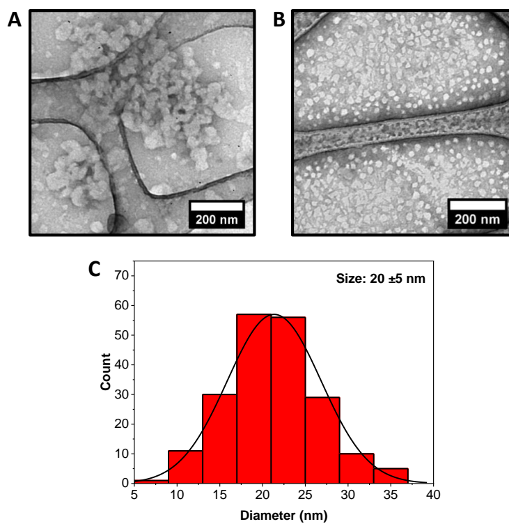
Figure A 2.32. (A and B) Dry-state TEM images of the mixed sphere and worm morphologies obtained from NiCCo-PISA of P(PAIC) 20 - b -P(MAIC) 50 . (C) Histogram of spherical particles' size distribution measured from particle analysis of TEM images.
