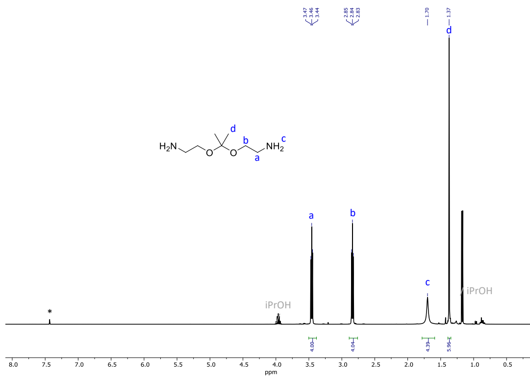
Figure 7.52. 1 H NMR of AEE in \text{CDCl}_3 (400 MHz, 298 K)
