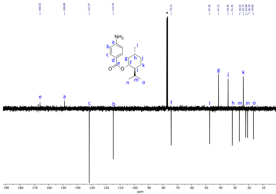
Figure 7.4. ^{13}\text{C} NMR spectrum of menthyl 4-aminobenzoate in \text{CDCl}_3 (100 MHz, 298 K).
