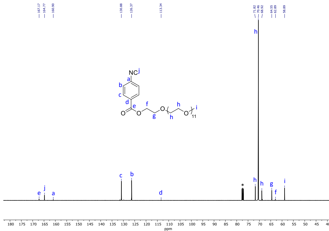
Figure 7.23. ^{13}\text{C} NMR spectrum of PAIC in \text{CDCl}_3 (100 MHz, 298 K).
