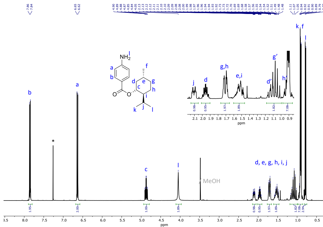
Figure 7.3. ^1\text{H} NMR spectrum of menthyl 4-aminobenzoate in \text{CDCl}_3 (400 MHz, 298 K).
