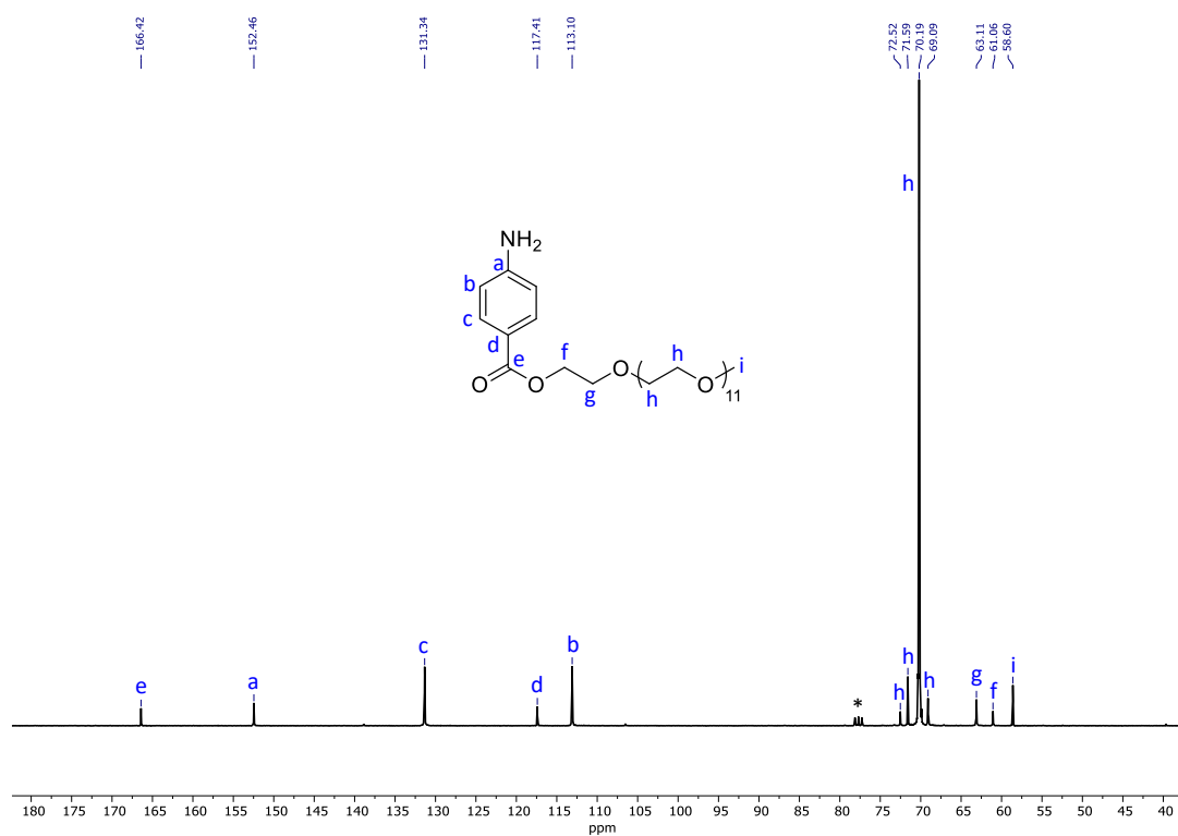
Figure 7.15. ^{13}\text{C} NMR spectrum of mPEG-Ar-NH 2 in CDCl 3 (100 MHz, 298 K).
