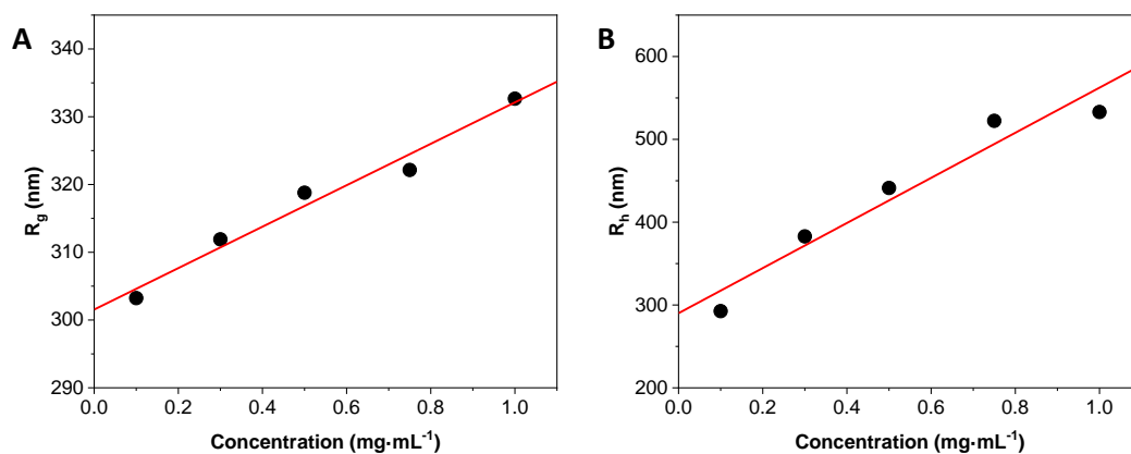
Figure 2.12. (A) Multi-angle SLS with R_g as a function of concentration and its linear regression where the intercept is R_g at \rightarrow 0 . (B) Multi-angle DLS with R_h as a function of concentration and its linear regression where the intercept is R_h at c \rightarrow 0 .
