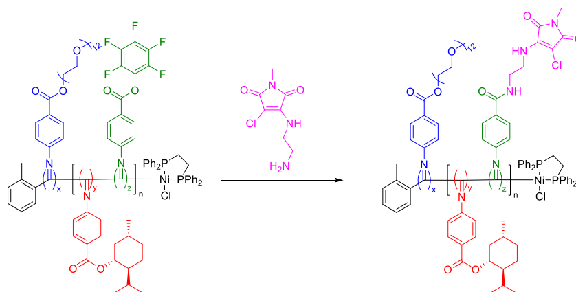
Scheme 3.8. Substitution of P(\text{PAIC})_x\text{-}b\text{-}P(\text{MAIC})_y\text{-}co\text{-}P(\text{FAIC})_z with a aminochloromaleimide (ACM).
