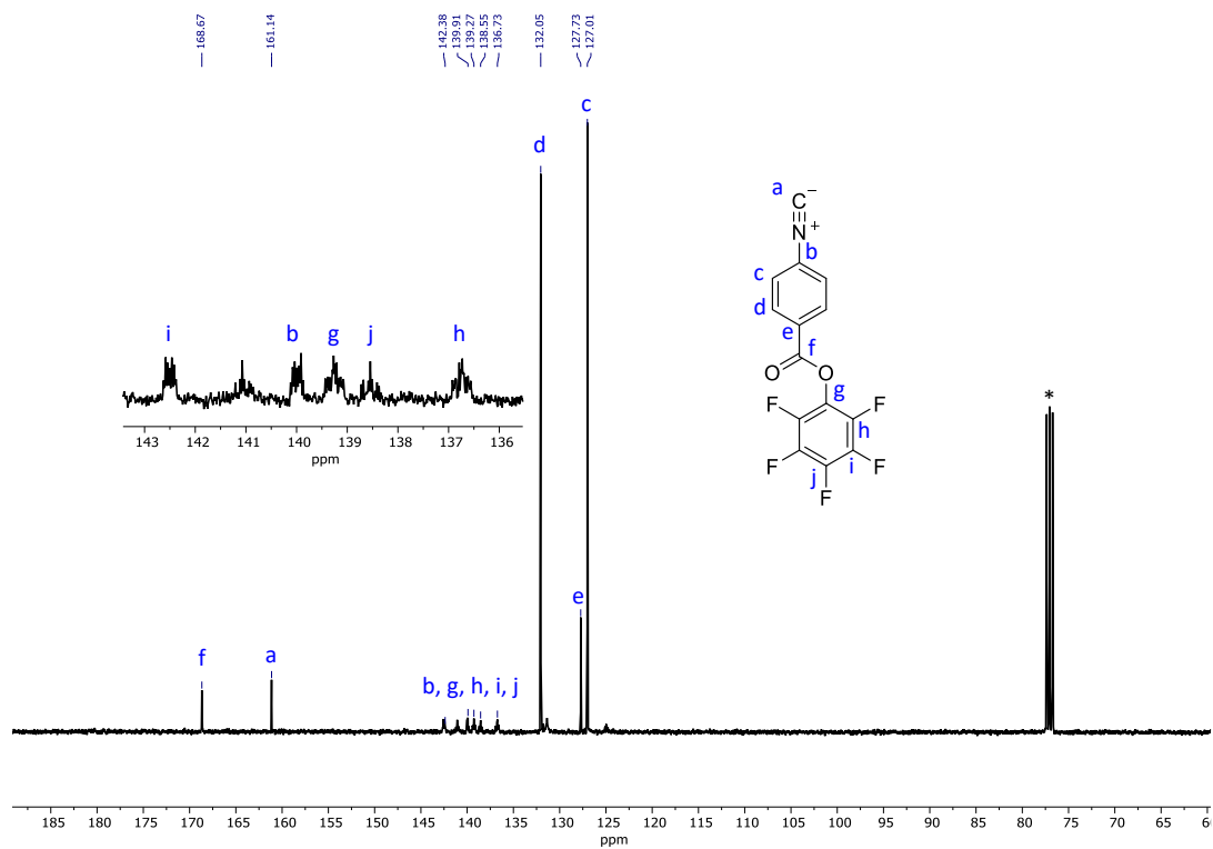
Figure 7.45. 13 C NMR of FAIC in CDCl 3 (100 MHz, 298 K)
