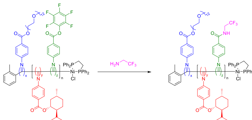
Scheme 3.7. Substitution of P(PAIC) x -b-(P(MAIC) y -co-P(FAIC) z ) n with trifluoroethylamine (TFEA).
