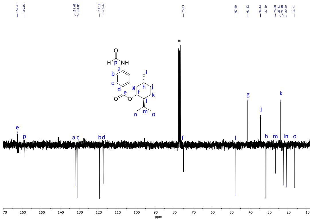
Figure 7.6. 13 C NMR spectrum of menthyl 4-formamidobenzoate in CDCl 3 (100 MHz, 298 K).
