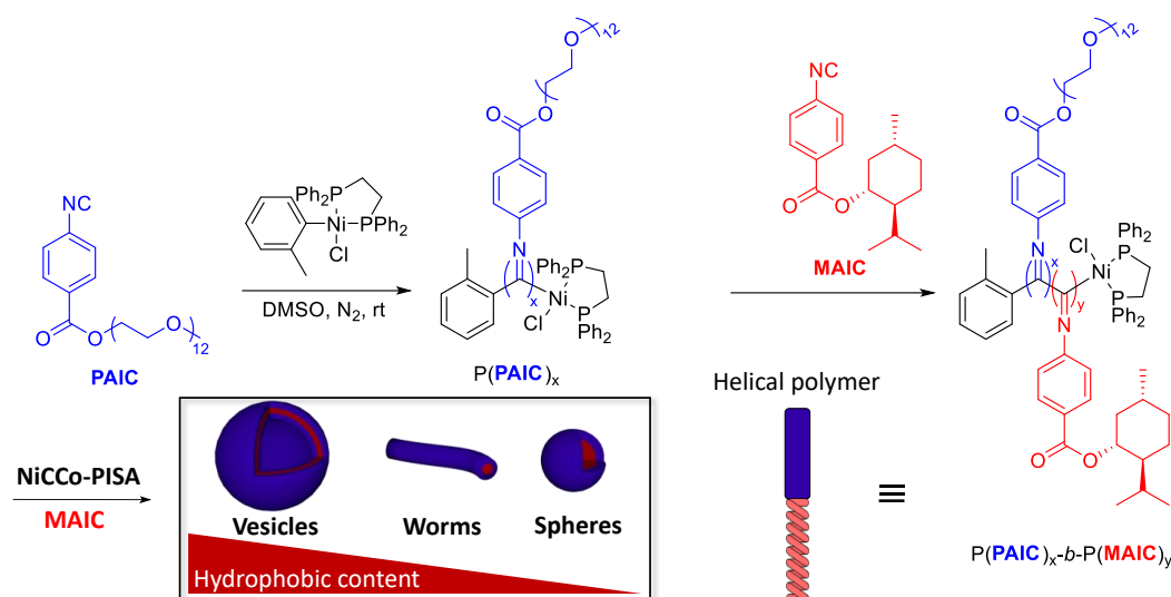
Scheme 2.2. Synthetic route followed for the preparation of diblock copolymers via NiCCo-PISA of P(\text{PAIC})_x\text{-}b\text{-}P(\text{MAIC})_y .
