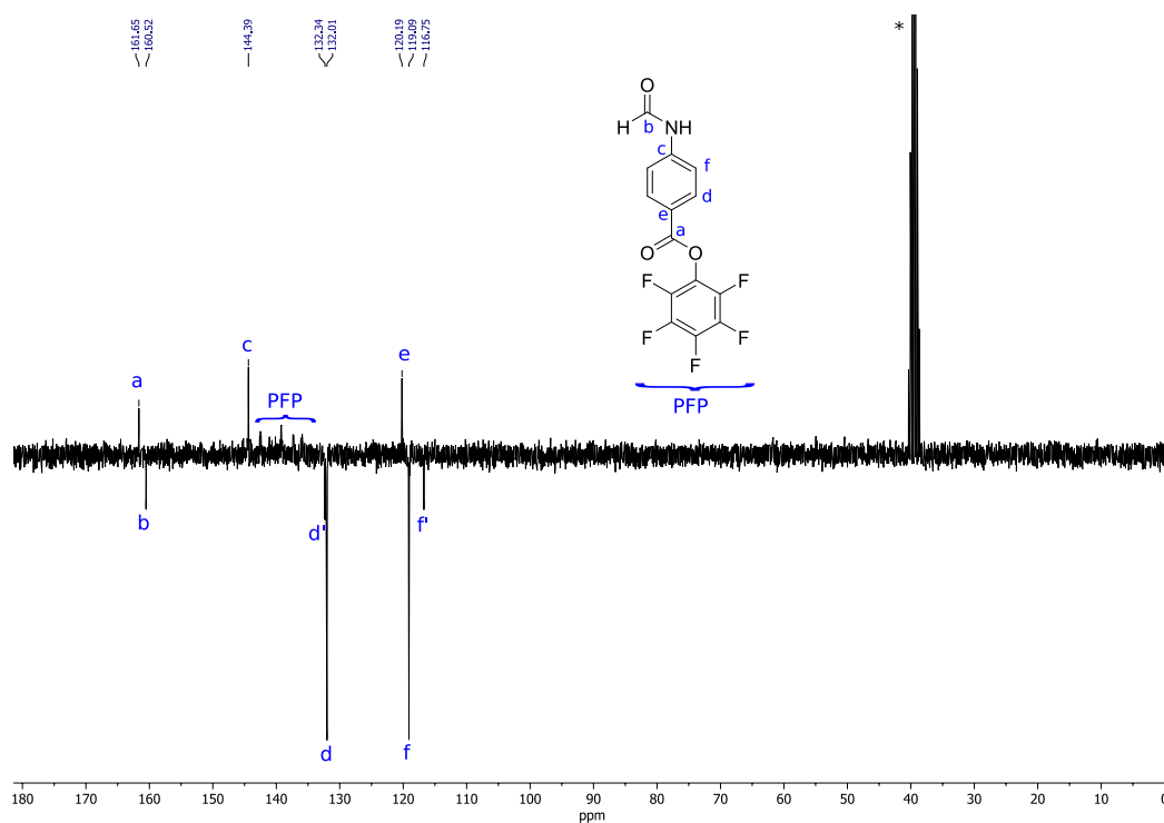
Figure 7.42. 13 C NMR of pentafluorophenyl 4-formamidobenzoate in (CD 3 ) 2 SO (100 MHz, 298 K)
