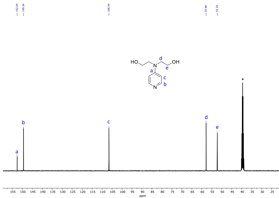
Figure 7.59. ^{13}\text{C} NMR of DMAP(OH) 2 in (CD 3 ) 2 SO (100 MHz, 298 K)
