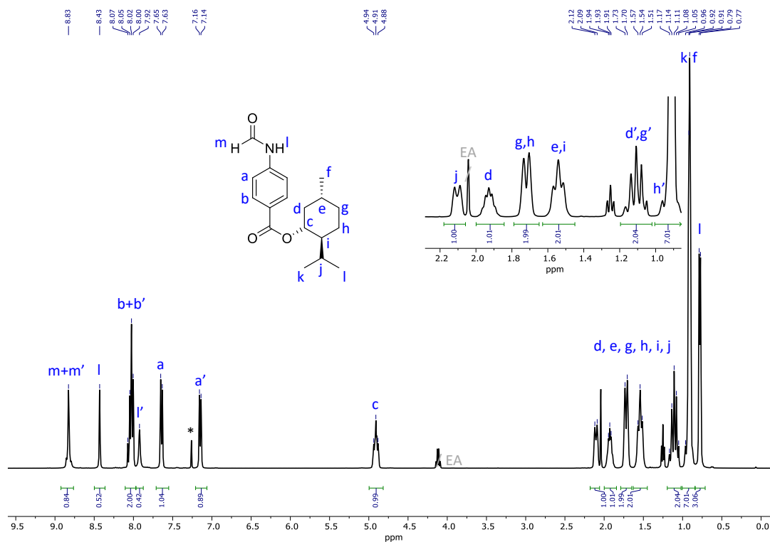
Figure 7.5. 1 H NMR spectrum of menthyl 4-formamidobenzoate in CDCl 3 (300 MHz, 298 K).
