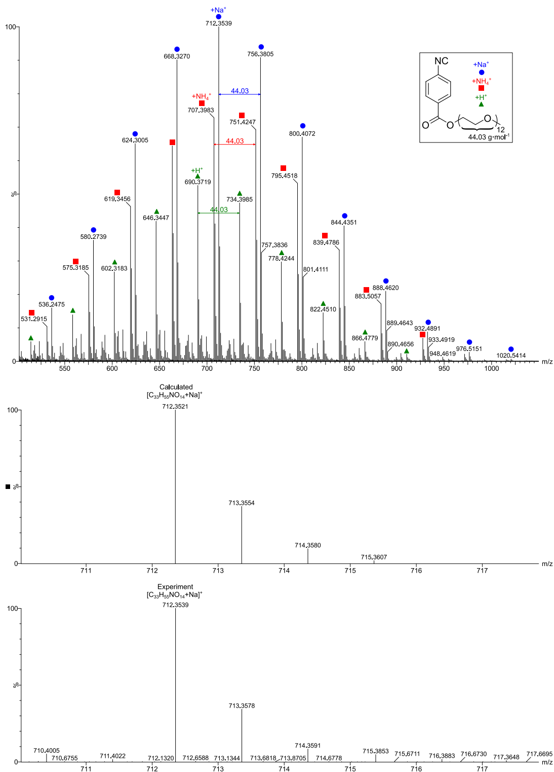
Figure 7.24. Top: Mass spectra of PAIC collected by ESI-MS. Top: Expanded spectrum (500-1000 m/z ) with \text{Na}^+ (blue circles), \text{NH}_4^+ (red squares) and \text{H}^+ (green triangles) adduct of the product PAIC. Bottom: Calculated vs experimental m/z value for \text{PAIC} + \text{Na}^+ adduct.
