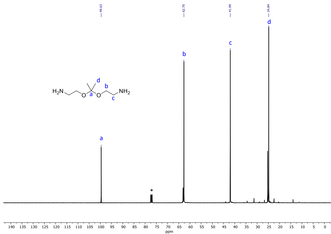
Figure 7.53. 13 C NMR of AEE in \text{CDCl}_3 (100 MHz, 298 K)
