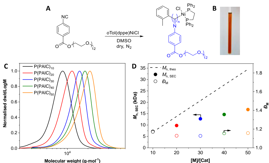
Figure 2.2. (A) Scheme of the homopolymerisation of PAIC. (B) The NMR tube contains P(PAIC) \text{DP}_{\text{PAIC}} = 10 in DMSO which shows the solubility of the homopolymer in DMSO. (C) Normalised SEC RI molecular weight distributions (THF + 2% v/v \text{NEt}_3 , 40 °C, PS standards) of the different DPs of P(PAIC) x homopolymer. (D) M_{n,\text{SEC}} (filled circles) and D_M (hollow circles) as a function of monomer over catalyst ratio.
