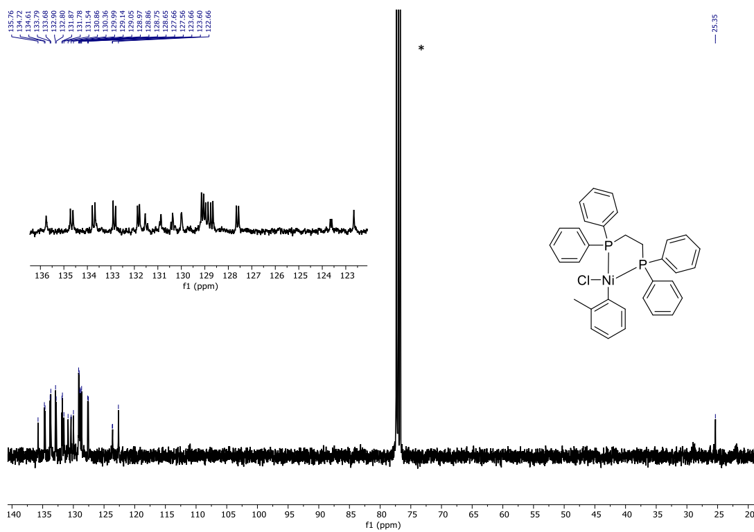
Figure 7.31. 13 C NMR spectrum of o -tol(dppe)NiCl 2 in CDCl 3 (100 MHz, 298 K).
