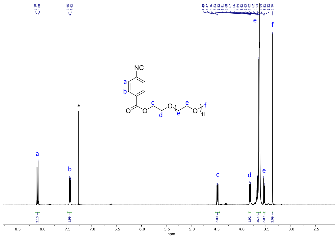
Figure 7.22. ^1\text{H} NMR spectrum of PAIC in \text{CDCl}_3 (400 MHz, 298 K).
