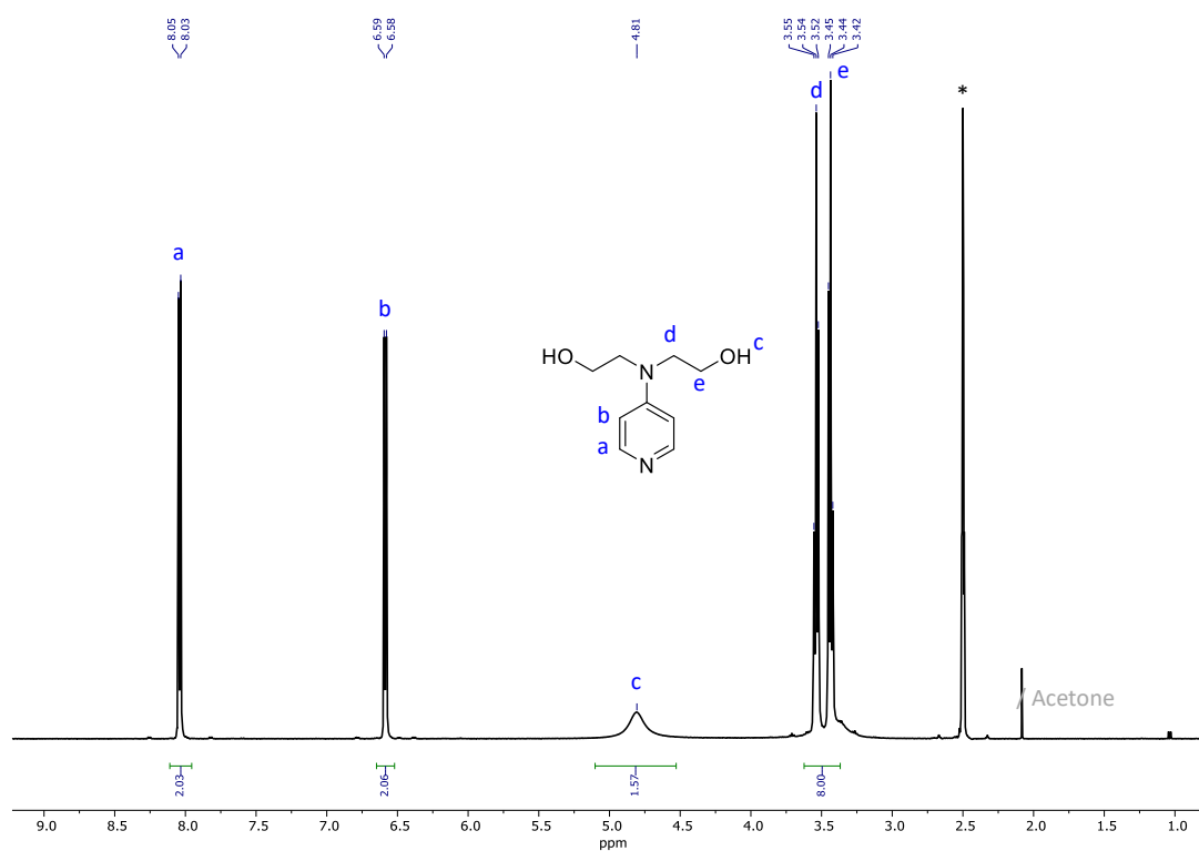
Figure 7.58. ^1\text{H} NMR of DMAP(OH) 2 in (CD 3 ) 2 SO (400 MHz, 298 K)
