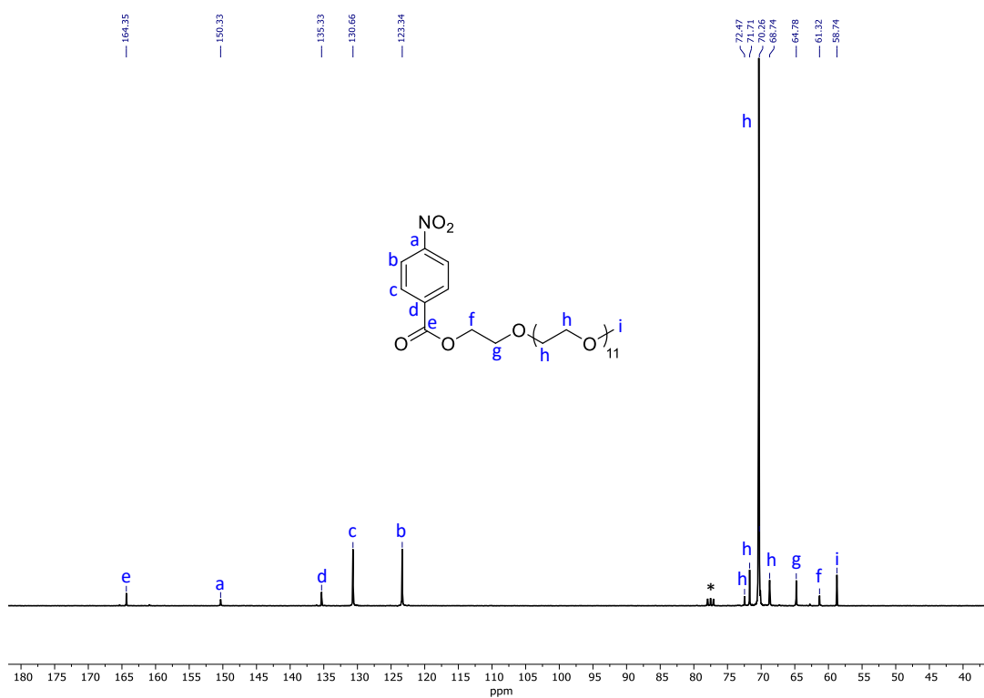
Figure 7.11. ^{13}\text{C} NMR spectrum of mPEG-Ar-NO 2 in CDCl 3 (100 MHz, 298 K)
