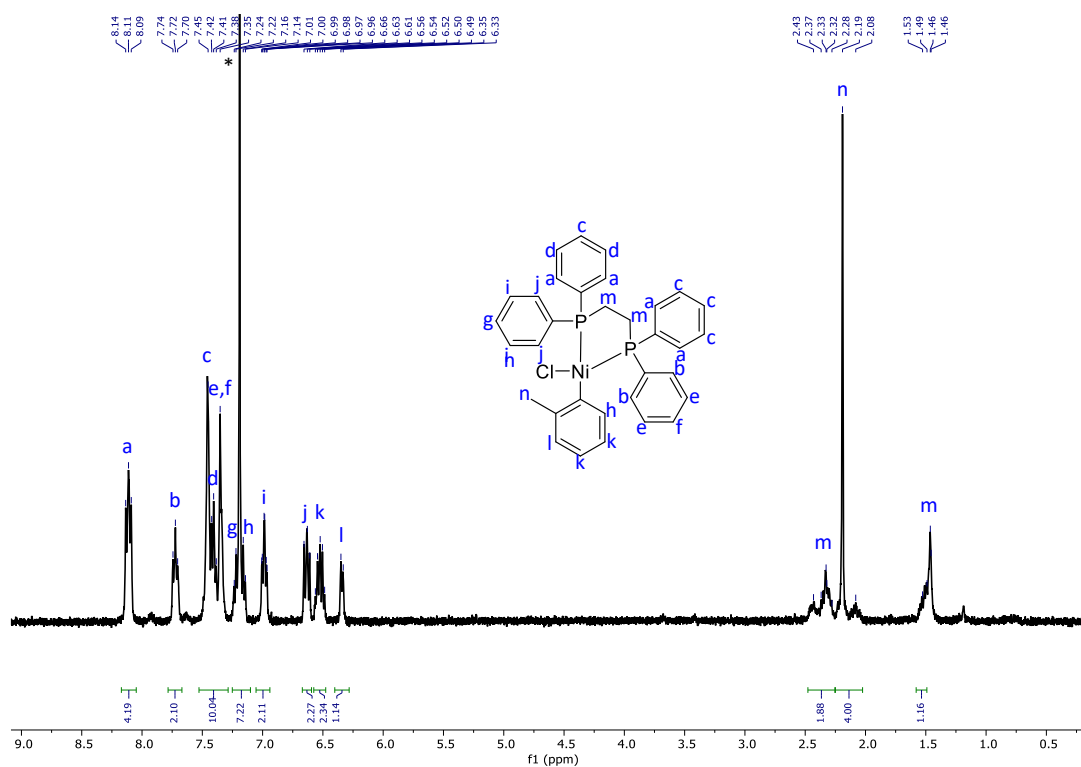
Figure 7.30. 1 H NMR spectrum of o -tol(dppe)NiCl 2 in CDCl 3 (400 MHz, 298 K).
