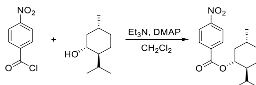
Scheme 7.1. Menthyl 4-nitrobenzoate synthesis.
