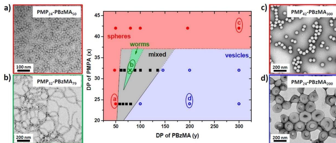
Figure 1.11. Phase diagram constructed by varying the solvophobic (abscissa) and solvophilic (ordinate) block length for poly(methacryloyloxymethyl dimethylphosphonate) _x - b -poly(benzyl methacrylate) _y diblock copolymer nano-objects: spherical micelles (red), worm-like micelles (green), polymersomes (blue) and mixed morphologies (grey). Reproduced from the work of Hanisch et al. published in ACS, Macromolecules . 157
