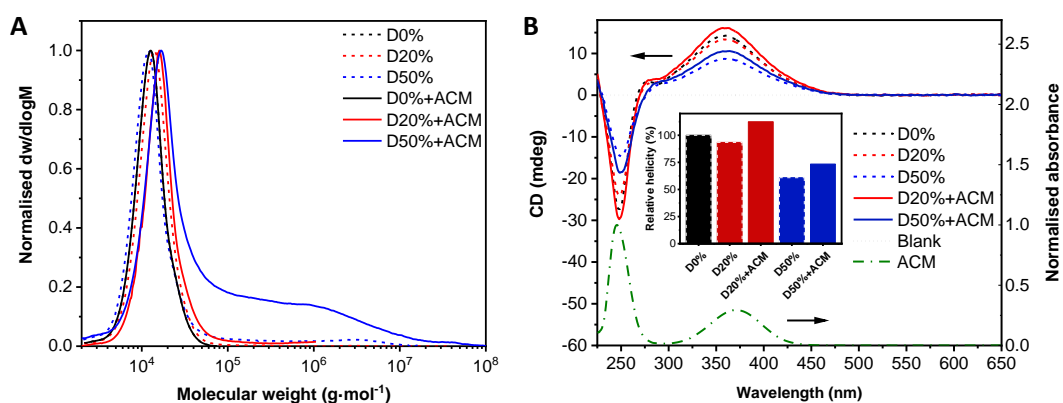
Figure 3.20. (A) Normalised SEC RI molecular weight distributions (THF + 2% v/v NEt 3 , 40 °C, PS standards) and B) CD (THF, 0.5 mg·mL -1 ) spectra of D0%, D0%+ACM, D20%, D20%+ACM, D50% and D50%+ACM. The inset shows the helicity (CD at \lambda = 360 nm) of the copolymers compared to D0%.
