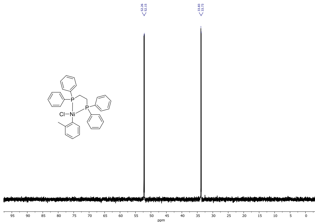
Figure 7.32. ^{31}\text{P} NMR spectrum of o -tol(dppe)NiCl 2 in CDCl 3 (100 MHz, 298 K).
