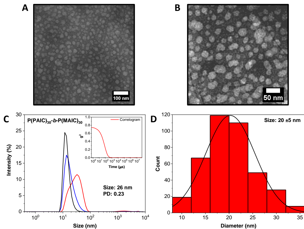
Figure A2.34. (A and B) Dry-state TEM images of the sphere morphology obtained from NiCCo-PISA of P(PAIC) 30 - b -P(MAIC) 30 . (C) Intensity-weighted size distributions of P(PAIC) 30 - b -P(MAIC) 30 in DMSO obtained by DLS. Inset : DLS autocorrelation function. (D) Histogram of spherical particles' size distribution measured from particle analysis of TEM images.
