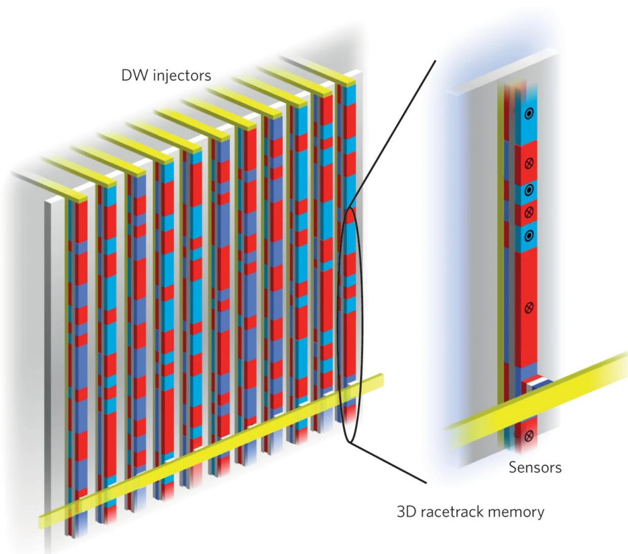
Figure 1.1: Three dimensional technology: Racetrack Memory 4.0. Red and blue regions represent areas that are oppositely magnetized. Adapted from [4].
