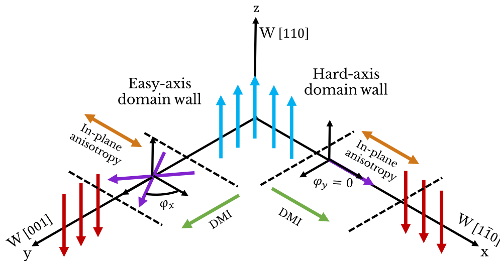
Figure 5.3: Micromagnetic W(110) framework framework. Sketch of the possible configurations for domain walls oriented along the in-plane easy axis and the in-plane hard axis. Red, blue and purple arrows: magnetisation direction. Orange arrows: effective in-plane anisotropy field direction. Green arrows: effective DMI field direction. Adapted from [ 156 ].
