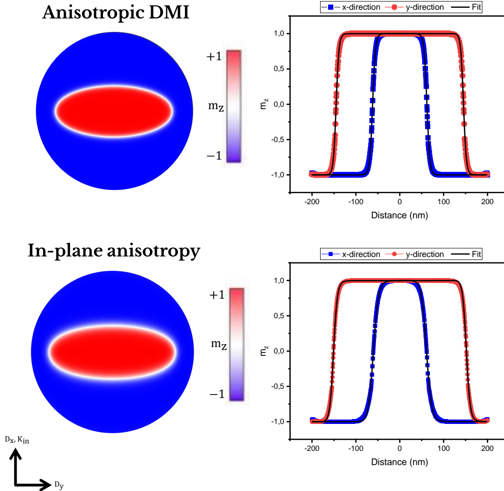
Figure 5.12: Micromagnetic stabilised elliptical skyrmion. Due due to an anisotropic DMI: ( D_y/D_x = 0.75 ) with D_x=1.5 \text{ kJ/m}^3 and K_{\text{in}}=0 \text{ mJ/m}^2 , or an in-plane anisotropy ( D_y/D_x = 1 ) with D_x=1.5 \text{ mJ/m}^2 and K_{\text{in}} = 136 \text{ kJ/m}^3 . A = 16 \text{ pJ/m} , M_s = 1.15 \text{ MA/m} , K_u = 1031 \text{ kJ/m}^3 are used for the two cases.
