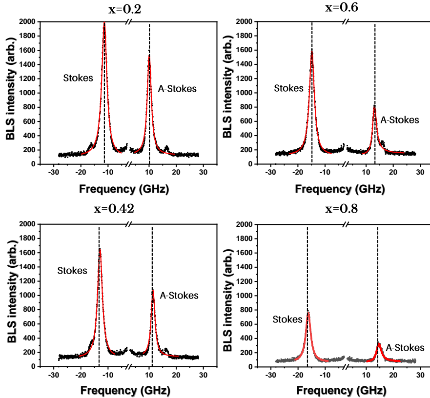
Figure 4.14: Brillouin light scattering spectrum for the \text{Au}_{1-x}\text{Pt}_x/\text{Co}(0.78\text{nm})/\text{W}(110) stack as function of the Au-to-Pt content x .
