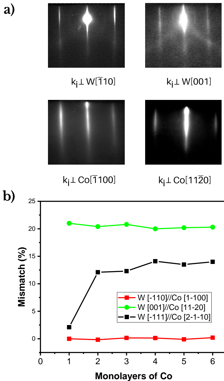
Figure 4.5: hcp-Co(0001)/bcc-W(110) reflection high energy electron diffraction along the two main in-plane directions. a) reflection high energy electron diffraction patterns with the incoming wavevector perpendicular to the two main in-plane directions of Co(0001) and W(110) b) Cobalt mismatch as function of the number of Co monolayers.
