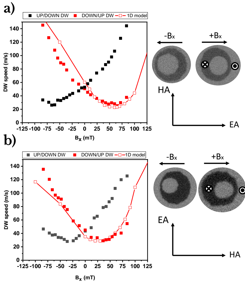
Figure 4.28: Field-driven domain wall motion for Au/Co(0.6nm)/W(110) under an static in-plane field. Black squares: Up/down domain wall. Red squares: Down/up domain wall. Empty red squares: one-dimensional model. The domain walls are driven by 20 ns long pulses B_z of 60 mT, under an static in-plane field applied along the a) easy and b) hard in-plane axis. In the differential Kerr images, the dark contrast represents the displacement of the domain walls during the application of the out-of-plane magnetic field pulse.
