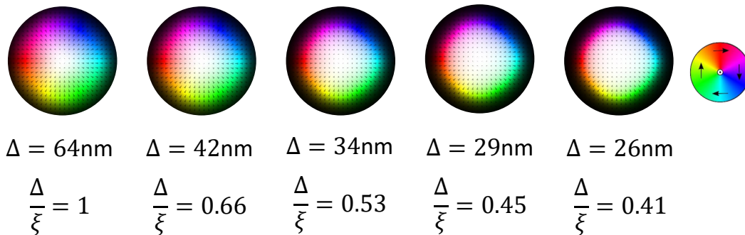
Figure 5.21: Stabilised magnetic states for a fix spin cycloid length for different domain wall parameters. Black means magnetisation into the plane and white means magnetisation out of the plane. The wheel represents the color code for in-plane magnetisation direction, red meaning magnetisation along positive x-direction and green meaning magnetisation along positive y direction. The spin cycloid length has been fixed to \zeta = 64 nm.
