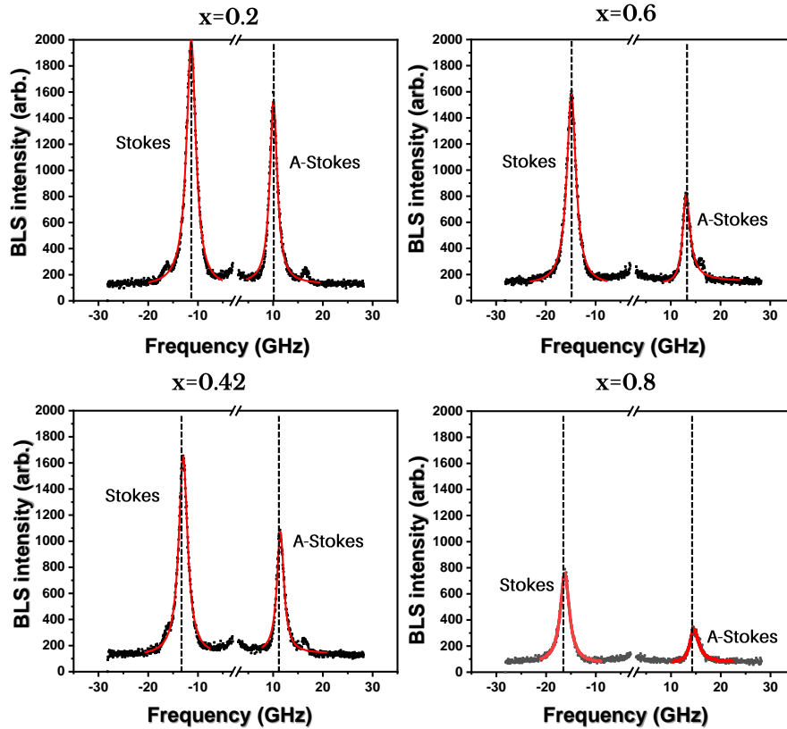
Figure 4.14: Brillouin light scattering spectrum for the Au 1-x Pt x /Co(0.78nm)/W(110) stack as function of the Au-to-Pt content x .
