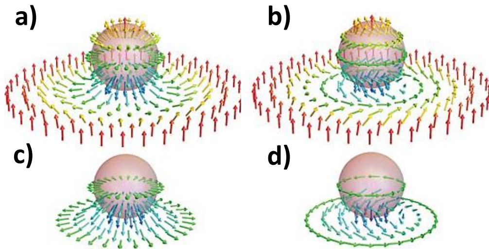
Figure 3.10: Bloch and Néel-type skyrmions and merons in the real space and their stereographical projection a) A Néel-type skyrmion in a 2D space and its stereographical projection. Note that the unit sphere is covered once, leading to Q = 1 . b) A Bloch-type skyrmion in a 2D space and its stereographical projection. Note that the unit sphere is covered once, leading to Q = 1 . Configurations a) and b) are topologically equivalent. c) Néel-type meron, often also described as a radial vortex, corresponds to half a skyrmion which is evident upon stereographic projection. d) A Bloch-type meron is topologically equivalent to the hedgehog-type meron shown in c) . Adapted from [90].
