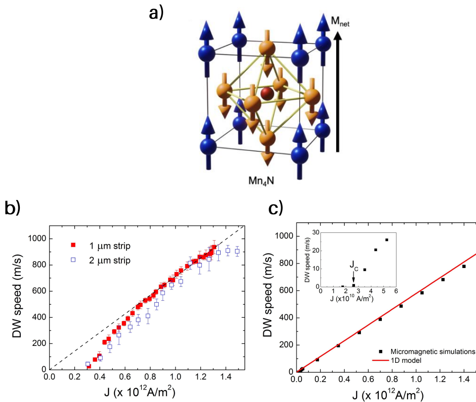
Figure 3.9: Manganite Nitride spin-transfer torque-domain wall motion. a) Crystal structure of \text{Mn}_4\text{N} . b) Experimental measurements of domain walls driven by STT for two different stripe widths. c) Micromagnetic simulations (dots) and 1D model (solid red line).
