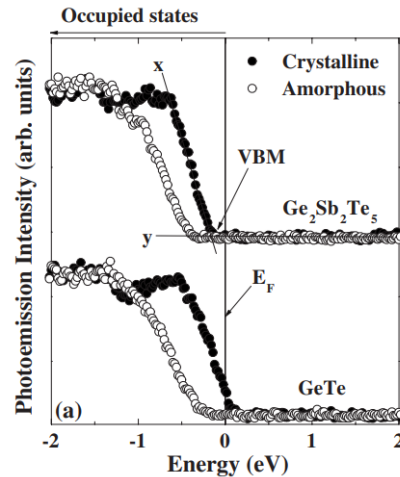
Fig. 1.7. HXPES spectra for GST (top) and GeTe (bottom) in the amorphous and crystalline phases [21], highlighting that the Valence Band Minimum (VBM) is closer to the Fermi level (Energy = 0 eV) for crystalline phase with respect to the amorphous
