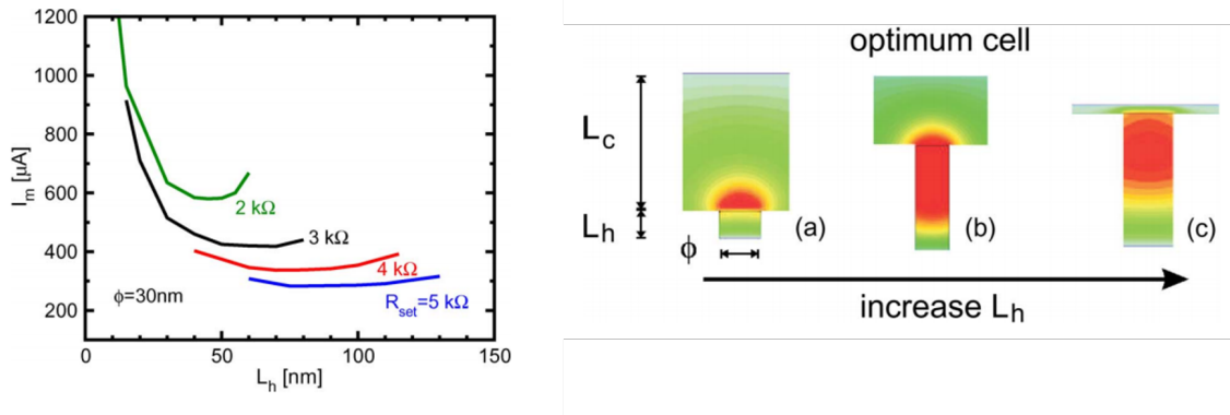
Fig. 2.3. left) Melting current ( I_m ) as a function of the heater length ( L_h ) for a fixed heater diameter \phi = 30 nm at different SET resistances obtained by tuning the phase-change layer thickness ( L_c ). right) Simulated temperature distributions in mushroom-type PCM cells for different non-isotropic scaling conditions.
