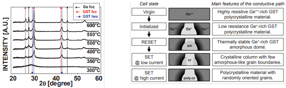
Fig. 1.19. X-ray diffraction (XRD) spectra of GST+Ge45% film after annealing at different temperatures, showing the phase separation of Ge and GST. Schematic of the composition and shape of the active volume during the programming of Ge-rich GST. [41].
