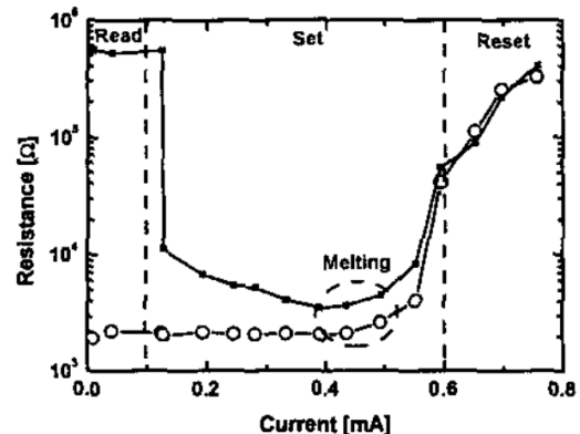
Fig. 1.14. Resistance as a function of current for a PCM device in SET state (empty circles) and RESET state (filled black squares) [32].
