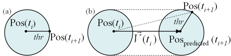
Figure II.8: Point-based (a) vs. vector-based (b) update policies with accuracy threshold thr
