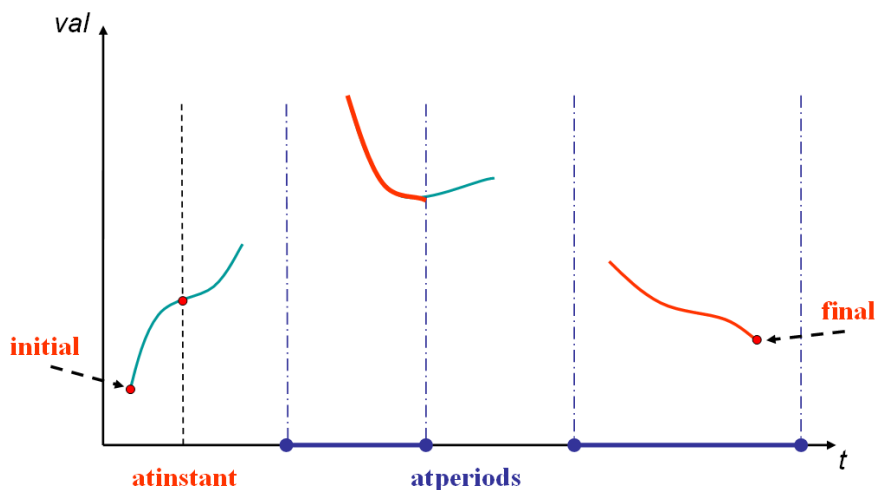
Figure II.11: Examples of interactions with time domain values
