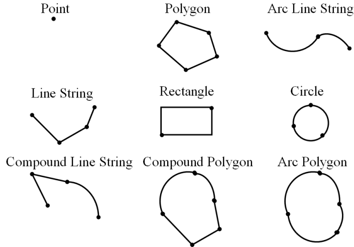
Figure II.4: Geometric types in Oracle Spatial
