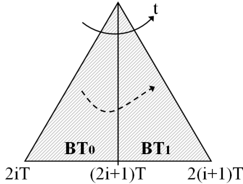
Figure IV.15: The ST^2B -tree rotates with time
