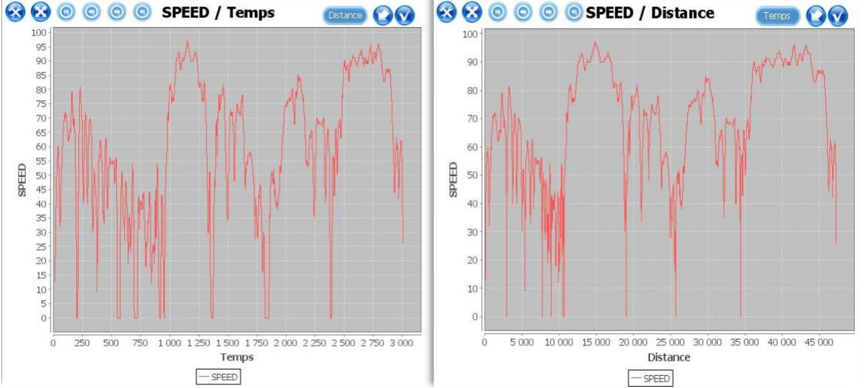
Figure VI.10: Variation of a measure in time or by distance
