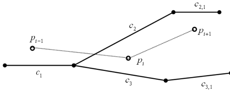
Figure VI.7: Incremental map-matching example with look-ahead
