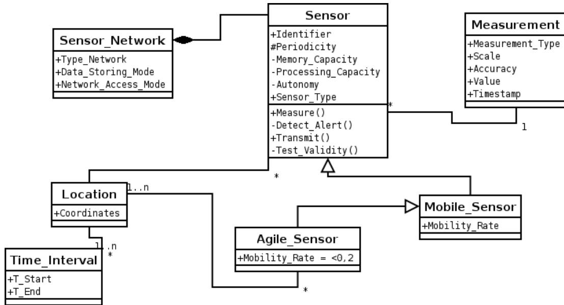
Figure III.2: Data model for measures and sensors [33]
