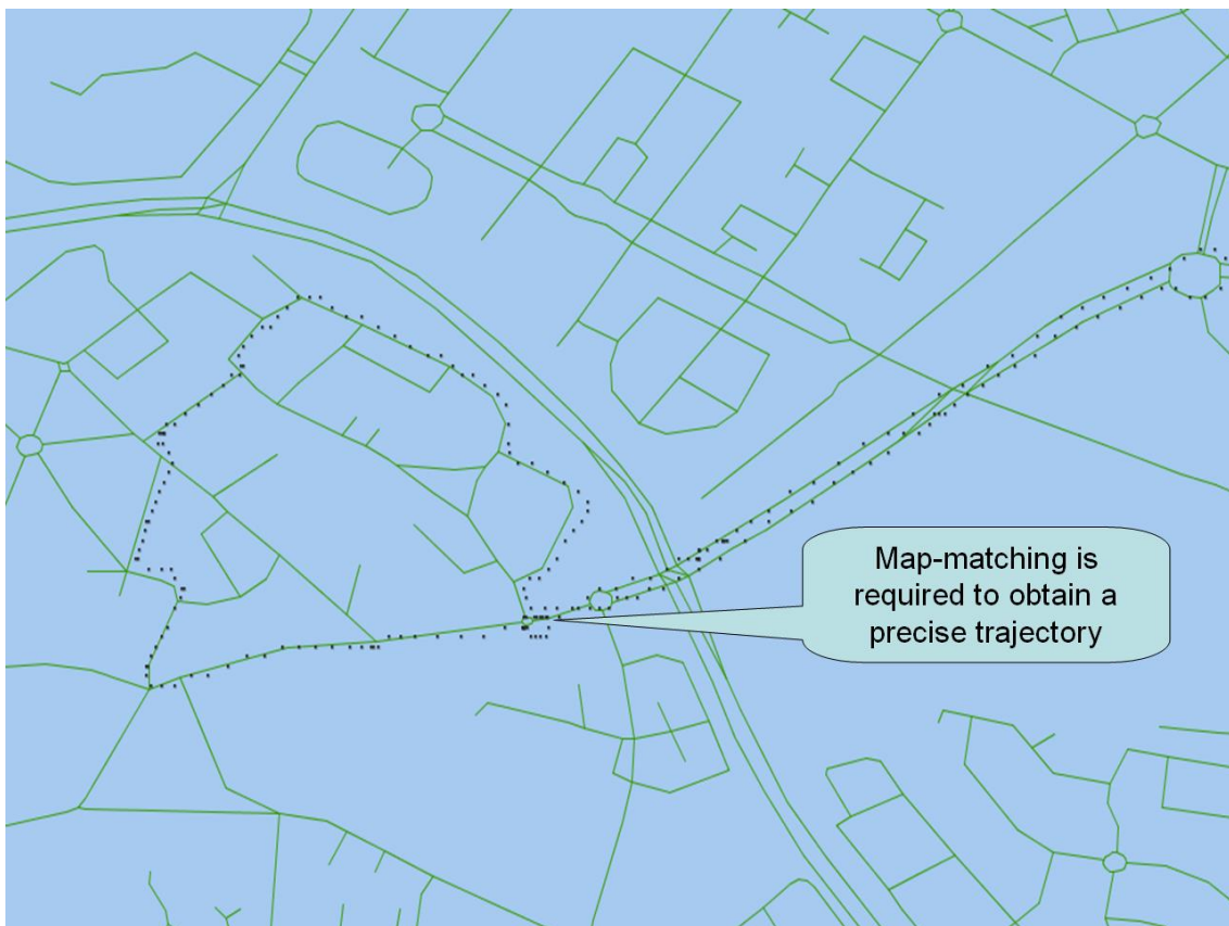
Figure VI.3: The GPS recordings and the maps are error prone
