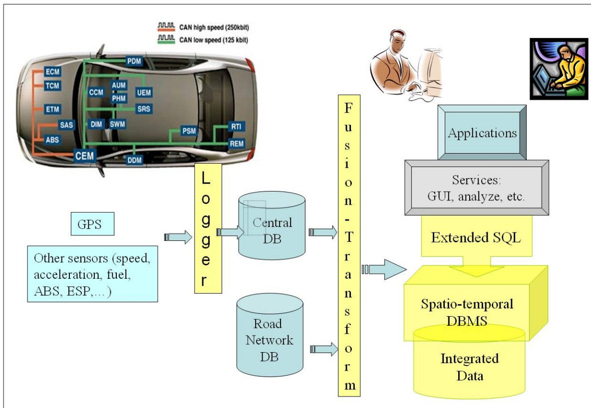
Figure III.5. Example of data chain processing
