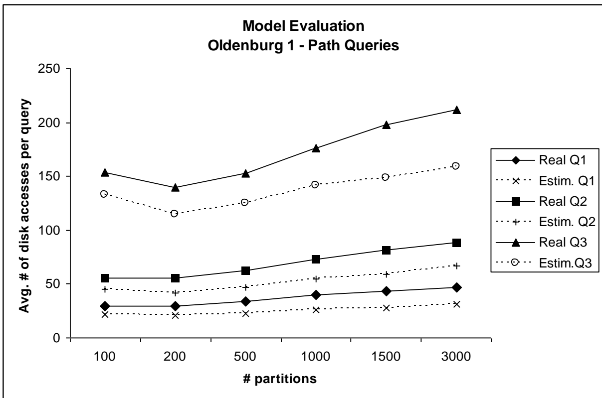
Figure V.12: PARINET cost model evaluation for small data set
