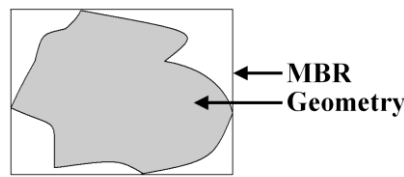
Figure II.6: Example of a MBR enclosing a geometry
