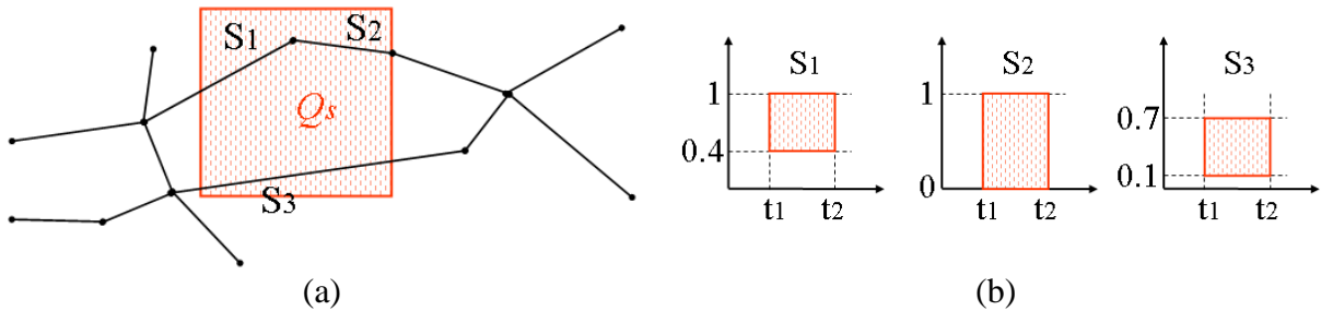
Figure IV.18: Example of query mapping from the 2D space (a) to the network space (b)
