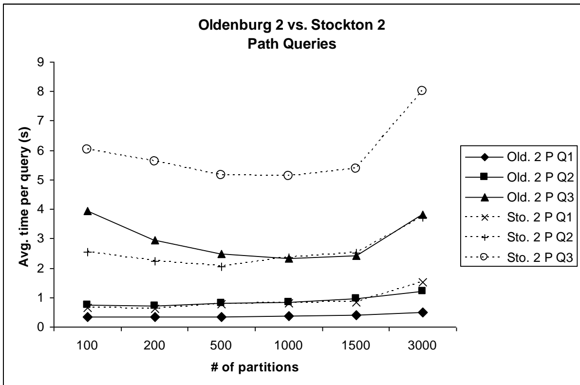
Figure V.11: PARINET query performance - path queries on large data sets
