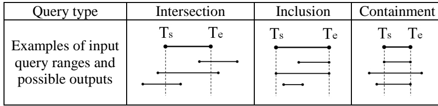
Figure IV.8: Particular types of queries over intervals
