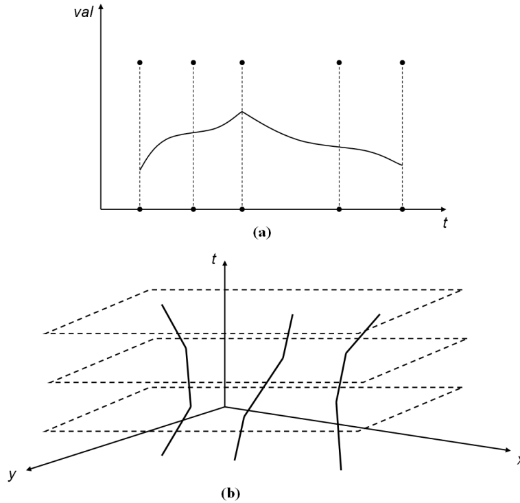
Figure II.15: Sliced representation of moving(real) and moving(points) value
