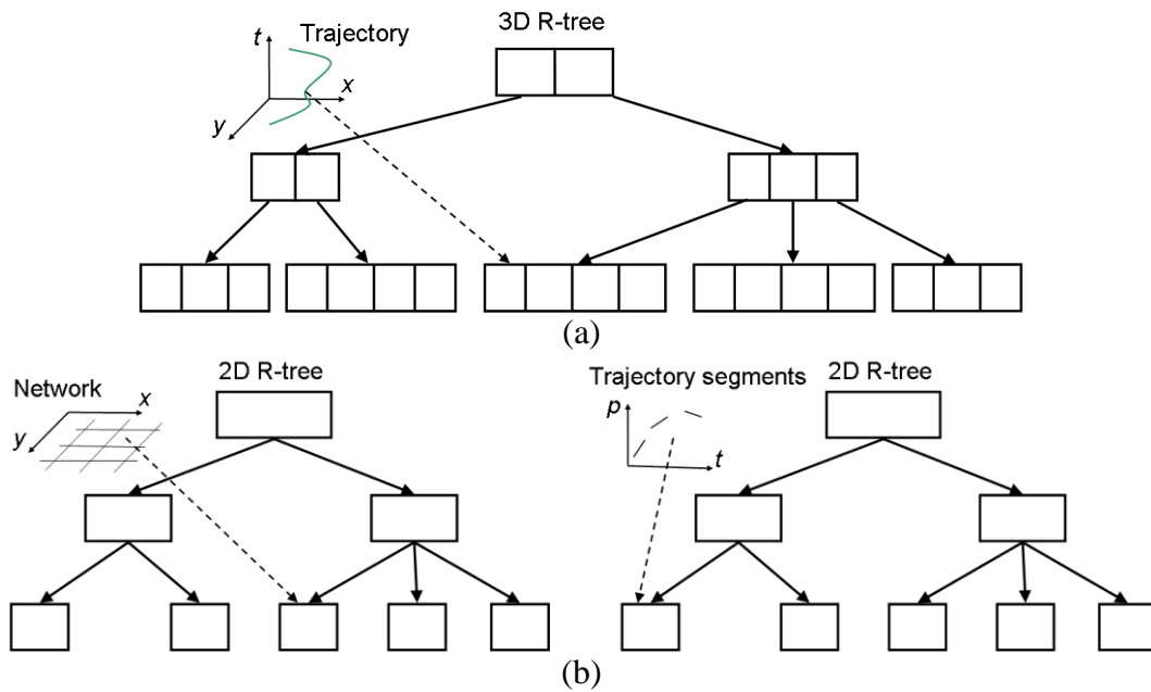
Figure IV.17: Replacing one 3D index (a) with two 2D indexes (b)
