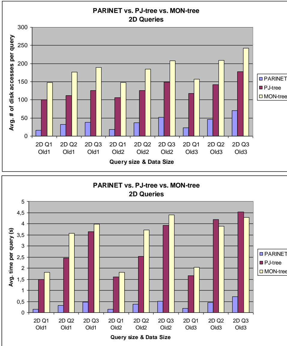
Figure V.6: Performance comparison between PARINET, PJ-tree and MON-tree for 2D queries
