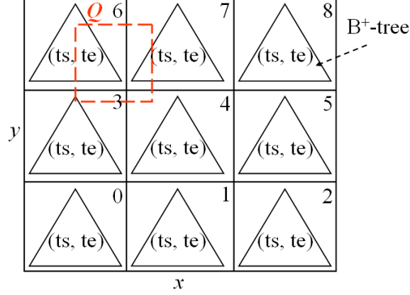
Figure IV.14: PIST's approach for a 3 \times 3 regular grid
