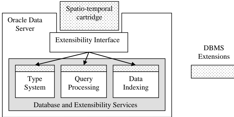
Figure III.6. Database System Architecture
