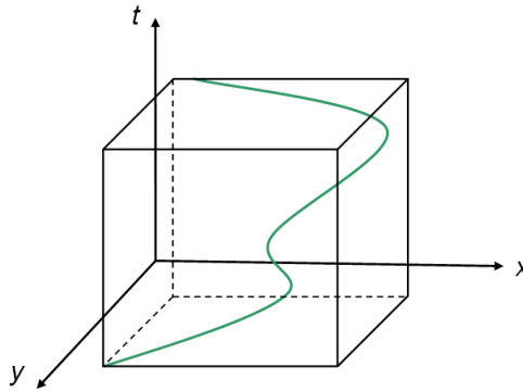
Figure IV.11: The MBB of a moving object occupies a large portion of the data space
