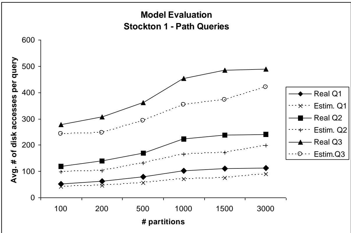
Figure V.14: PARINET cost model evaluation for small data set
