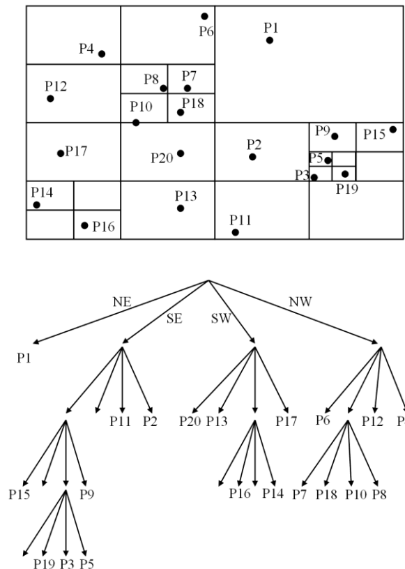
Figure IV.5: Example of a quadtree
