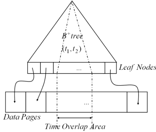
Figure V.4: Example of index range scan
