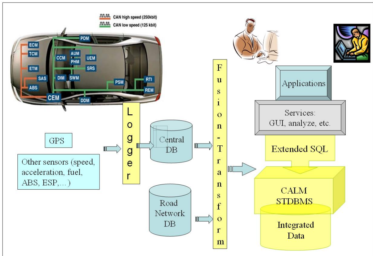
Figure VI.1: Data-chain processing in naturalistic driving applications
