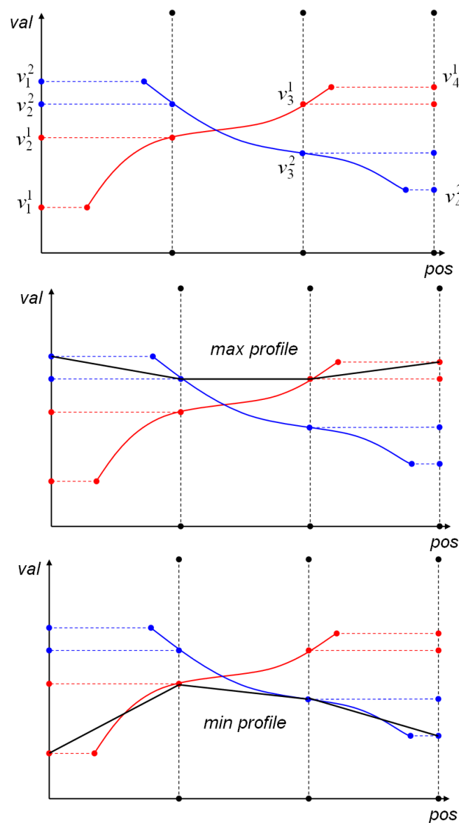
Figure III.9. Example of calculating the max_agg (second graph) and min_agg (third graph) on two profiles (first graph) using a regular slicing
