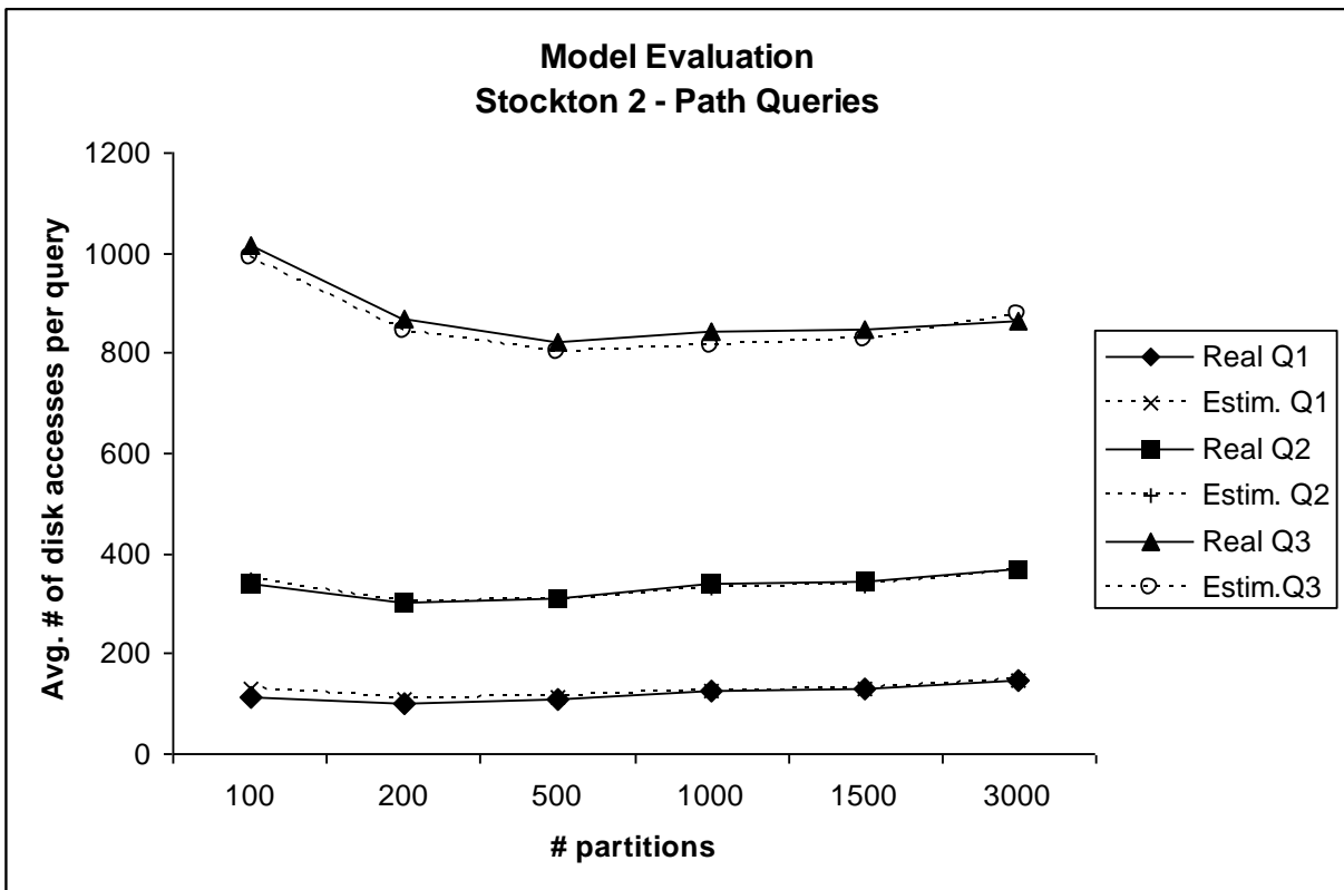
Figure V.15: PARINET cost model evaluation for large data set
