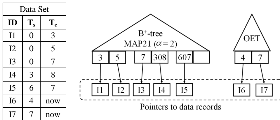
Figure IV.9: Example of the MAP21 indexing approach
