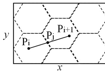
Figure IV.13: Spatial partitioning and segment splitting in SETI
