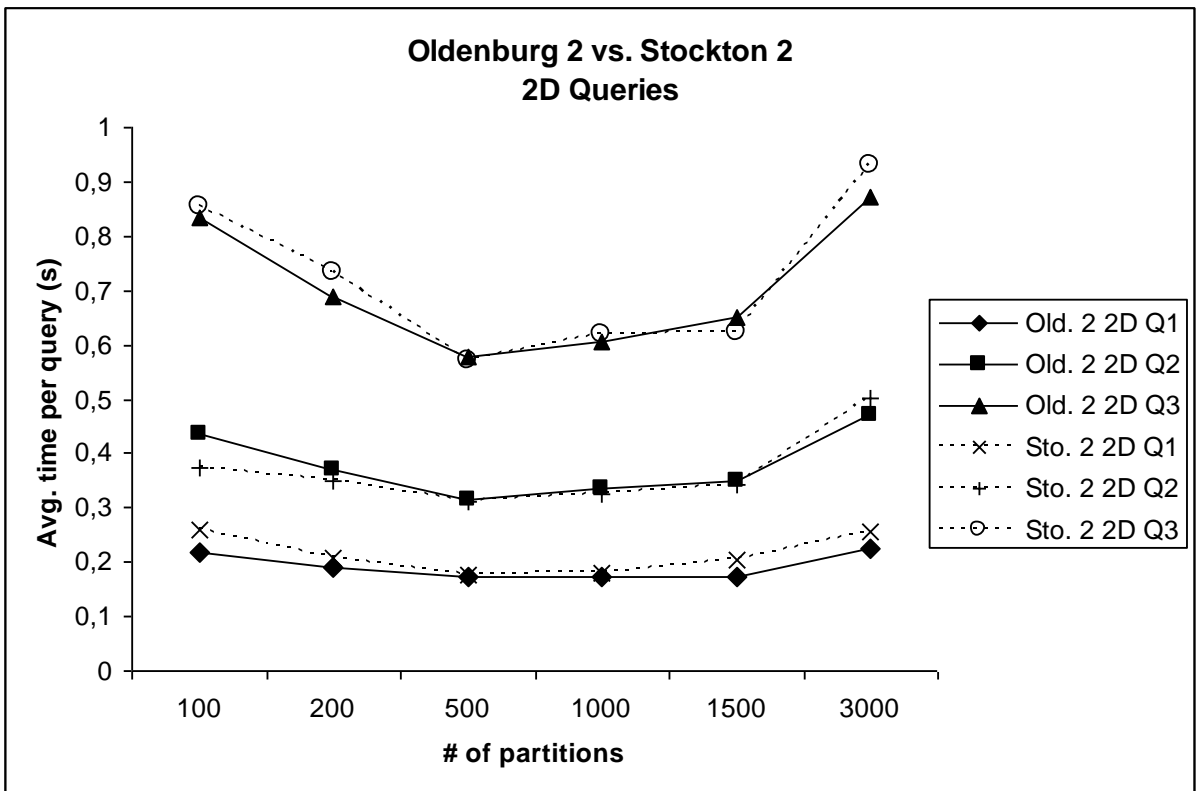
Figure V.10: PARINET query performance - 2D queries on large data sets
