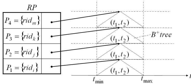
Figure V.3: Example of PARINET index structure
