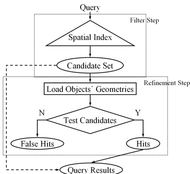
Figure IV.3: Two-step spatial query processing
