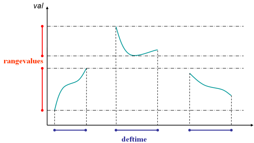
Figure II.10: Example of deftime and rangevalues projections over a moving(real)
