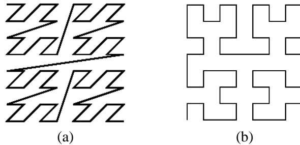
Figure IV.6: Two space-filling curves: (a) z-ordering and (b) Hilbert curve
