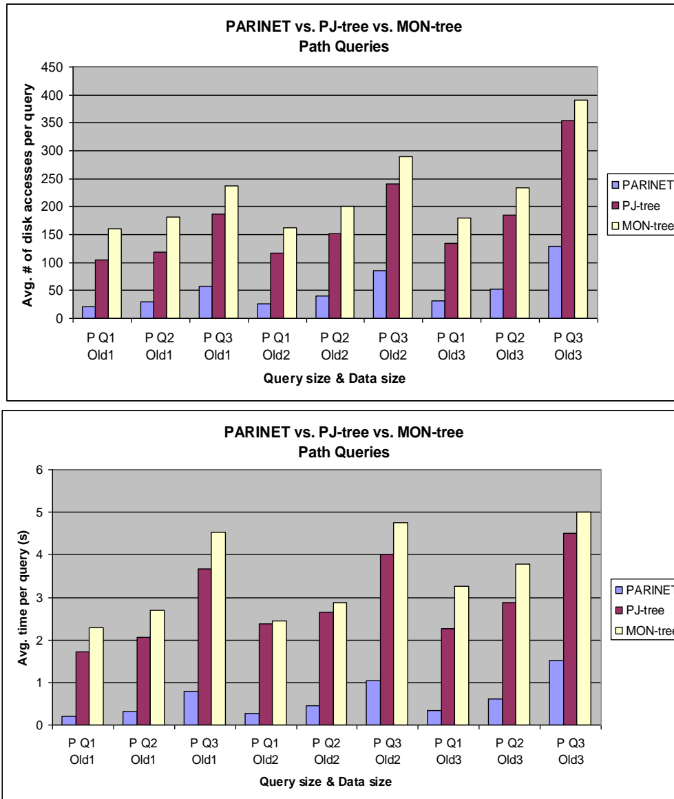
Figure V.7: Performance comparison between PARINET, PJ-tree and MON-tree for path queries
