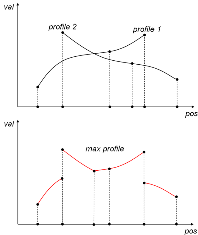
Figure III.8. Example of fragmentation after using the max_agg (second graph) on two profiles (first graph)
