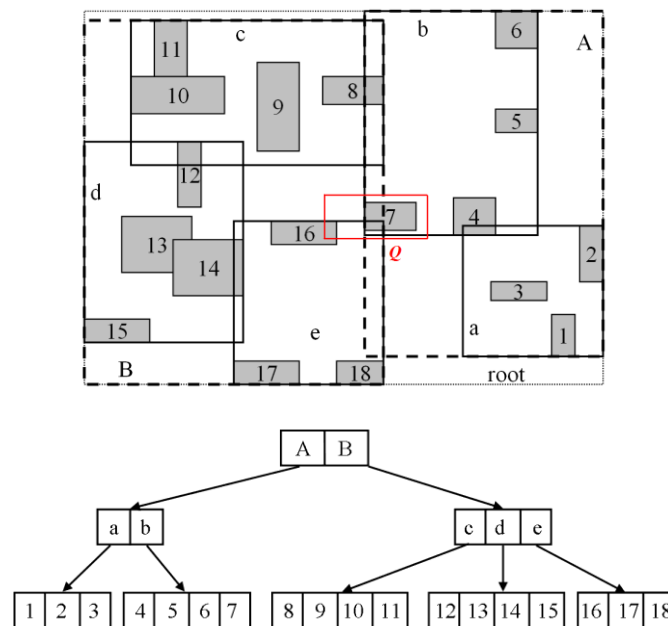
Figure IV.7: Example of an R-tree hierarchical index on MBBs
