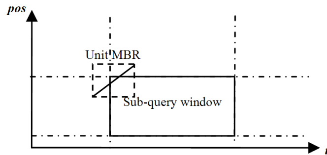
Figure V.2: Example of unit and sub-query intersection
