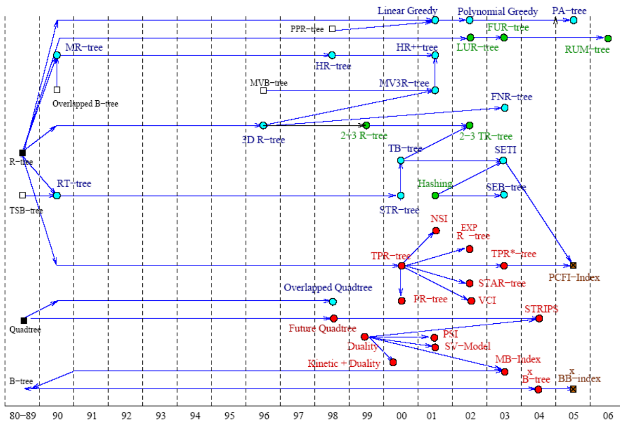
Figure IV.12: Spatio-temporal access methods (blue → past; green → present; red → future; brown → all) [74]
