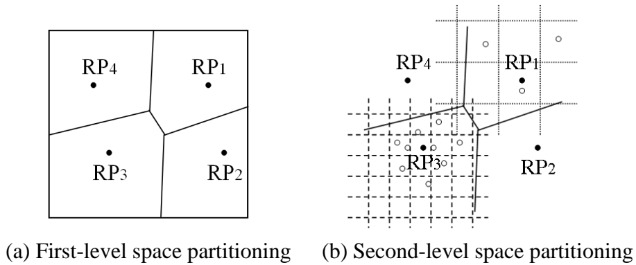
Figure IV.16: ST^2B -tree: Space partitioning
