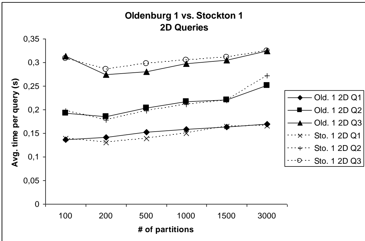
Figure V.8: PARINET query performance - 2D queries on small data sets
