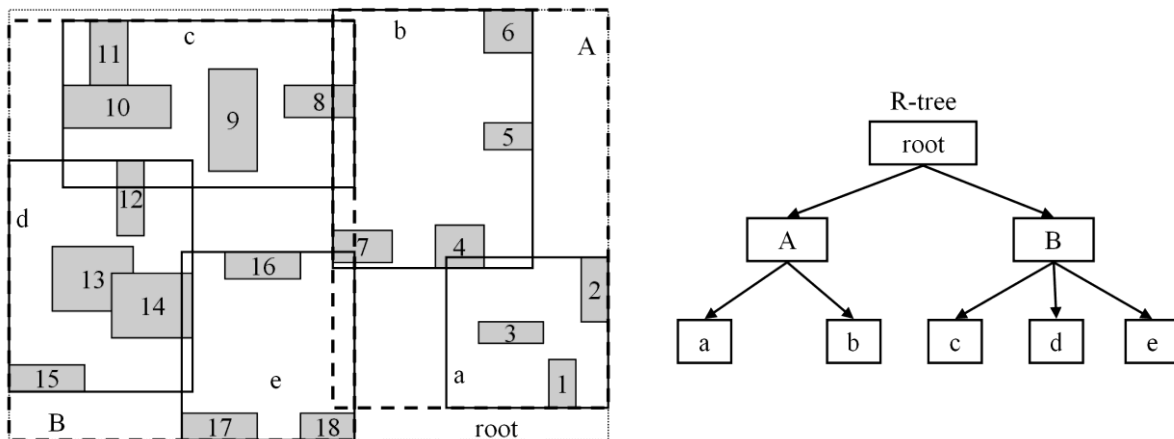
Figure II.7: Example of an R-tree hierarchical index on MBRs
