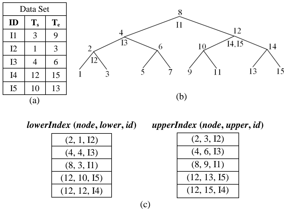
Figure IV.10: Example for an RI-tree. a) five intervals. b) virtual backbone and registration positions of the intervals. c) resulting relational indexes lowerIndex and upperIndex
