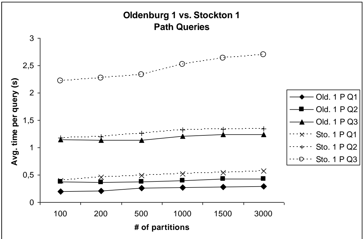
Figure V.9: PARINET query performance - path queries on small data sets
