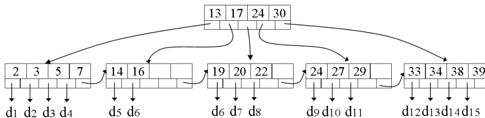
Figure IV.4: A simple B + -tree example
