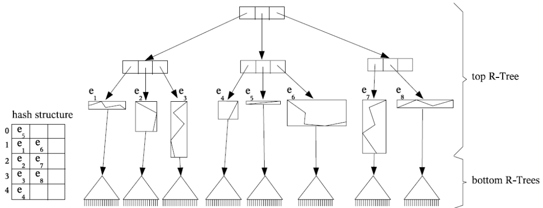
Figure IV.19: Example of the MON-tree index structure [102]
