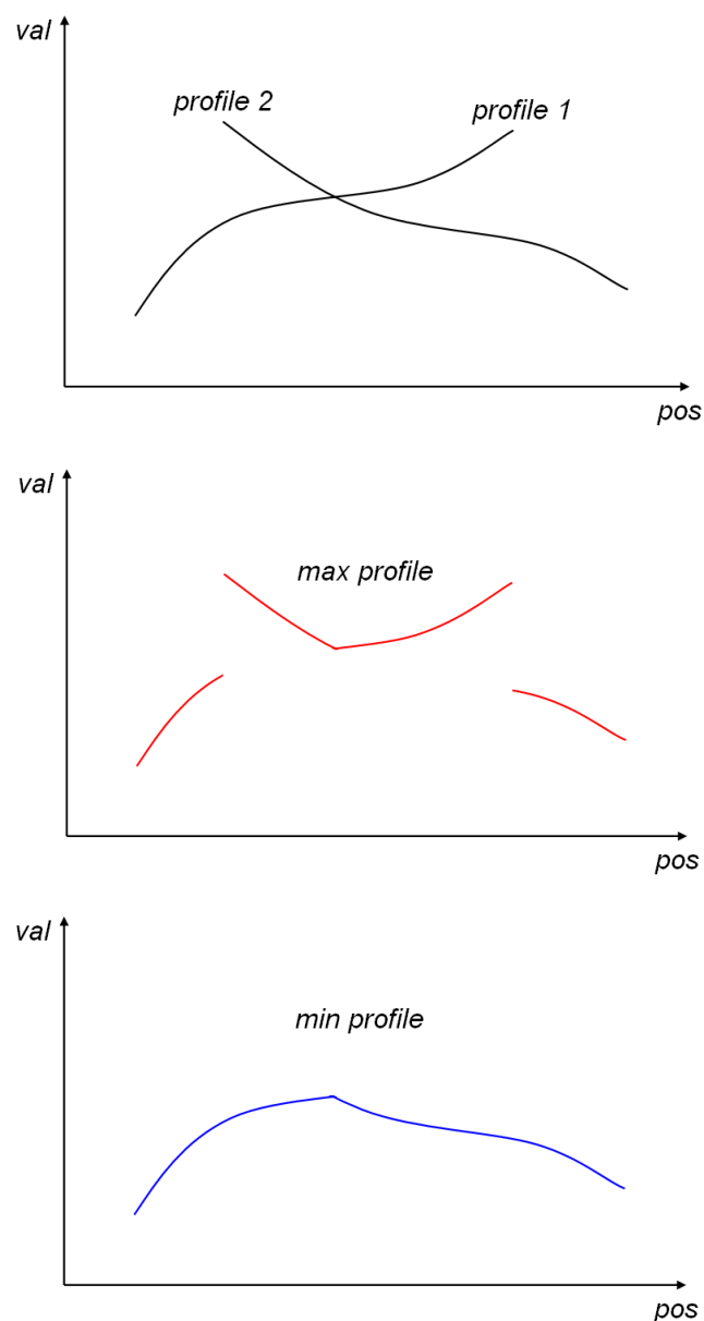
Figure III.4. Example of using max_agg (second graph) and min_agg (third graph) on two profiles (first graph)
