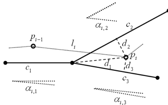
Figure VI.6: Incremental map-matching example
