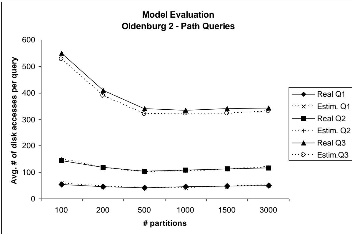
Figure V.13: PARINET cost model evaluation for large data set
