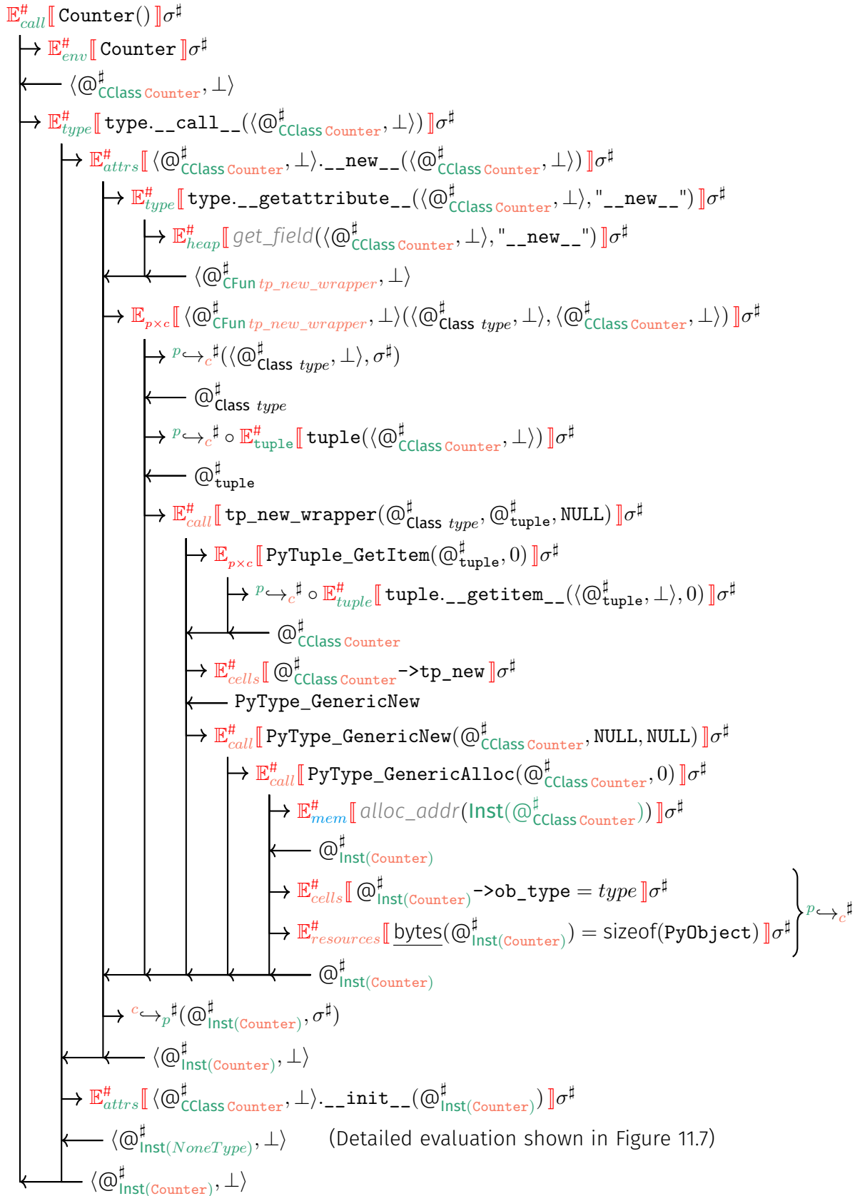
Figure 11.6: Sequence diagram of the analysis of Counter creation (Listing 9.1, line 4) – part 1
