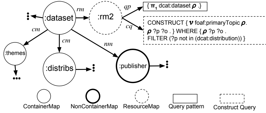
FIGURE 4.6: Example of a NonContainerMap
