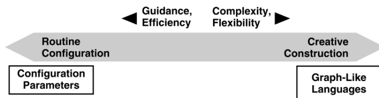
FIGURE 3.5: Main types of domain-specific language [SVB + 06]
