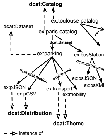
FIGURE 4.7: Example of an interpretation of a data source
