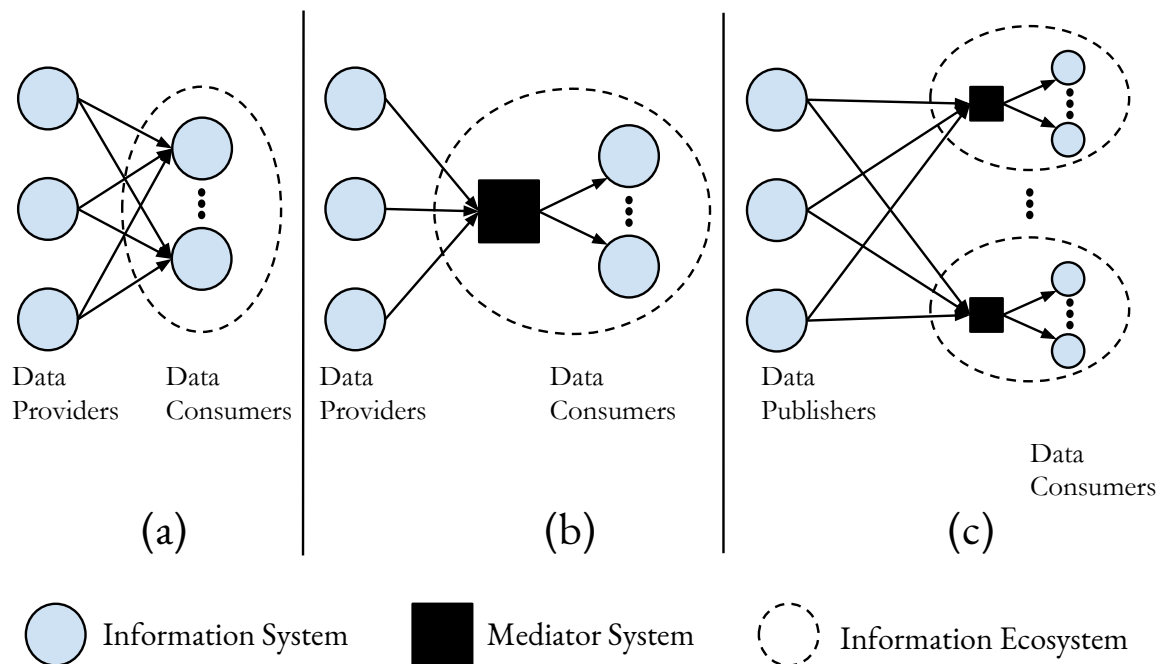
FIGURE 1.4: Data Integration Approches
