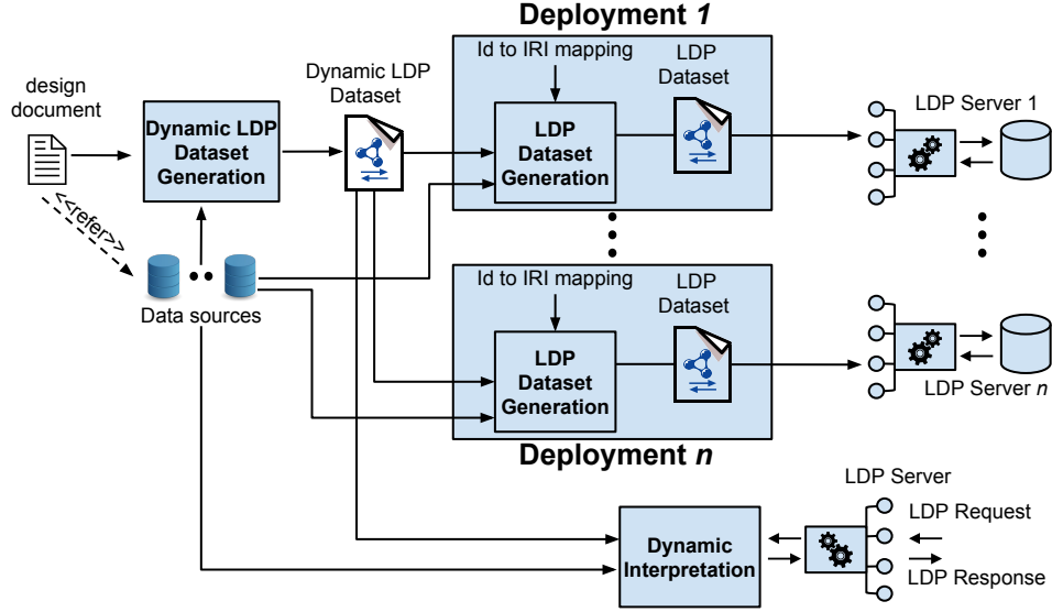
FIGURE 4.12: Application of dynamic LDP datasets
