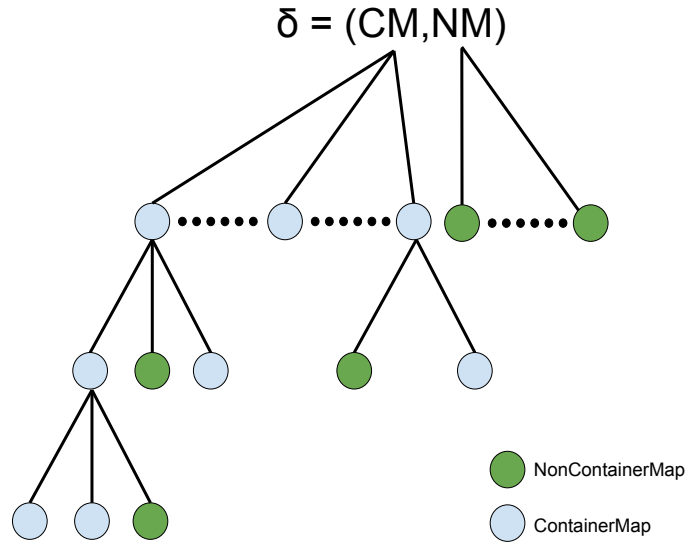
FIGURE 4.13: Abstract View of design document \delta containing maps that are finite and having no cycles
