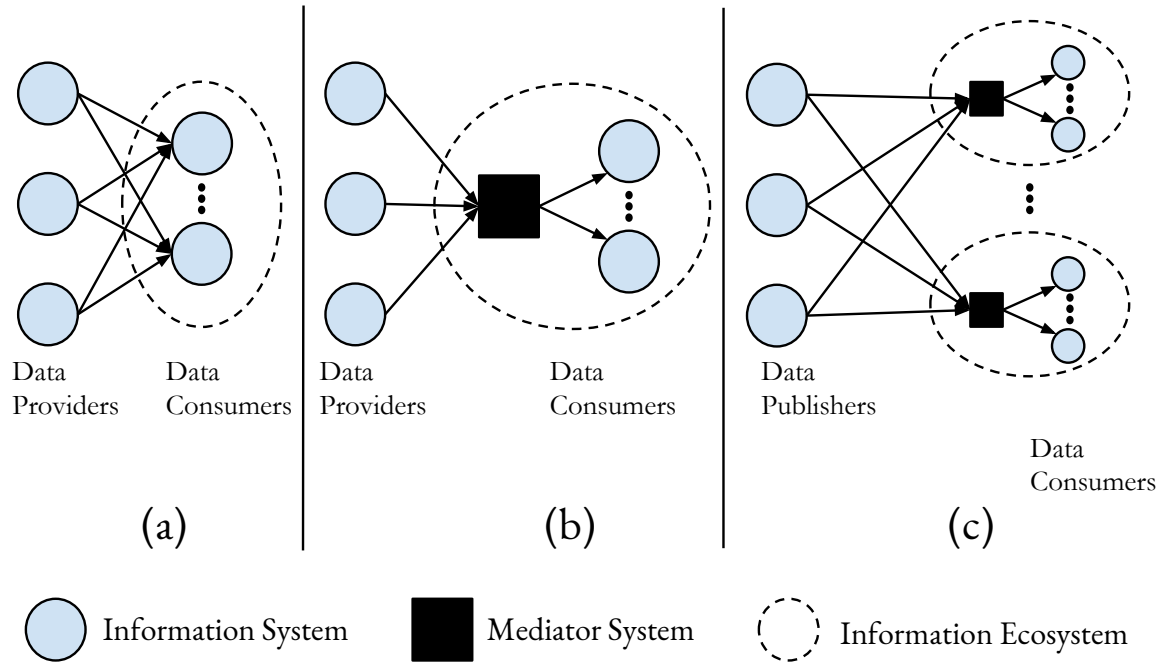
FIGURE 1.4: Data Integration Approaches
