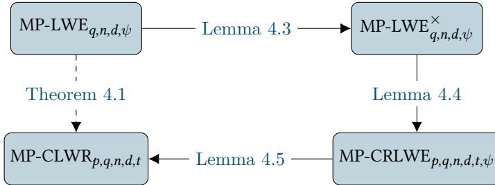
Figure 4.2: Overview of the proof of Theorem 4.1.
