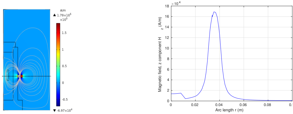
(a) Color map of the distribution of the z component of the magnetic field in ( \text{A} \cdot \text{m}^{-1} ) in the 2D axisymmetric model. (b) H_z versus the radius r . The z component of the magnetic field is computed through a horizontal line defined at Z = 0.0675 m and crossing the magnet center.
