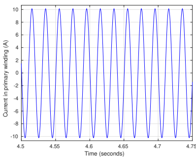
(a) Current I_1 versus time.
