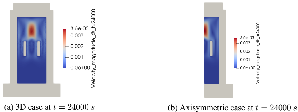
Figure 4.2: Color maps of the velocity magnitude (in \text{m}\cdot\text{s}^{-1} ) when the magnetic force is inactive. The symmetry axis ( Oz ) is on the left for the axisymmetric model (panel b).
