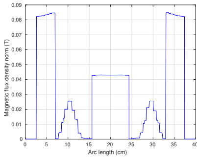
(a) Magnetic flux density (in T) along B_1 .
