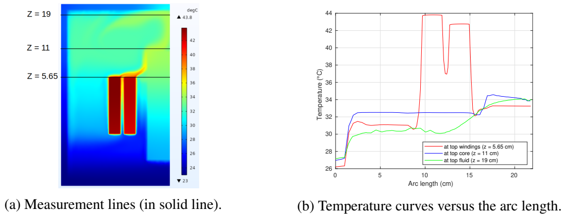
Figure 4.67: Temperature evolution (in ^{\circ}\text{C} ) in (y, z) plane and x = 0 at a steady state t = 15\,000 s using mesh 1.
