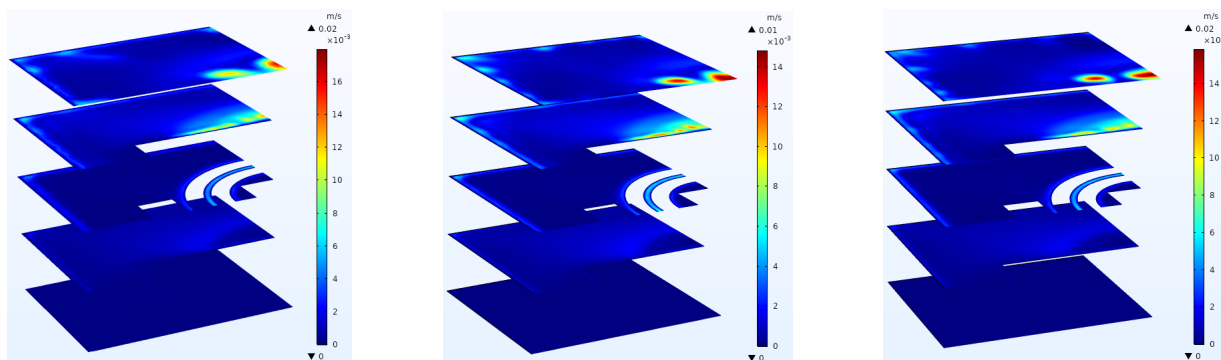
(a) Mesh 0.
