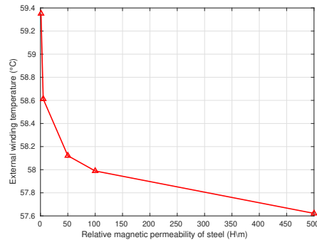
Figure 4.18: Variation of the external conductor temperature versus the relative magnetic permeability of steel.
