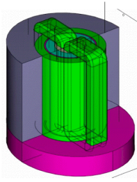
Figure 2.39: Partial view of a prototype power transformer cooled with ferrofluid [86, p. 145].
