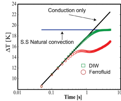
Figure 2.20: Temperature increase for the heated wire, bath temperature = 40^{\circ}\text{C} , supplied current I = 1.5\text{A} [22, p. 303]
