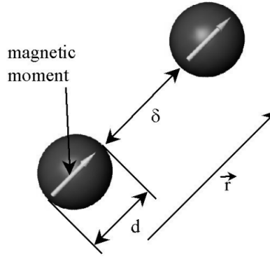
Figure 2.3: Sketch of magnetic dipole-dipole interaction [10].
