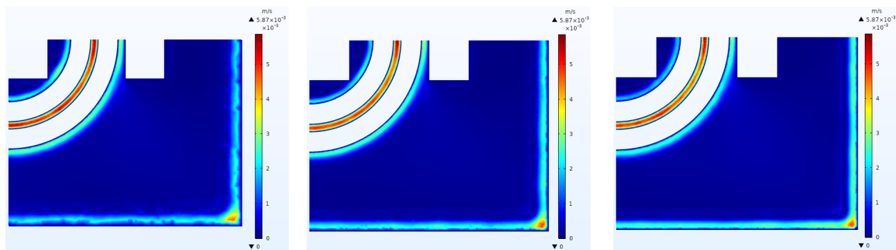
(a) Mesh 0.
