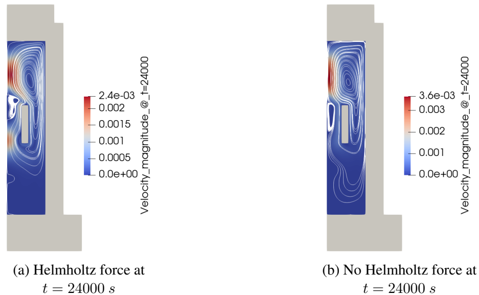
Figure 3.24: Color maps of the velocity magnitude (in \text{m.s}^{-1} ) with and without the magnetic force. The symmetry axis ( Oz ) is on the left.
