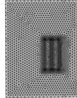
(c) mesh in (x, z) plane and y = 0 .
