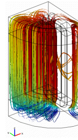
Figure 2.40: Streamlines of the velocity field in the vertical configuration [86, p. 146].
