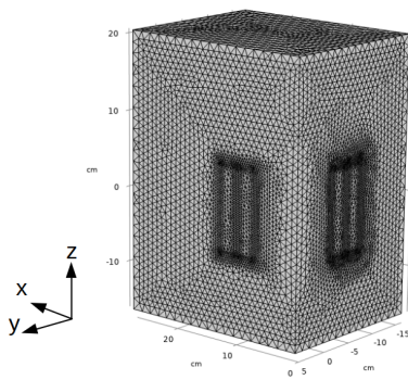
(a) 3D tetrahedral mesh.
