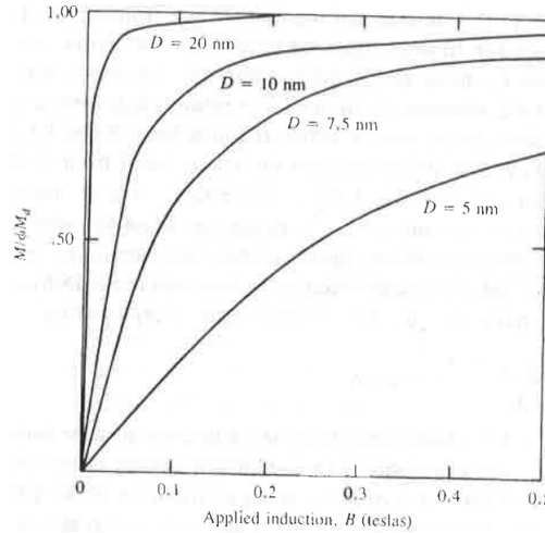
Figure 2.7: Magnetization curves computed for monodisperse spherical particles of magnetite ( M_d = 4.46 \times 10^5 \text{ A}\cdot\text{m}^{-1} ) [6].
