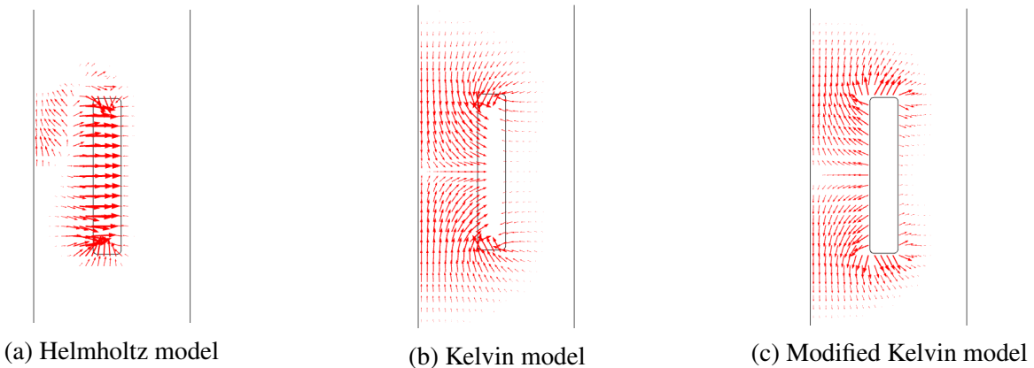
Figure 3.19: Spatial distribution of magnetic force fields for different models at t = 24\,000 s.
