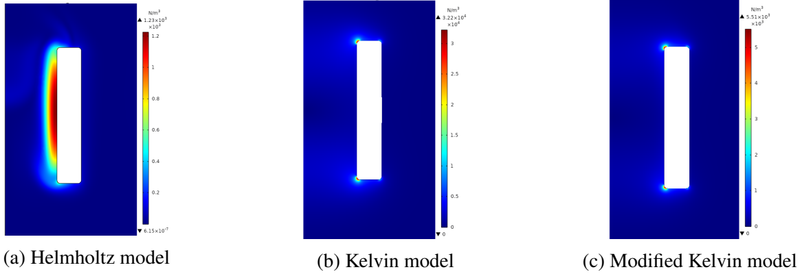
Figure 3.18: Intensity distribution of the magnetic body force (in \text{N}/\text{m}^3 ) for different models at t = 24\,000 s.
