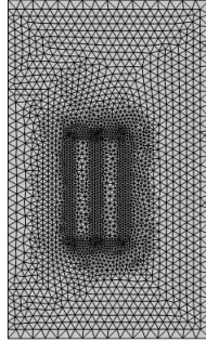
(b) mesh in (y, z) plane and x = 0 .
