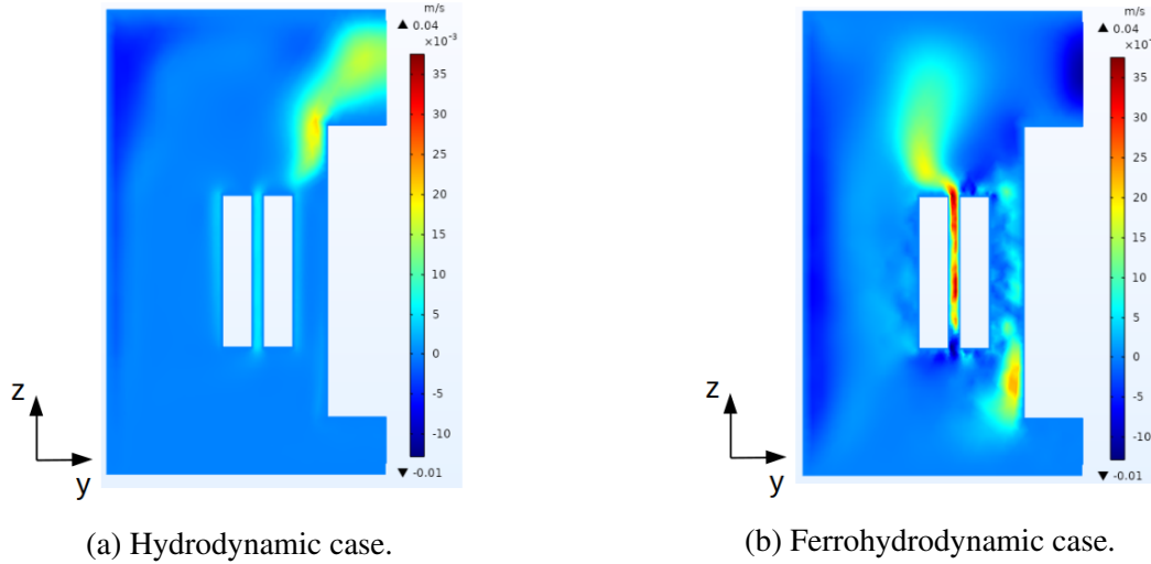
Figure 4.51: Distributions of the z component of the velocity field v_z (in \text{m.s}^{-1} ) in (y, z) plane and x = 0 at a steady state t = 15000 s.
