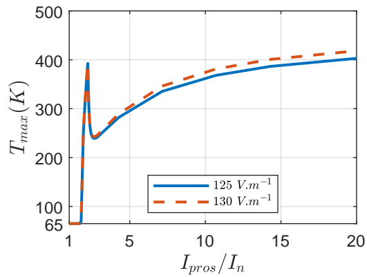
Figure 5.8: Maximum temperature as a function of the prospective current normalized by the rated current of the circuit using the actual resistance per unit length of the conductor at two electric fields.
