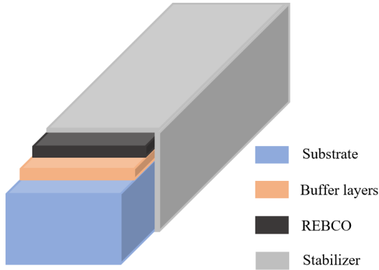
Figure 1.12: Simplified architecture of a 2G HTS tape.
