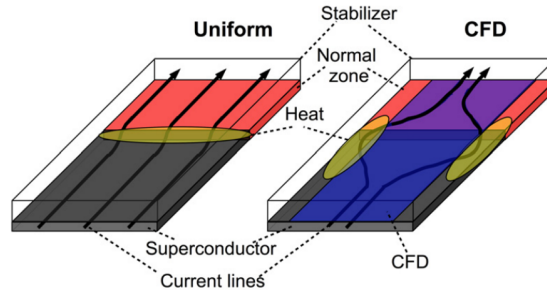
Figure 2.20: Schematic drawing of the current path flows in a uniform (left) and CFD tape (right) from [82].
