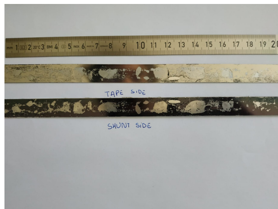
Figure 5.17: Fastgrid conductor manufactured with the industrial process. The sample was delaminated in purpose.
