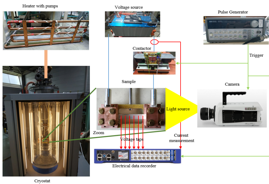
Figure 3.15: Scheme of user-controlled elements of the set-up.
