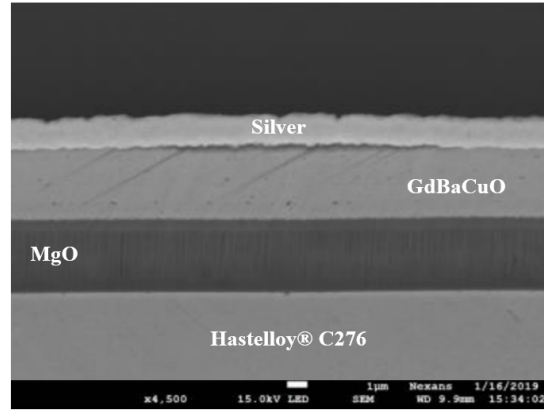
Figure 1.13: Cross-section of a REBCO coated conductor from THEVA (Scanning Electron Microscopy) (Courtesy of Nexans®).
