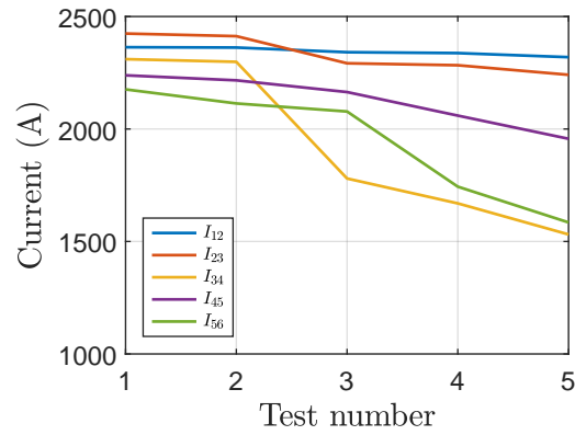
Figure 5.16: Evolution of the current giving an electric field of 10 V/m on the five portions of the sample of the conductor produced with the industrial manufacturing process of THEVA as a function of the test number.
