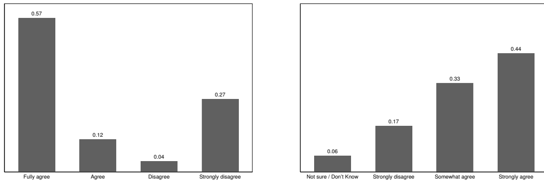
Figure 1.2: Agents' perceptions about redistributive pressure
