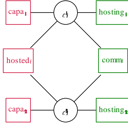
Figure 6.5 – Factor graph representation of a the DCOP model for migrating computation c_i
