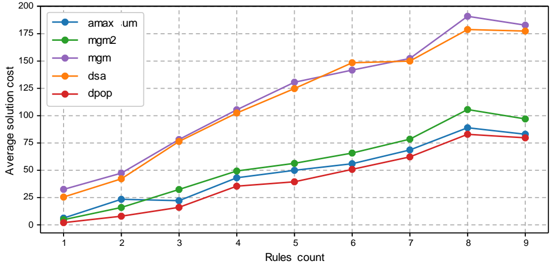
Figure 4.15 – Average solution cost for SECP with a growing number of rules, solved with several DCOP algorithms
