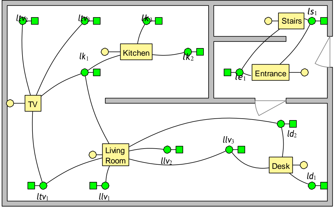
Figure 4.7 – Factor graph for a realistic full house level
