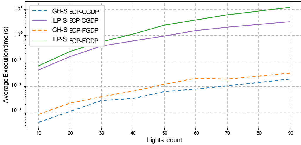
Figure 5.13 – Times for computing a distribution for increasing size SECP instances with several SECP -specific distribution methods
