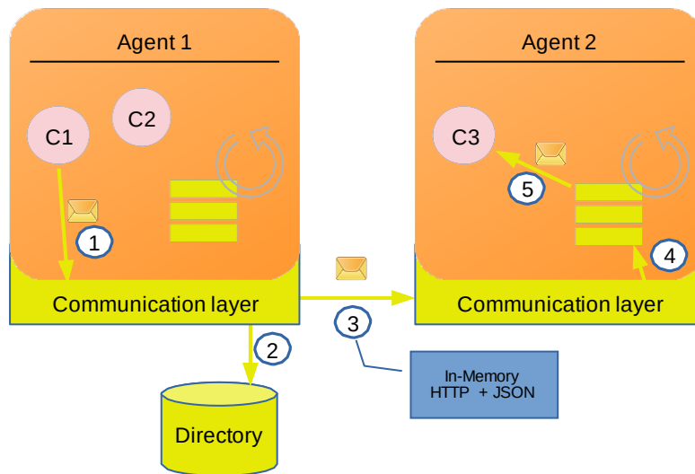
Figure 7.4 – pyDCOP Inter-agent Communication Scheme
