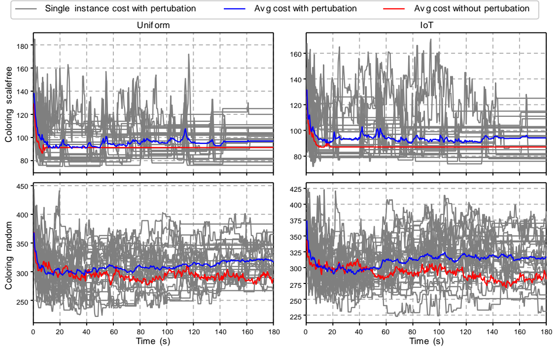
Figure 6.23 – Cost of A-MaxSum solution at runtime, with (blue) and without perturbation (red), on uniform (left) and problem-dependent (right) infrastructure, and when solving scale free graph coloring (top) and random graph coloring (bottom), using DRPM[MGM-2] to repair
