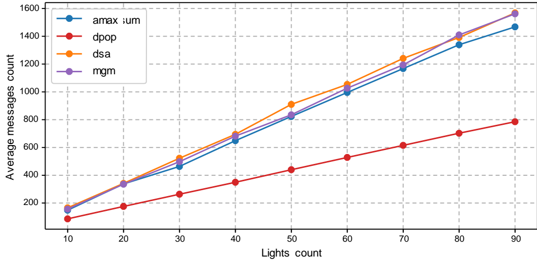
Figure 4.12 – Messages count and communication load for increasing size SECP instances with several DCOP algorithms
