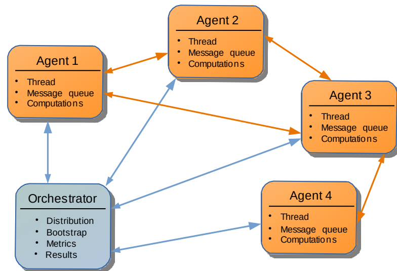
Figure 7.3 – Sample pyDCOP Architecture Instantiation
