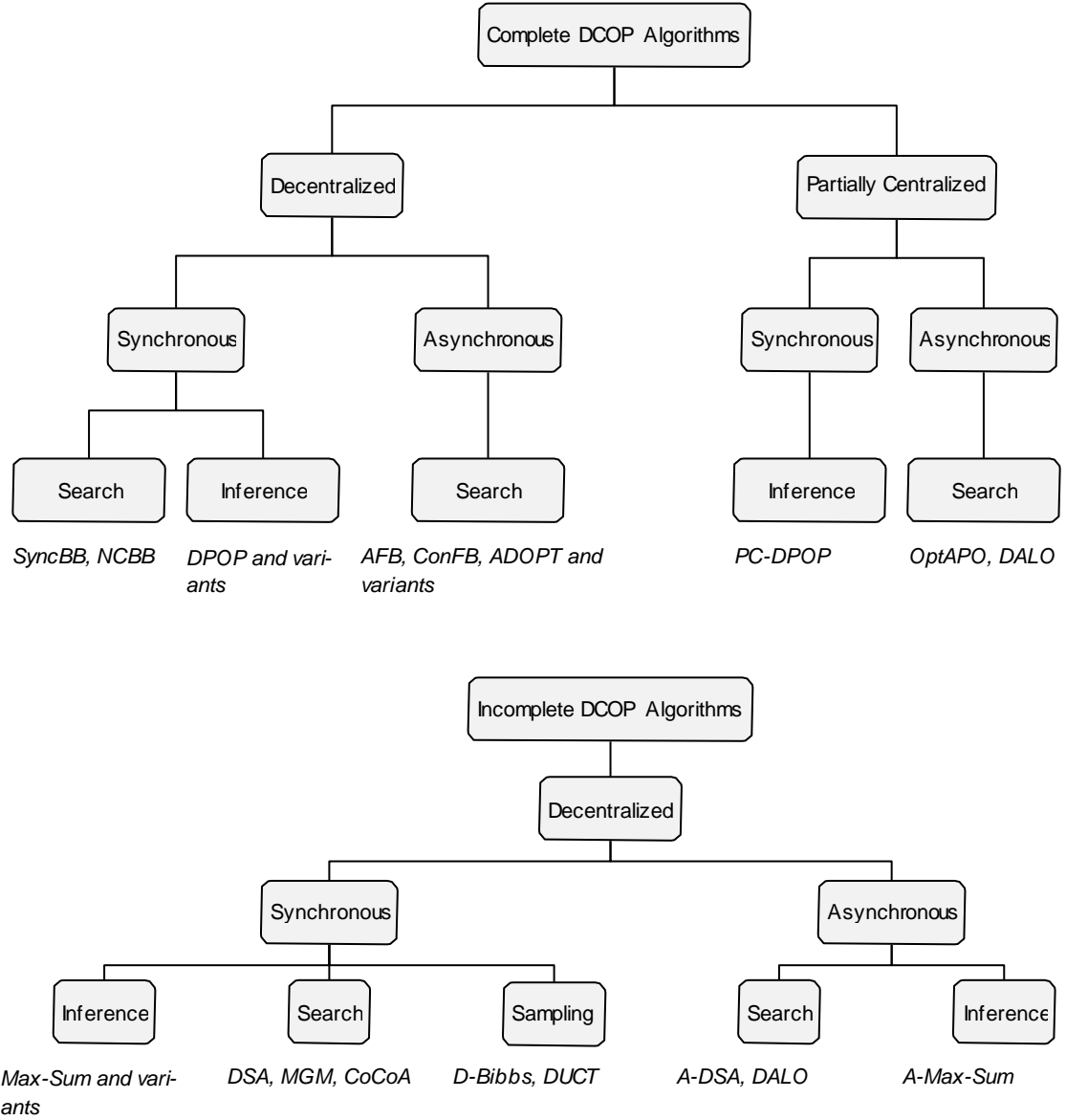
Figure 3.8 – DCOP taxonomy
