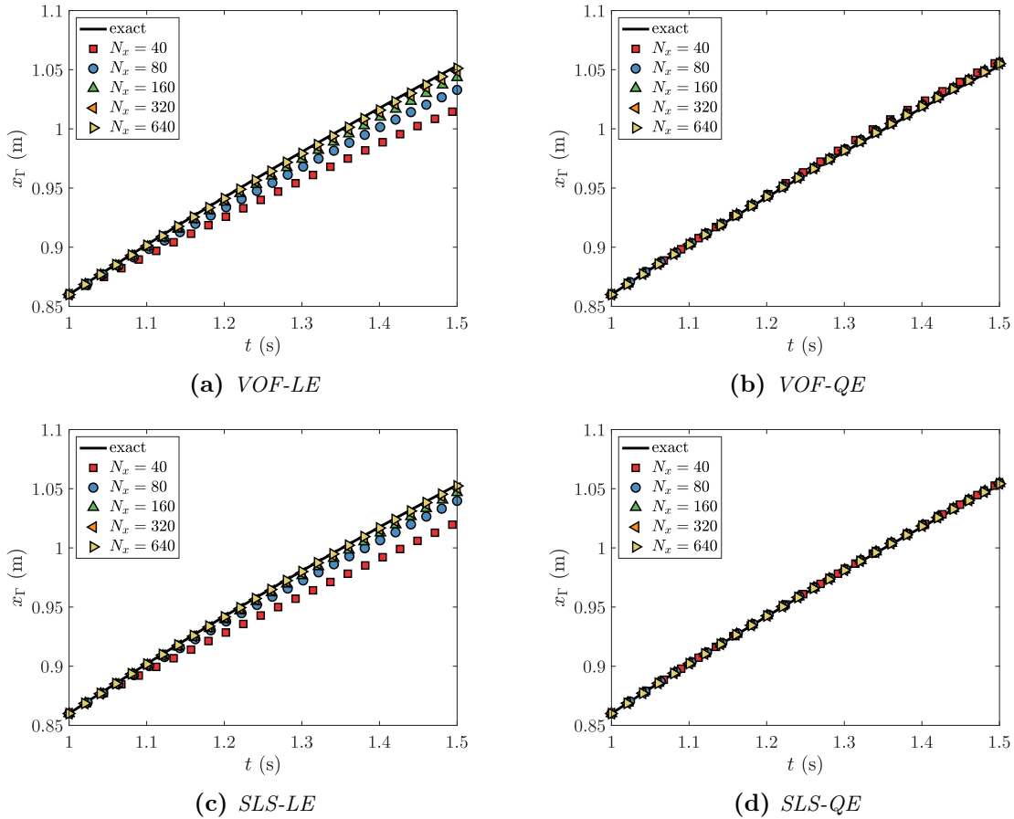
Figure 9.3: Interface position evolution x_\Gamma(t) for the planar Frank sphere problem
