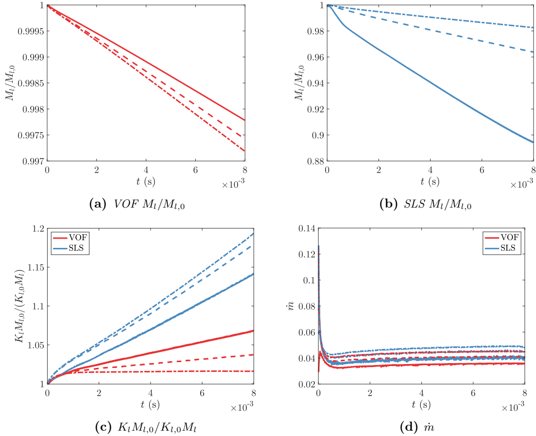
Figure 9.14: M/M_0 , K_l M_{l,0}/K_{l,0} M_l and \dot{m} temporal evolution for VOF and SLS for the convected droplet evaporation using the standard treatment of velocity in the imposition of \nabla \cdot \mathbf{u}^{n+1} . The three meshes N_D = 10 (—), N_D = 20 (---) and N_D = 40 (-·-) are represented.
