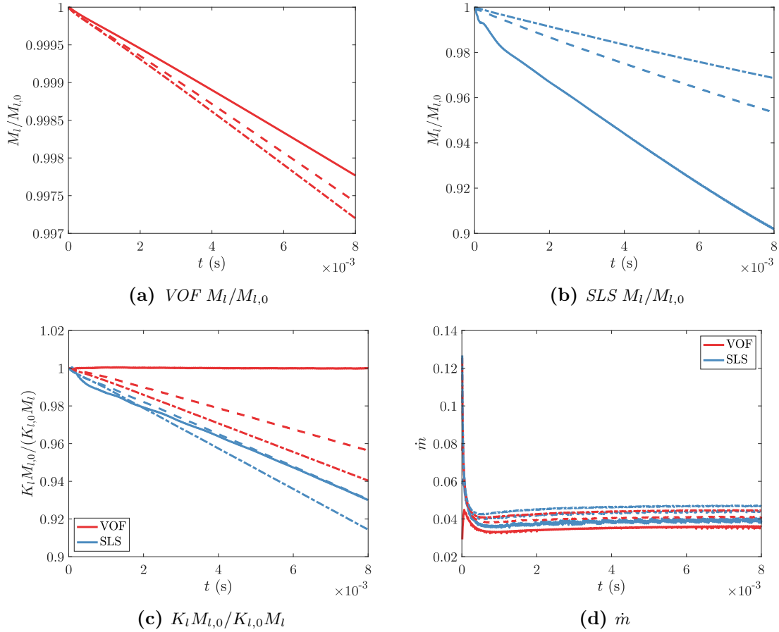
Figure 9.18: M/M_0 , K_{i,0}M_{i,0}/K_{i,0}M_i and \dot{m} temporal evolution for VOF and SLS for the convected droplet evaporation using MA2. The three meshes N_D = 10 (—), N_D = 20 (---) and N_D = 40 (-·-·) are represented.
