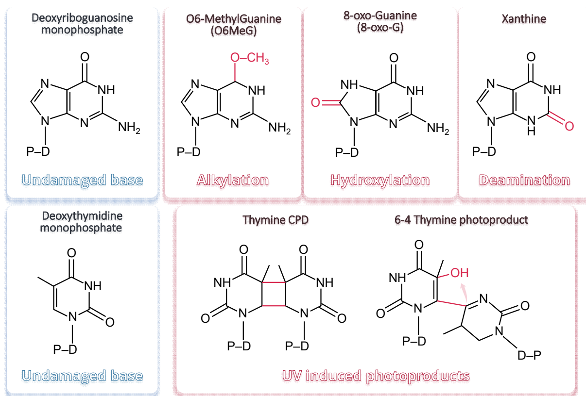
Figure 2. Examples of altered bases. Top row: Guanine modified with either alkylation, hydroxylation or deamination reactions. Bottom row : Basic thymine photoproducts. Figure devised with data from [5, 13, 14].
