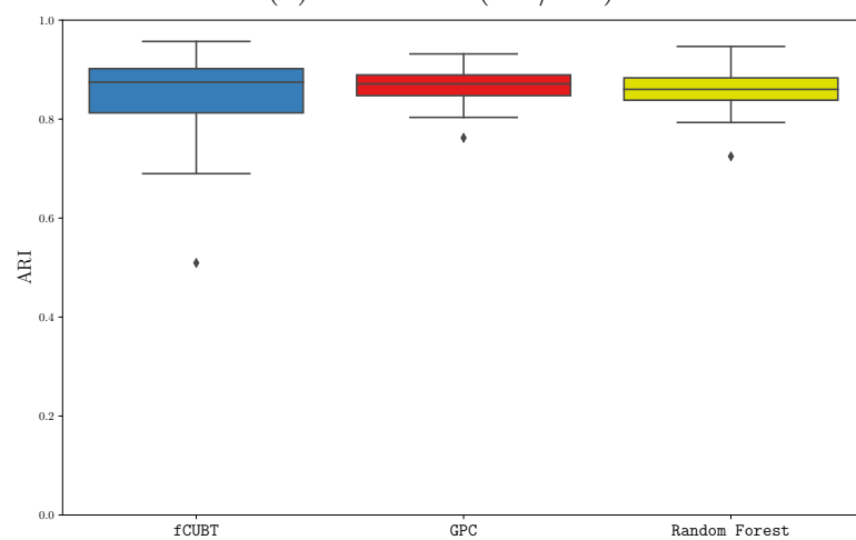
(c) Scenario 3 (188/500)
