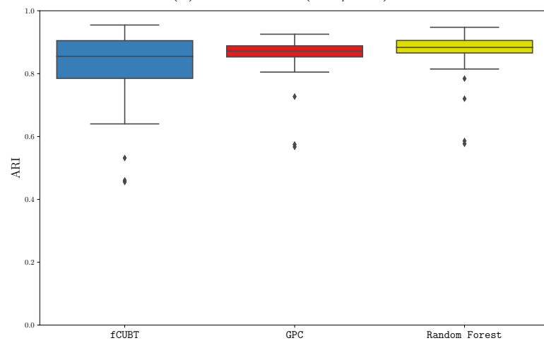
(b) Scenario 2 (172/500)
