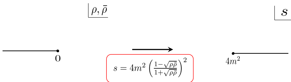
Figure 3.5. The analytic structure of the four-point function in CFT and the flat-space S-matrix. The conformal Mandelstam variables map the branch-cut singularities of the four-point function to a two-particle threshold of the S-matrix.
