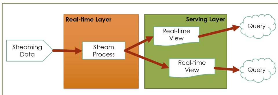
Figure 2.3: Kappa Architecture
