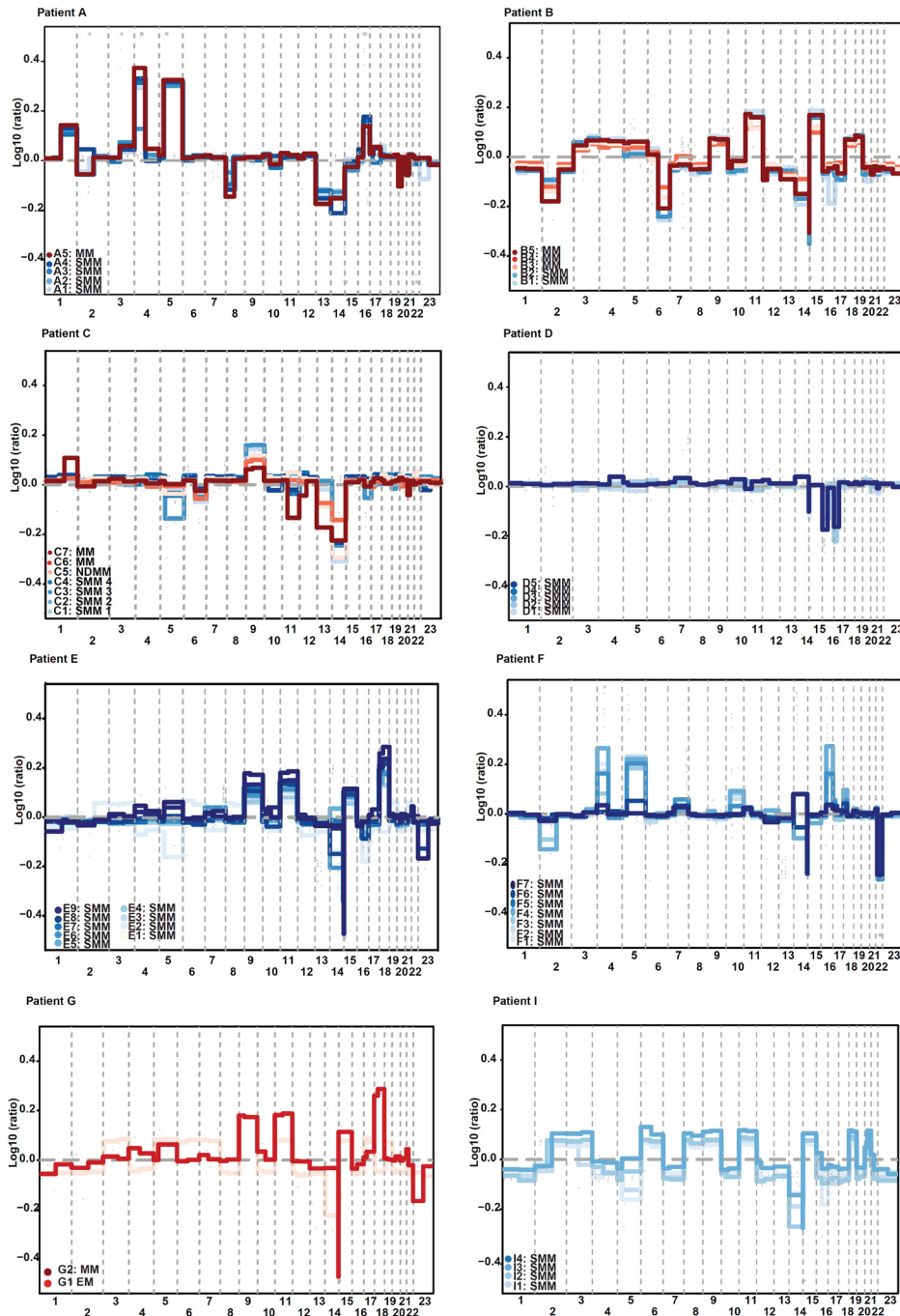
Figure 5.3.2.1.2. Evolution of CNA changes overtime
