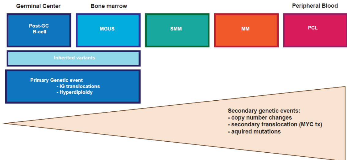
Figure 1.2.1.1. Schematic representation of our current understanding of the genetics of plasma cell disorders where a predisposed post-germinal centre B-cell acquires an initiating event (hyperdiploidy or an IG translocation) and progresses through the various phases of disease by acquiring secondary events (adapted from (Morgan et al , 2012)).
