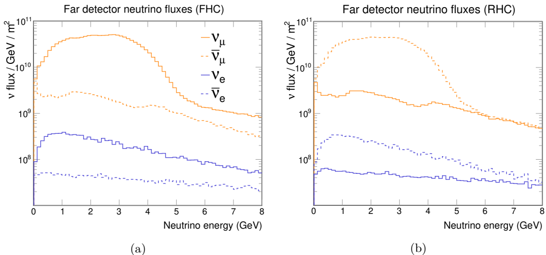
Figure 2.5: Neutrino unoscillated fluxes expected at the DUNE far detector in FHC mode ( i.e. neutrino mode, left) and RHC mode ( i.e. antineutrino mode, right). The plots show the contributions of the \nu_\mu , \bar{\nu}_\mu , \nu_e , \bar{\nu}_e which were created at the beam site (Fermilab). Note that fluxes are given per unit of energy with an energy bin size of 0.125 GeV.
