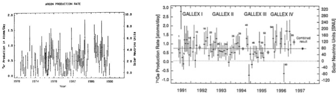
Figure 1.2: The argon production rate (left y axis) and solar neutrino flux (in SNU units) of the Homestake experiment between 1970 and 1990 [10], and from the GALLEX experiment between 1991 and 1997 [17].
