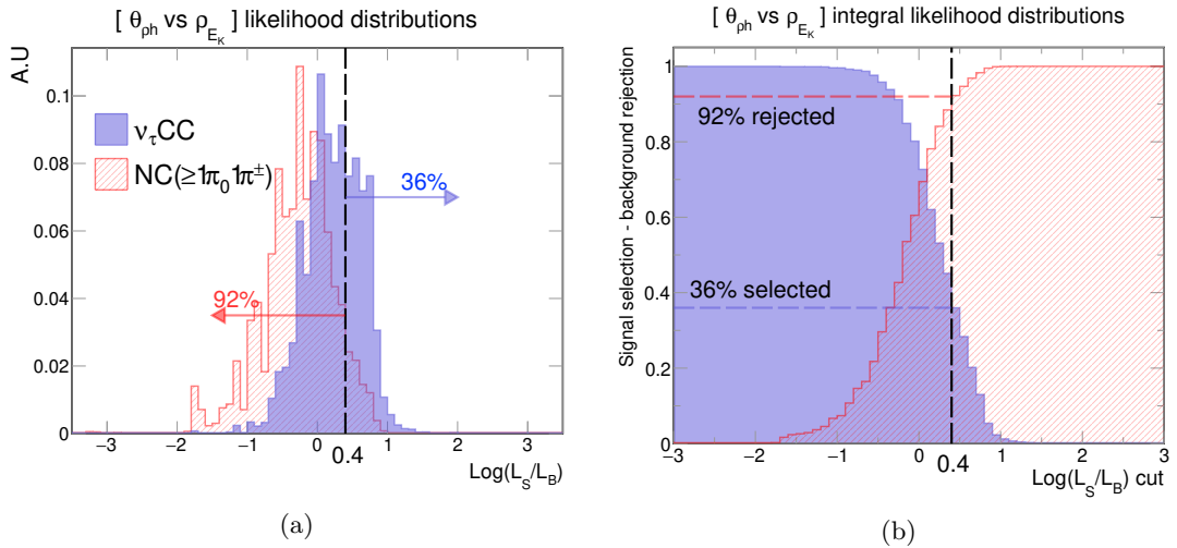
Figure 4.9: Left: log-likelihood ratio distributions of the signal (background) in blue (red) associated to the correlation of the variables \theta_{\rho h} (laboratory angle between the hadronic and the \rho momenta) and \rho_{E_K} (the \rho energy). Right: the integrated distributions of the two. The signal (background) convention is to represent the selection efficiency (rejection efficiency) as a function of the log-likelihood ratio cut value. An illustrative cut at 0.4 is shown. It allows for a 36% selection efficiency and a 92% background rejection efficiency.
