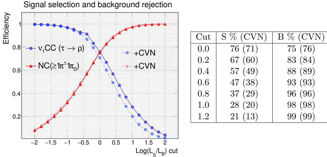
Figure 4.13: Effect of the CVN pre-selection (NC score \geq 0.5 ) on the likelihood efficiencies. The signal selection efficiency (background rejection efficiency) is shown in blue with circle markers (red with triangle markers). Full bright curves (dashed filmy curves) correspond to the case without (with) the CVN pre-selection. The right table reports the corresponding signal selection (S) and background rejection (B) efficiencies in percentage. The efficiencies obtained with the CVN bias are indicated between brackets.
