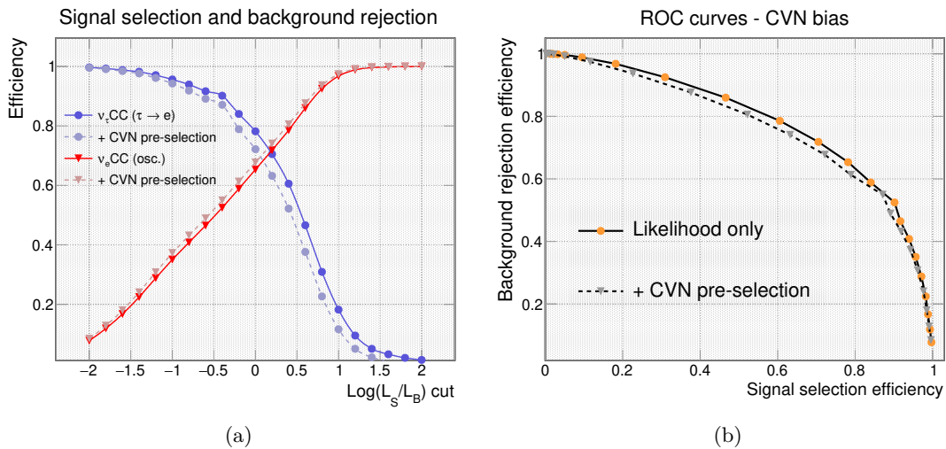
Figure 3.8: Left: signal (blue) and background (red) efficiencies as a function of the log-likelihood ratio cut with (film color) and without (bright color) the CVN pre-selection. Right: ROC curves of these efficiencies with (dashed) and without (full) the CVN pre-selection.
