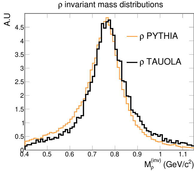
Figure 4.3: \rho invariant mass distributions of hadronic \rho simulated by the library PYTHIA (orange), and \rho of \tau decays simulated by TAUOLA (black).
