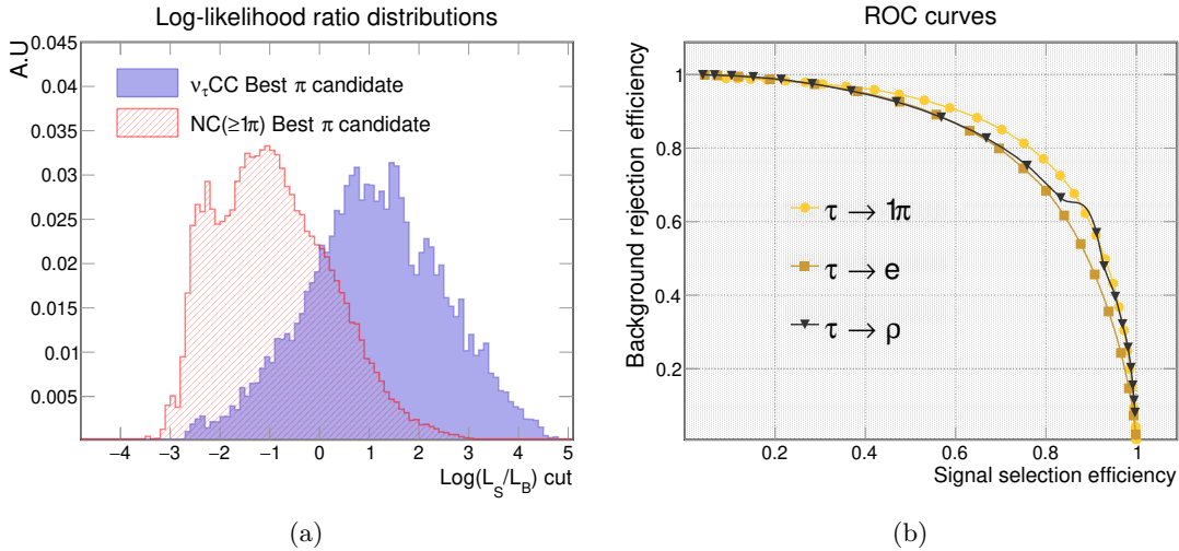
Figure 5.5: Left: Log-likelihood ratio distributions of \nu_\tau CC (blue) and NC( \geq 1\pi^\pm ) (red) for which the Medal Game is used to reconstruct the \tau daughter pion. Right: corresponding ROC curve (background rejection efficiency against signal selection efficiency) in yellow with circle markers. As for comparison, the previous ROC curves obtained for the \tau \rightarrow e analysis (dark orange with square markers) and \tau \rightarrow \rho analysis (black with inverted triangle markers) are shown. The bump of the black spline is an artefact from the ROOT smoothing algorithm.
