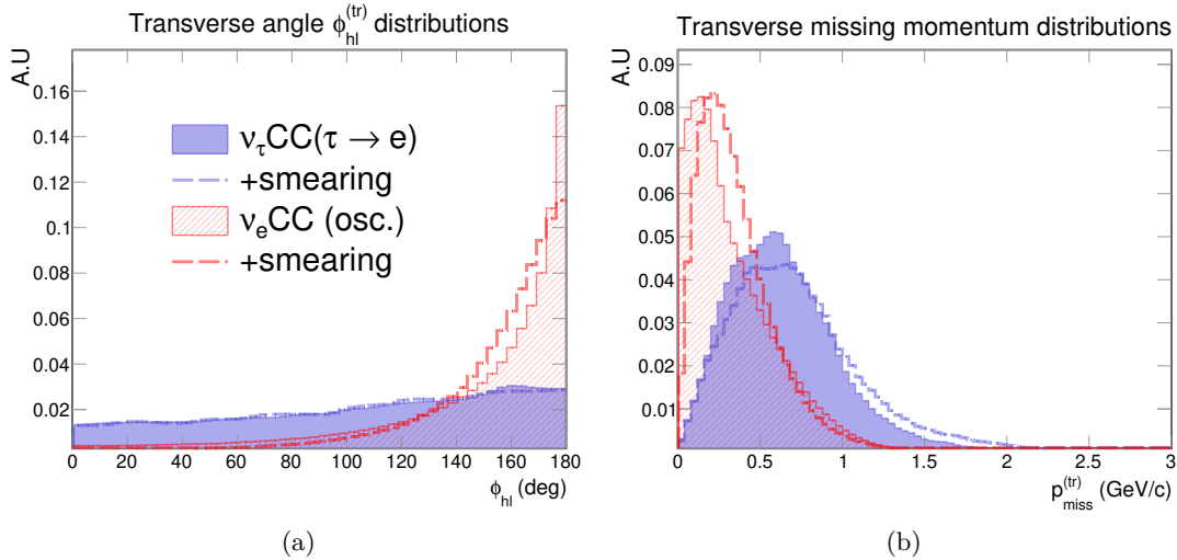
Figure 3.12: Smearing (dashed lines) and not smeared (full) distributions of the transverse angle \phi_{hl}^{(tr)} (left) and the transverse missing momentum (right). Blue is the signal ( \nu_\tau ) and red the background (oscillated \nu_e ).
