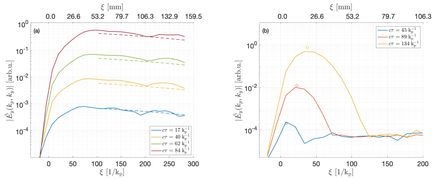
Fig. 5.4: 2D PIC simulations of the OTSI induced by a step-like e^-e^+ pair beam and comparison with linear theory in the spatiotemporal regime for \gamma_{0b} = 20 . Spectral amplitude |\tilde{E}_y(k_x, k_y)| of the dominant oblique mode ( k_x = k_p , k_y \simeq 3k_p ) as a function of \xi for different propagation distances c\tau with ballistic propagation for beam particles at the beam entrance (a) and without ballistic propagation (b). Dashed lines in (a) plot the theoretical temporal growth of |\tilde{E}_y(k_p, 3k_p)| at different times c\tau \geq 17k_p^{-1} . Circles in (b) display the temporal growth of the initial (blue) circle propagating at c/3 . Figure (a) from Ref. [111].
