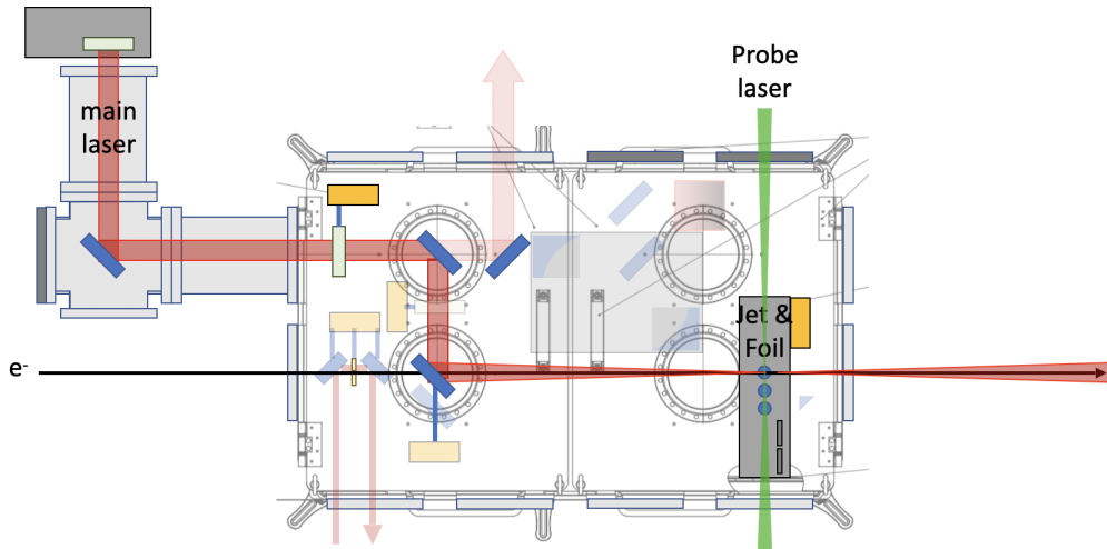
Fig. 6.1: Schematic overview of the E305 experimental set-up. The electron beam goes from left to right, main laser comes from the top left, and probe laser from the bottom right. Blue rectangles are mirrors and light green rectangle is a focusing optic.
