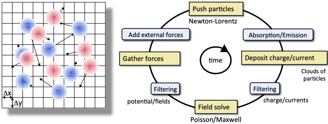
Fig. A.1: Left: schematic representation of a two-dimensional PIC cell together with the Macro-Particles represented by red and blue circles and their velocities, represented by the arrows. Right: schematic representation of a PIC loop. The main steps of the loop are displayed in the yellow squares, and additional steps are displayed in blue squares. Figure from Ref. [144].
