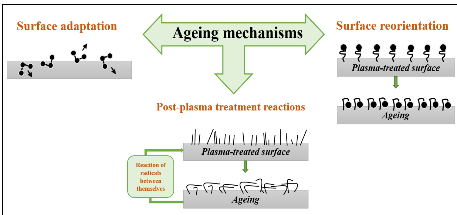
Figure 5 Ageing mechanisms
