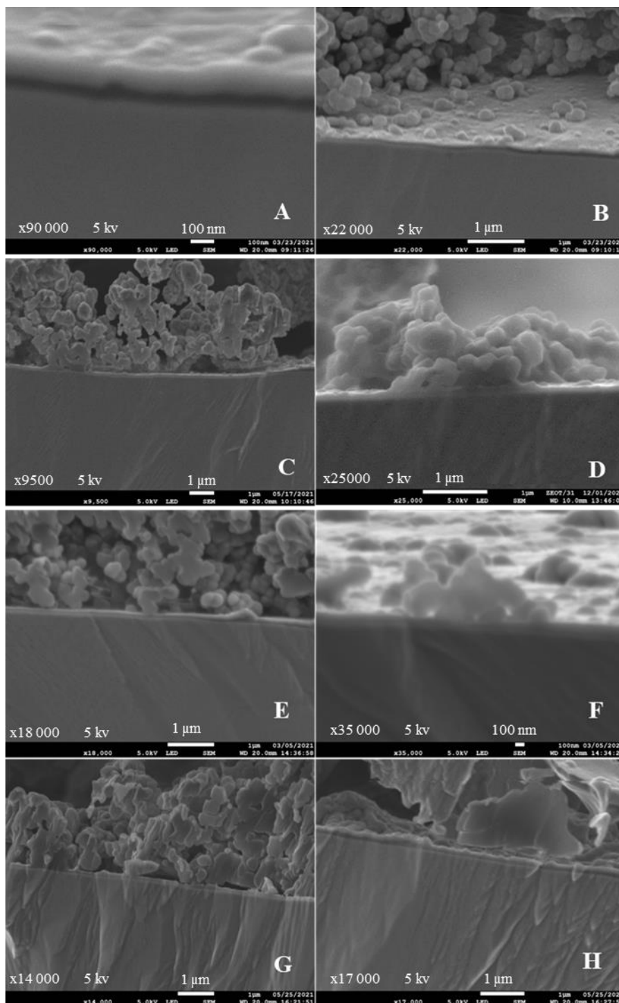
Fig. 10. SEM micrographs of cross section of coated surfaces after ion beam polishing. SD (A-B), SDGN (C-D), SDAN (E-F), SDN (G-H).
