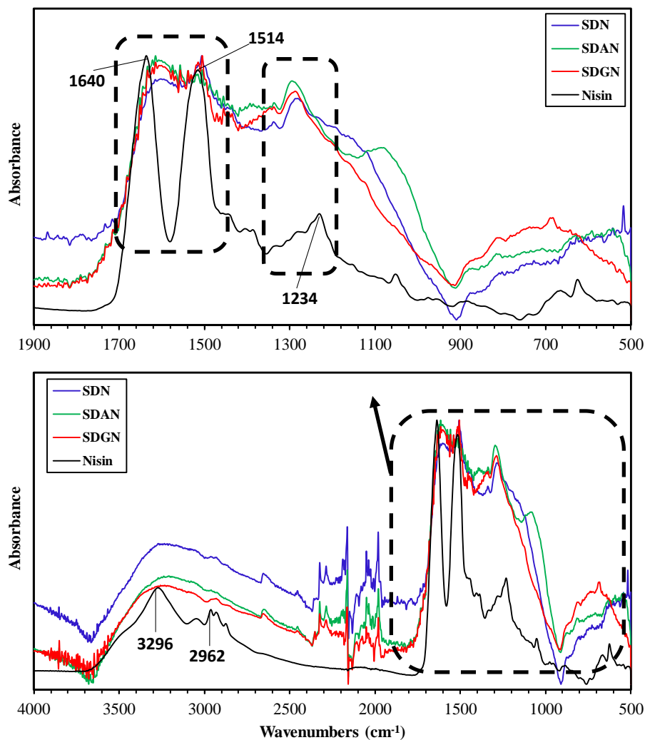
Fig. 11. FTIR spectra of different Nisin based coated SS surfaces.
