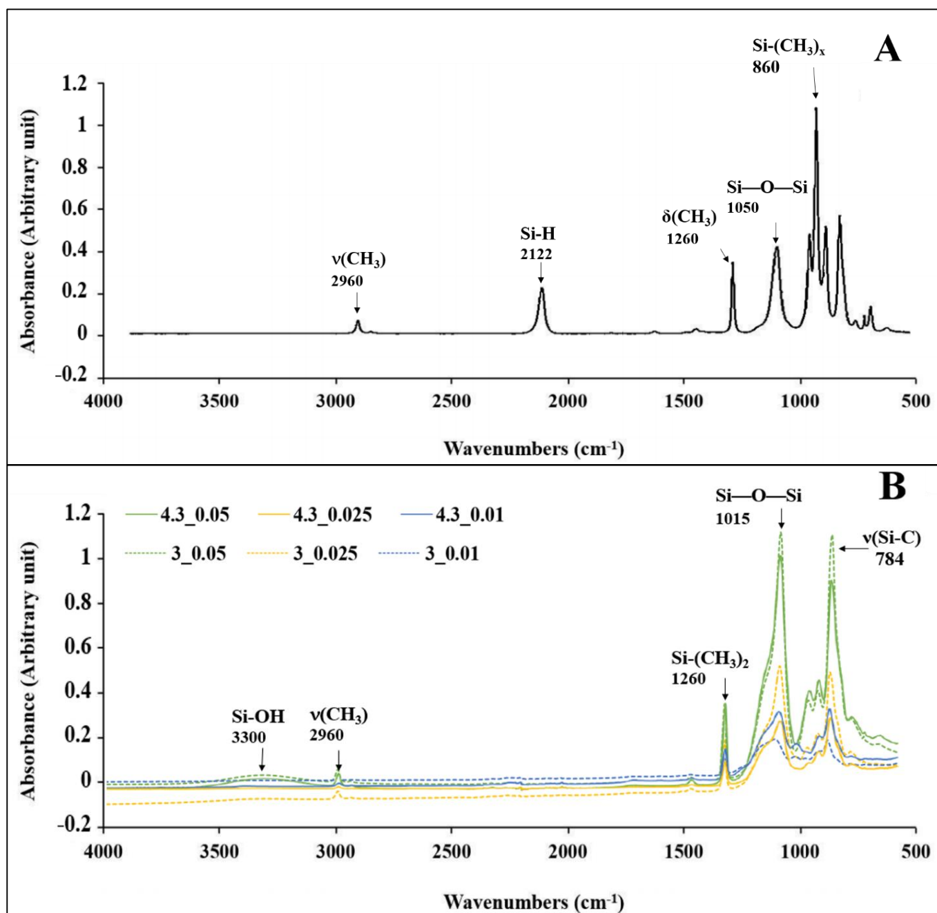
Figure 2. (A) FTIR Spectrum of TMDS monomer as a control. (B) FTIR Spectrum of TMDS coated surfaces; N 2 flow rate = 4.3 and 3 slpm varying O 2 flow rate from 0.01 to 0.025 to 0.05 slpm.
