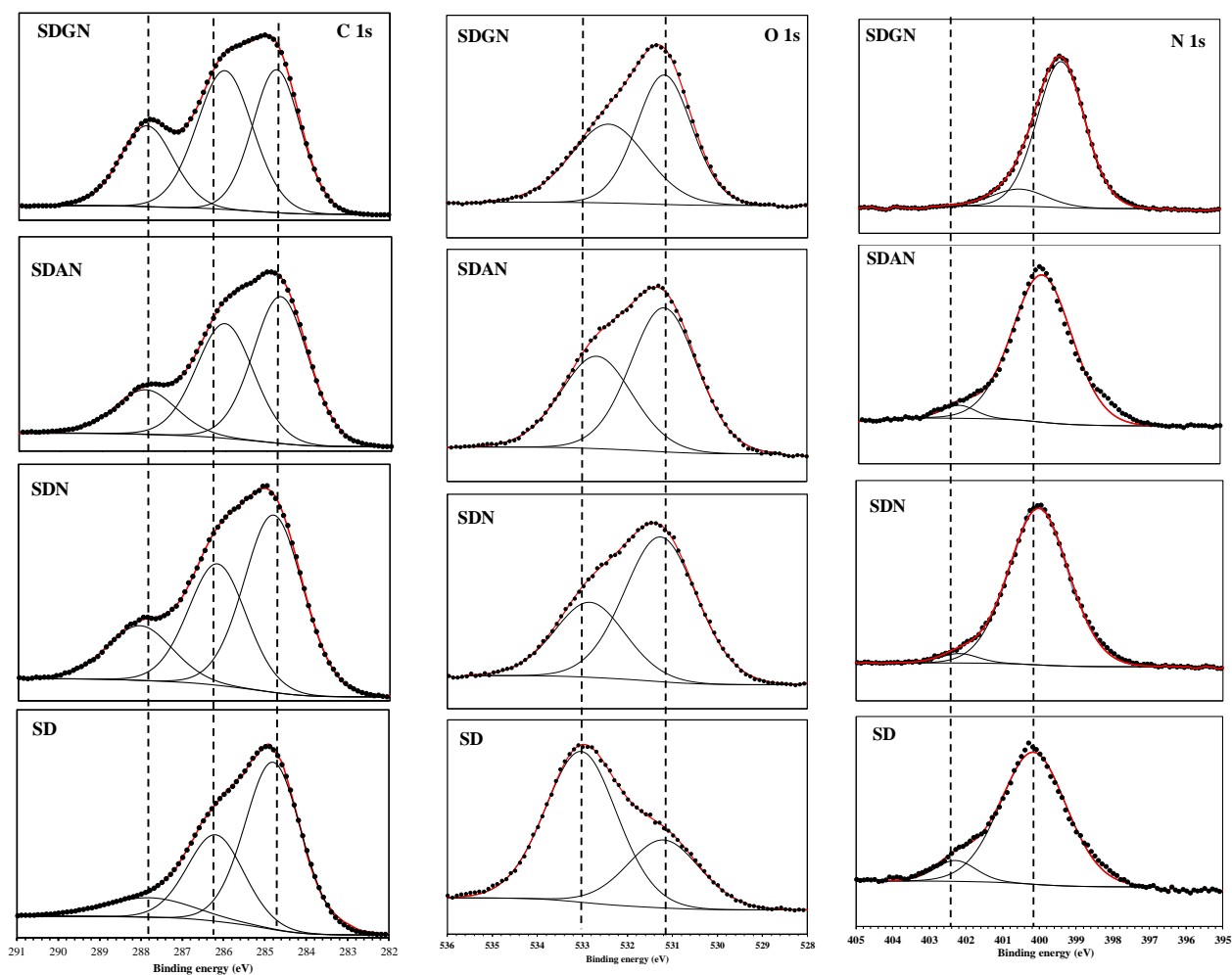
Fig. 13. High-resolution X-ray photoelectron deconvoluted profiles of C 1s, O 1s and N 1s for different coated SS surfaces.
