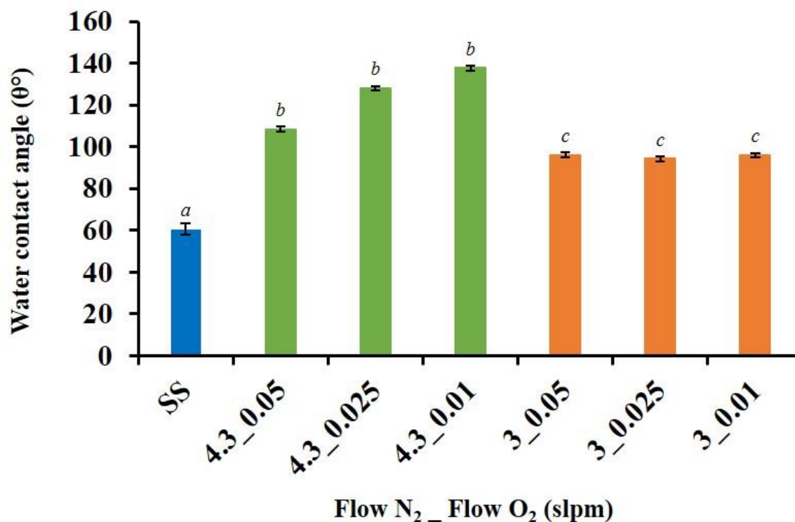
Figure 3. Water contact angle measurements for uncoated and coated SS; (Blue) uncoated SS; (Green) TMDS coatings with N 2 flow rate = 4.3 slpm varying O 2 flow rate from 0.05 to 0.025 to 0.01 slpm (Orange) TMDS coatings with N 2 flow rate = 3 slpm varying O 2 flow rate from 0.05 to 0.025 to 0.01 slpm. (*) each represented value is a mean of 6 measures for each type of coupon. Different letters on error bars (a, b, and c) indicate significant differences ( P < 0.05 ); same letters on error bars indicate non-significant differences ( P > 0.05 ).
