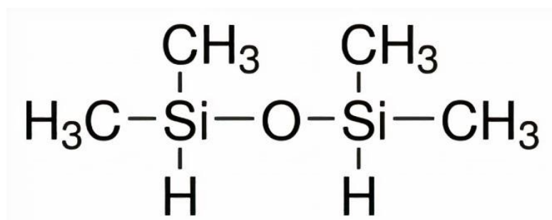
Figure 1. Chemical structure of 1,1,3,3-Tetramethyldisiloxane
