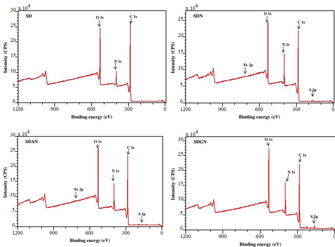
Fig. 12. XPS survey spectra of different coated SS surfaces.
