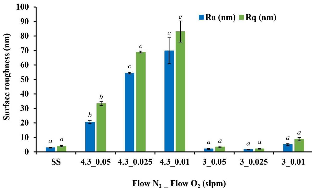
Figure 6. Surface roughness variation of bare SS and TMDS-based coatings. (Blue) representing the Ra (nm) and (Green) representing the Rq (nm). (*) each represented value is a mean of 6 measures for each type of coupon. Different letters on error bars (a, b, and c) indicate significant differences ( P < 0.05 ); same letters on error bars indicate non-significant differences ( P > 0.05 ).
