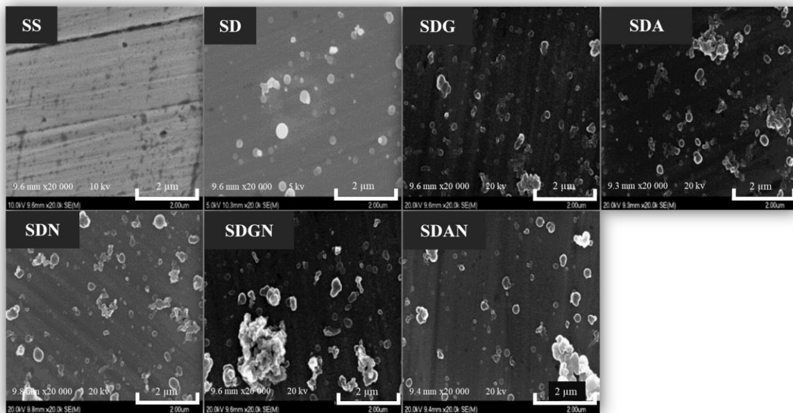
Fig. 9. Scanning electron microscopy micrographs of bare SS coated surfaces.
