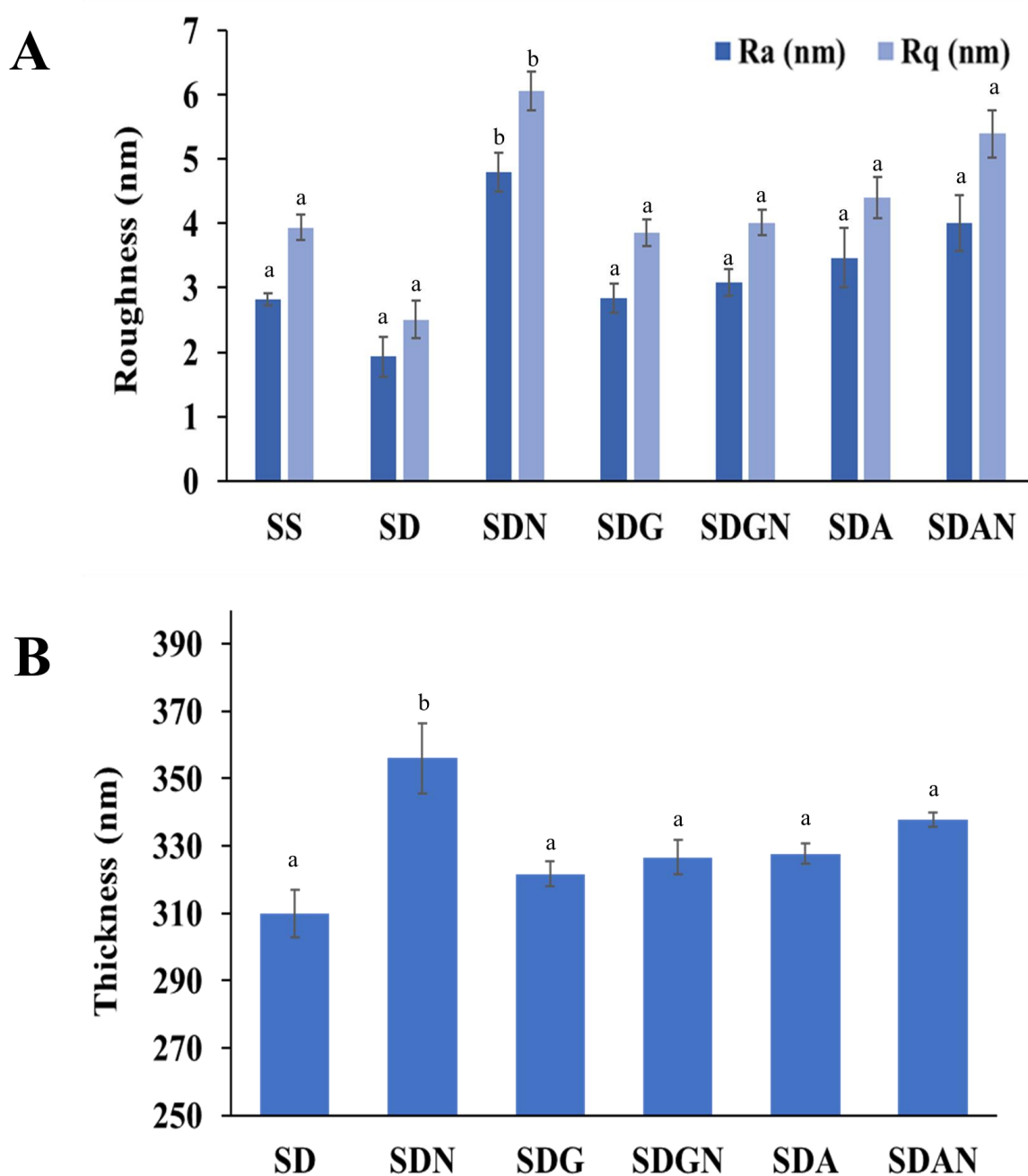
Fig. 8. (A) Surface roughness parameters R_a and R_q for bare SS and coated SS surfaces. (B) Thickness of treated surfaces defined by averaged values in \text{nm} \pm \text{SD} . (*) Different letters on top of error bars (a, b) indicate significant differences ( p < 0.05 ); the same letters on error bars indicate non-significant differences ( p > 0.05 ).
