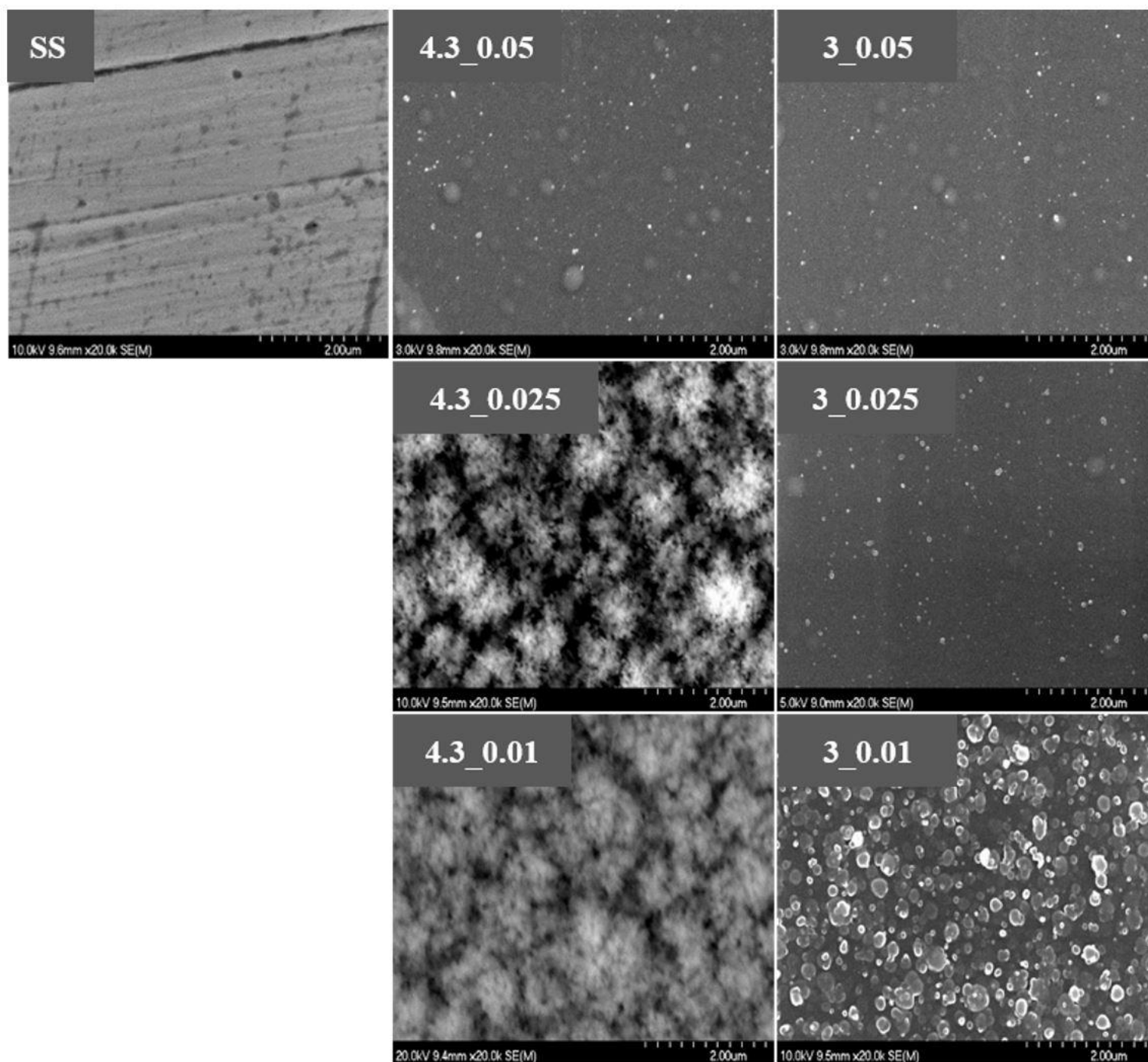
Figure 7. Scanning electron microscopy (SEM) micrographs; (SS) Micrograph of uncoated SS; (4.3_0.05, 4.3_0.025; 4.3_0.01) Micrographs of TMDS coatings with N 2 flow rate = 4.3 slpm varying O 2 flow rate from 0.05 to 0.025 to 0.01 slpm; (3_0.05, 3_0.025; 3_0.01) Micrographs TMDS coatings with N 2 flow rate = 3 slpm varying O 2 flow rate from 0.05 to 0.025 to 0.01 slpm
