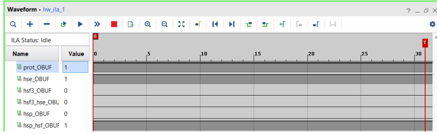
(a) Hardware debug of \mathcal{R}_{hsr1} model.
