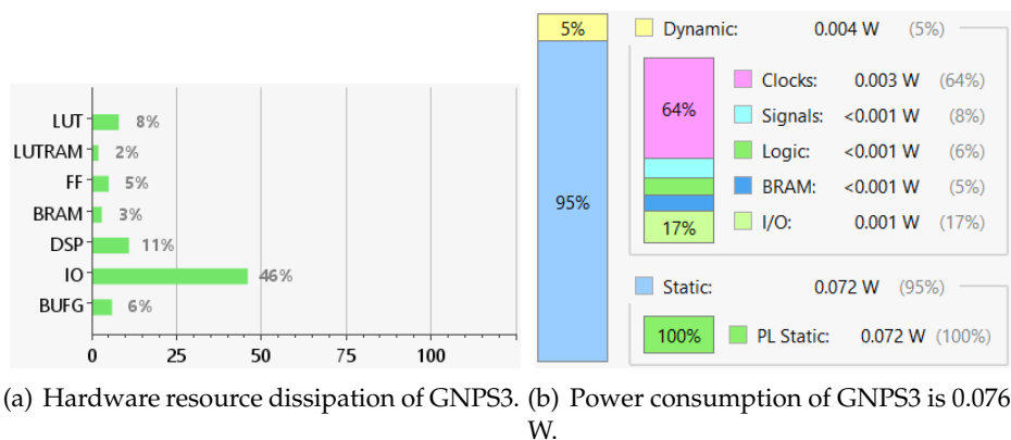
FIGURE B.9: Hardware resource dissipation and power consumption of hardened GNPS3.
