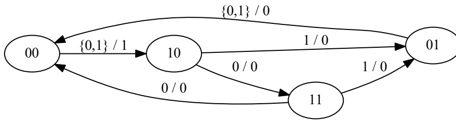
FIGURE 4.1: The Mealy automaton for the circuit described by Equation (4.2). The label of the state corresponds to the value of the vector (q_1, q_2) . The label of the transition corresponds to the value of the input variable x and output y .
