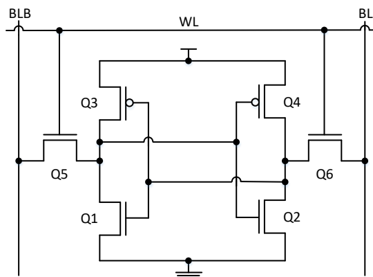
FIGURE 3.3: A 6T CMOS SRAM cell [115].
