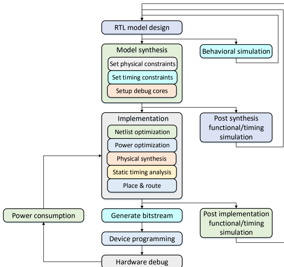
FIGURE 3.6: Vivado FPGA development flow.
